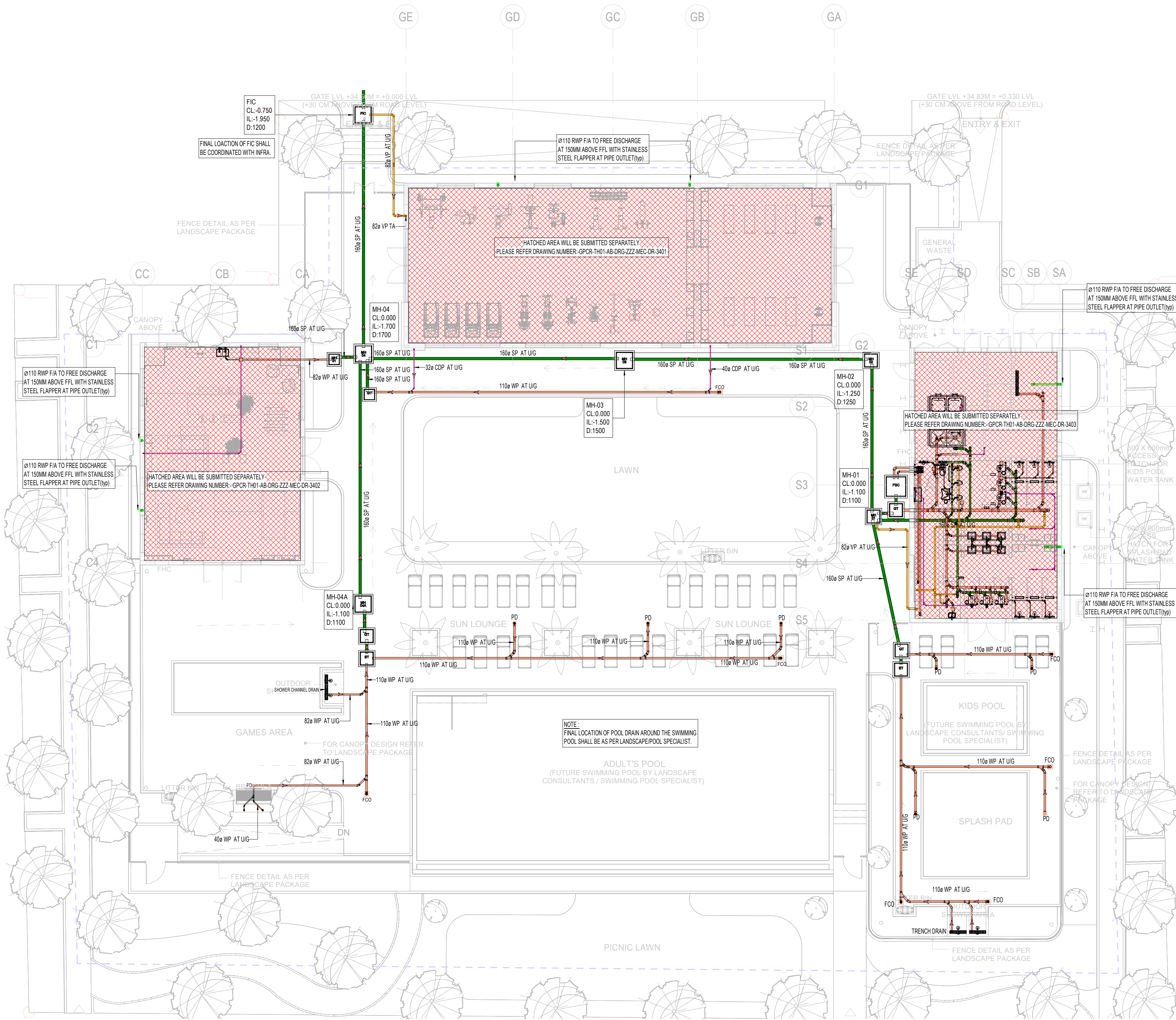
1 OVERALL GROUND FLOOR DRAINAGE LAYOUT 1 : 150
