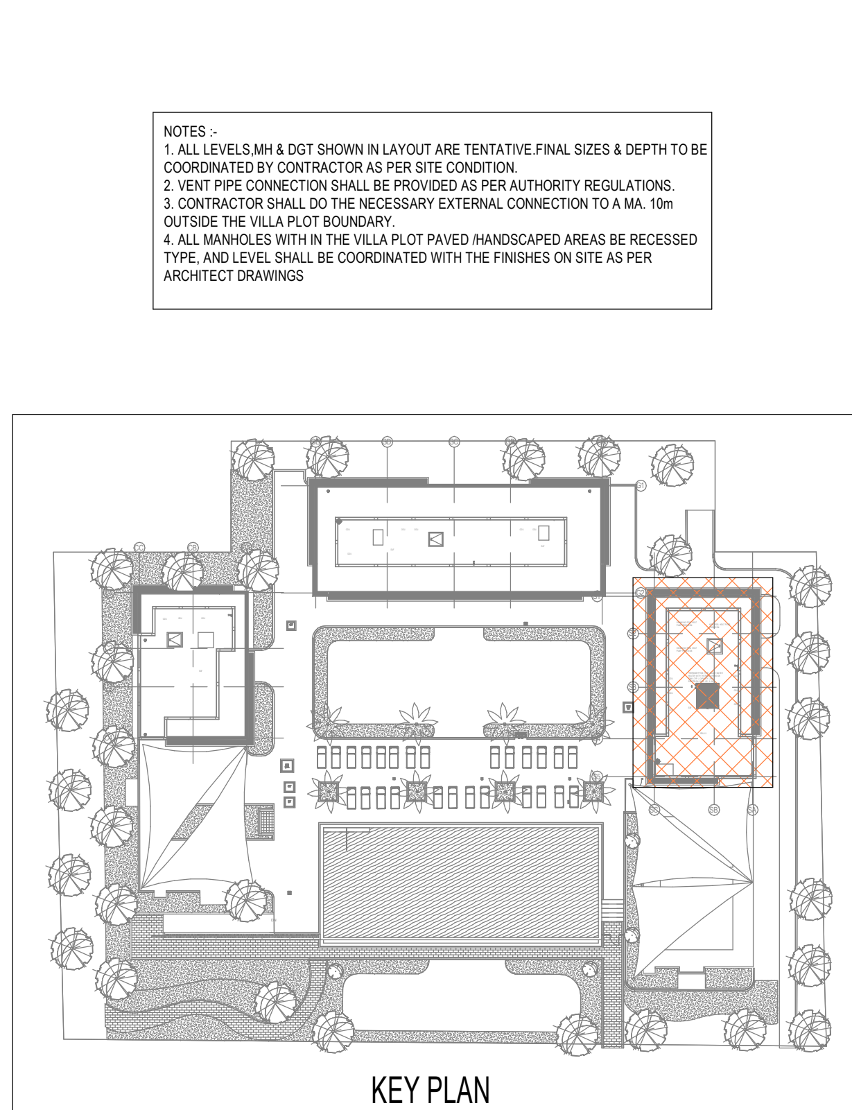
KEY PLAN
