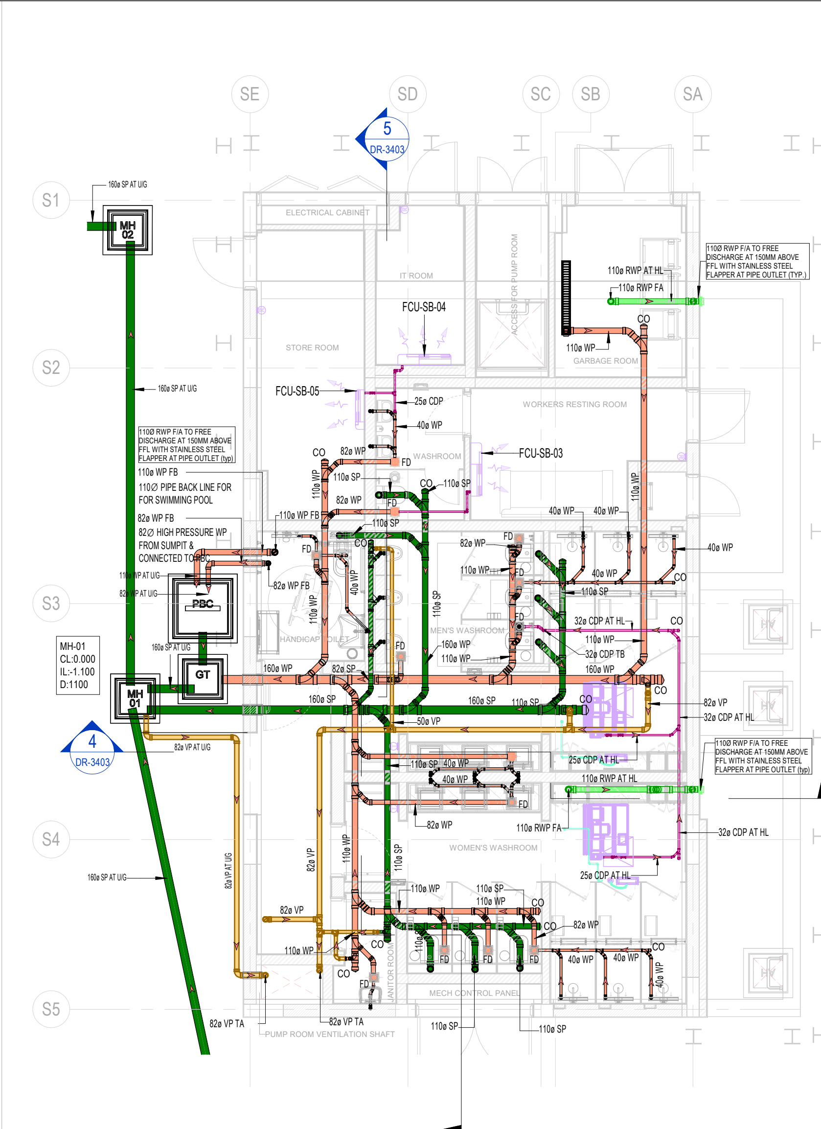
2 GROUND FLOOR DRAINAGE LAYOUT SERVICE BLOCK 1 : 75
