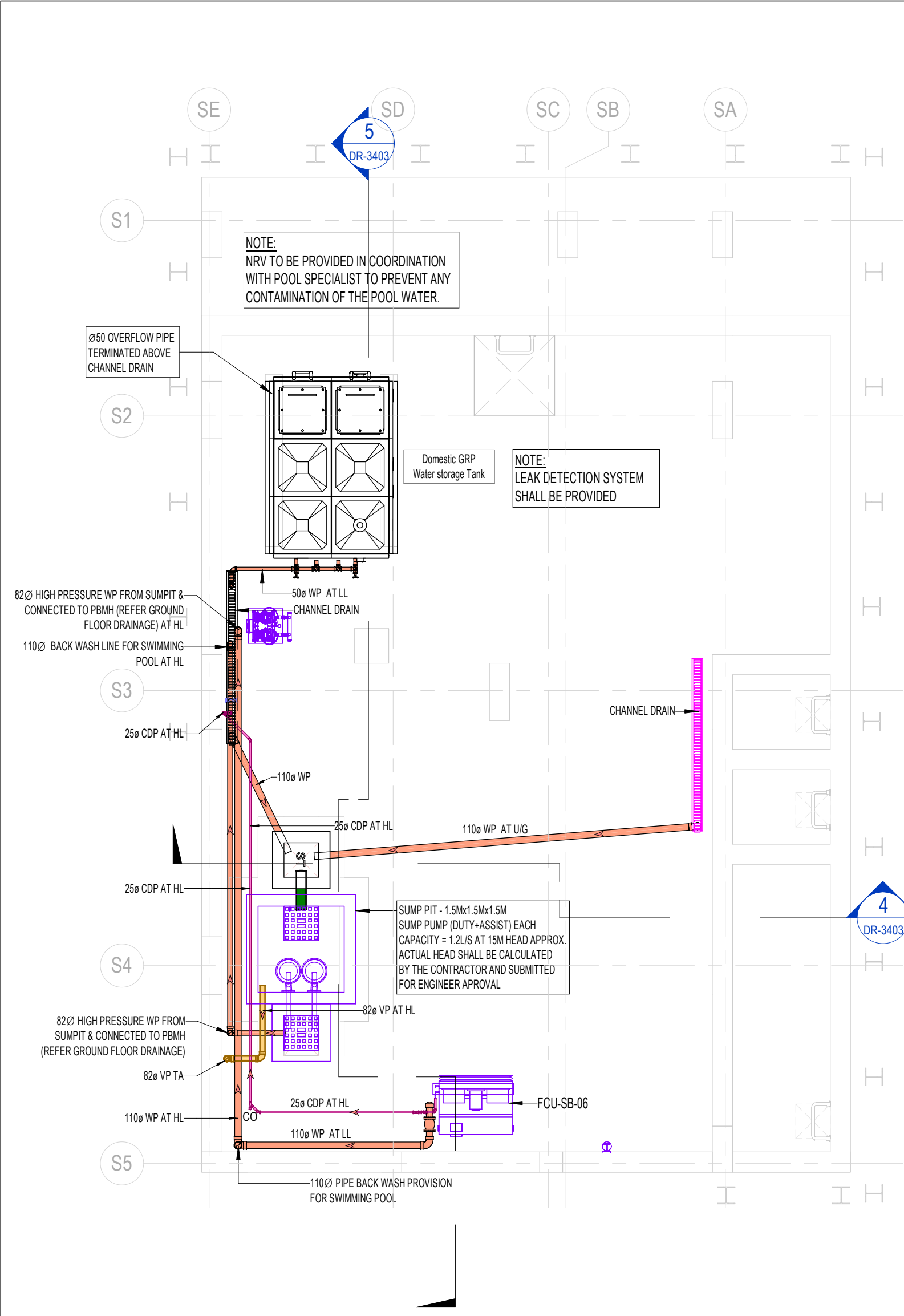
1 BASEMENT FLOOR DRAINAGE LAYOUT SERVICE BLOCK 1 : 75
