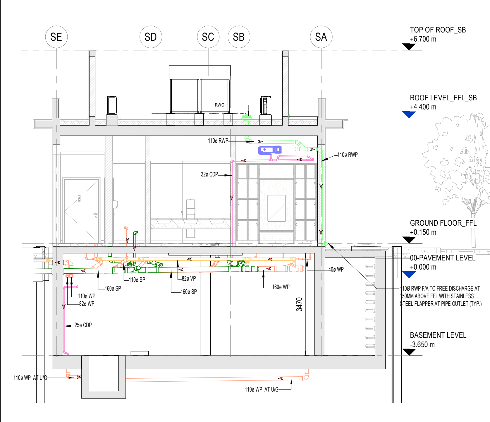
4 SERVICE BLOCK DRAINAGE SECTION 01 1 : 75
