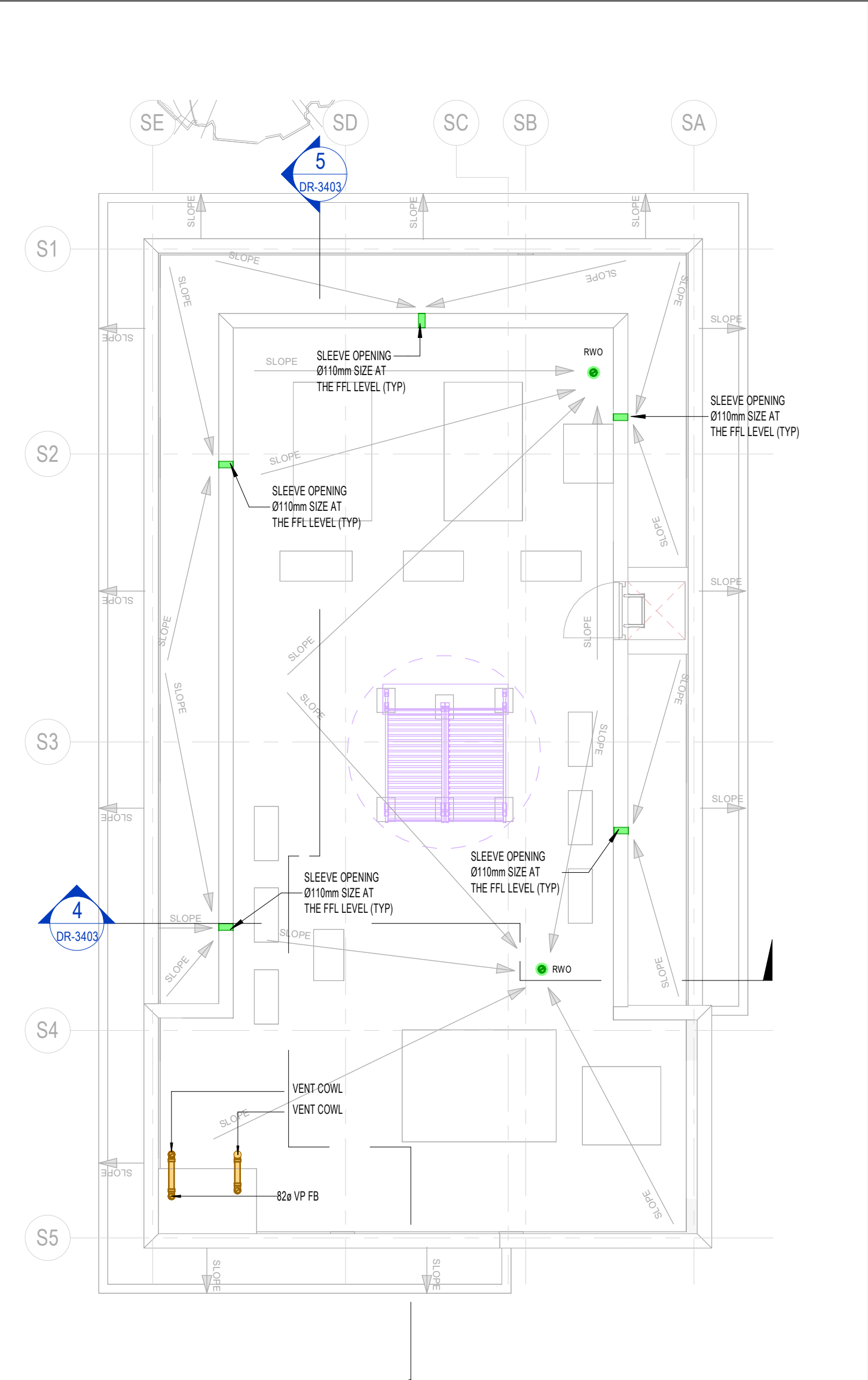
3 ROOF FLOOR DRAINAGE LAYOUT SERVICE BLOCK 1 : 75
