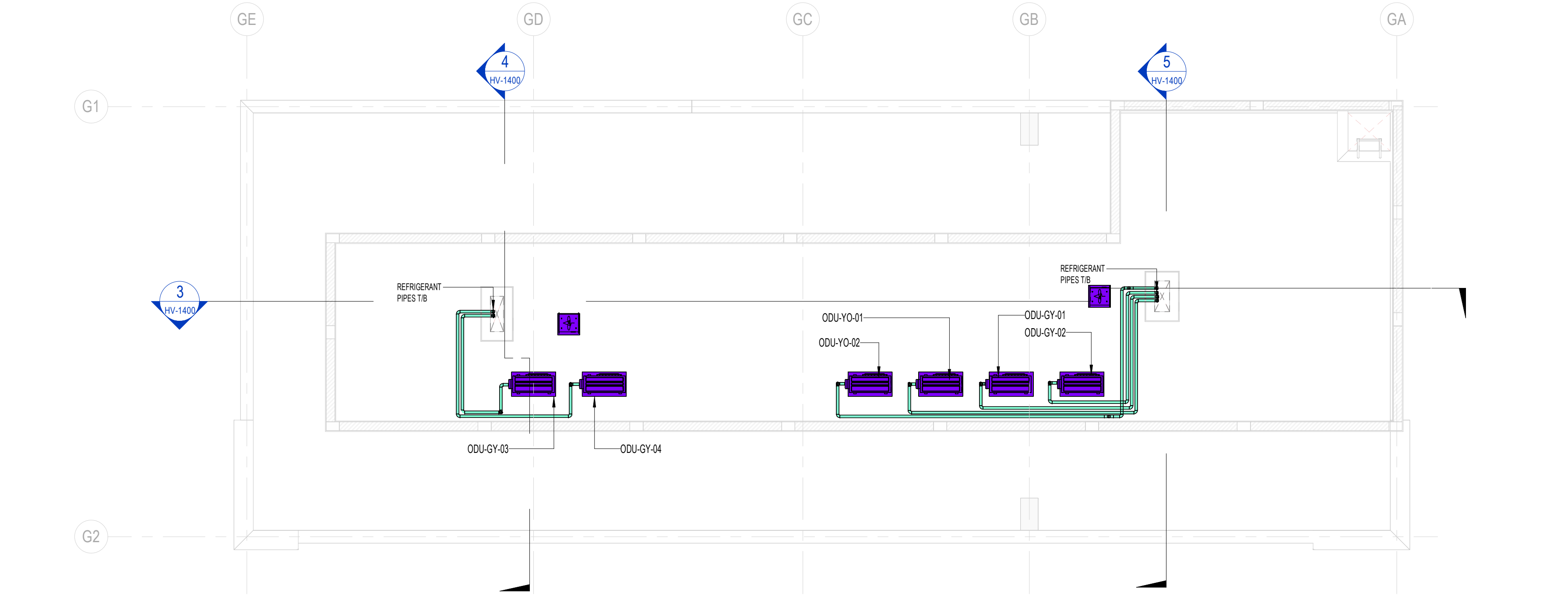
2 ROOF FLOOR HVAC LAYOUT-GYM&YOGA 1 : 75
