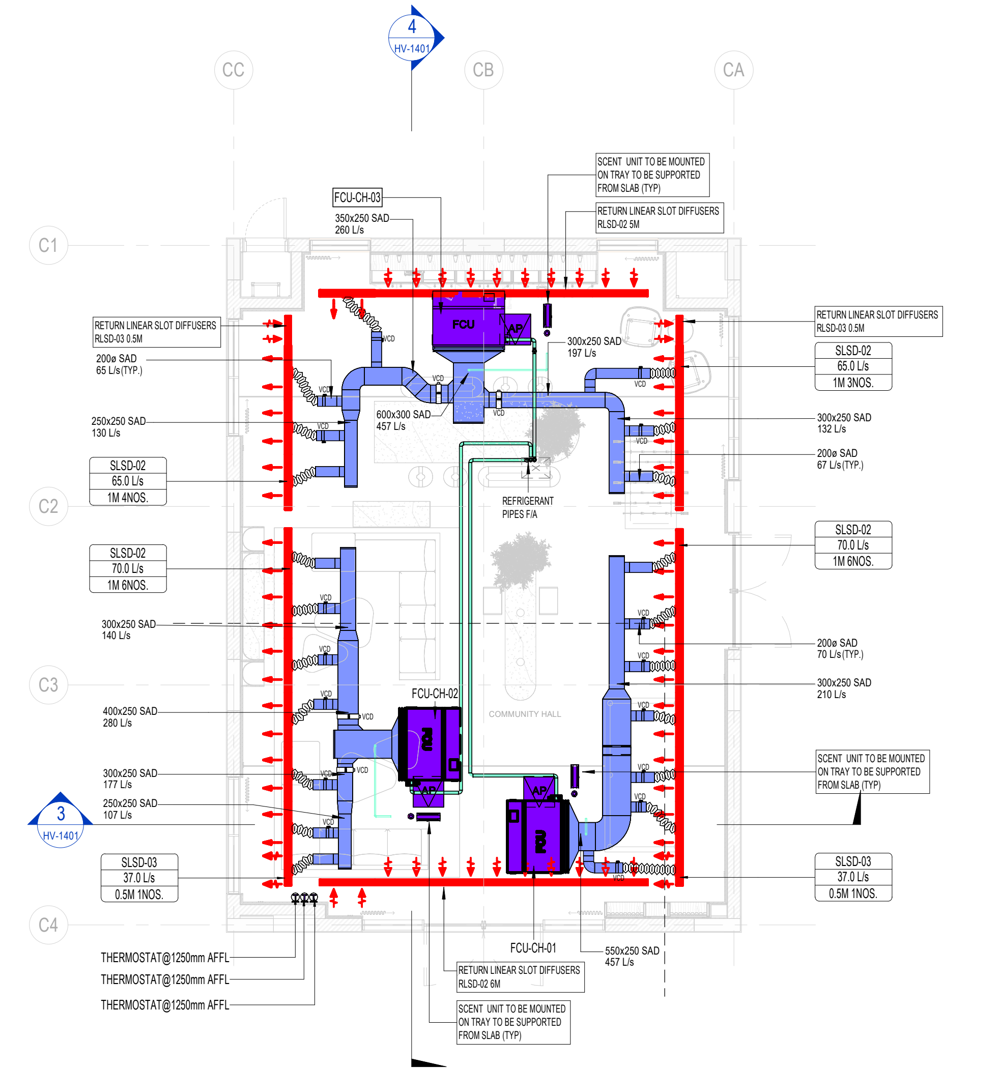
1 GROUND FLOOR HVAC LAYOUT-COMMUNITY HALL 1 : 75
