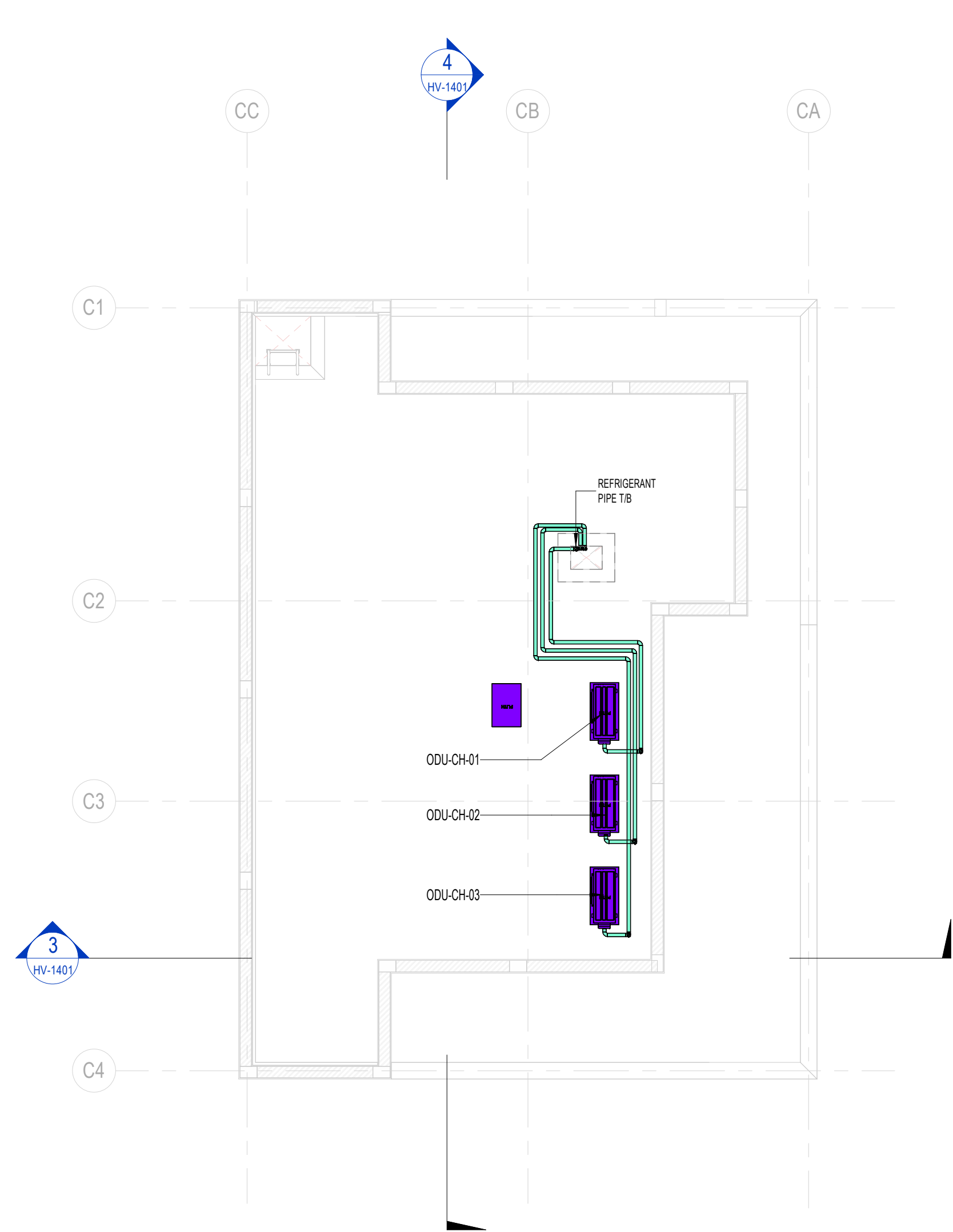
2 ROOF FLOOR HVAC LAYOUT-COMMUNITY HALL 1 : 75
