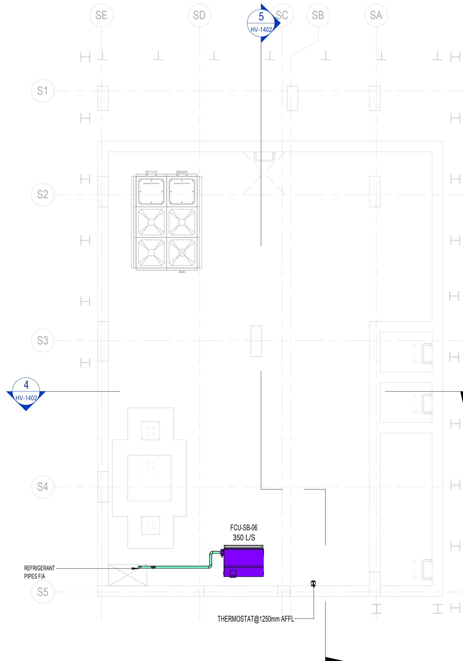
1 BASEMENT FLOOR HVAC LAYOUT 1 : 75
