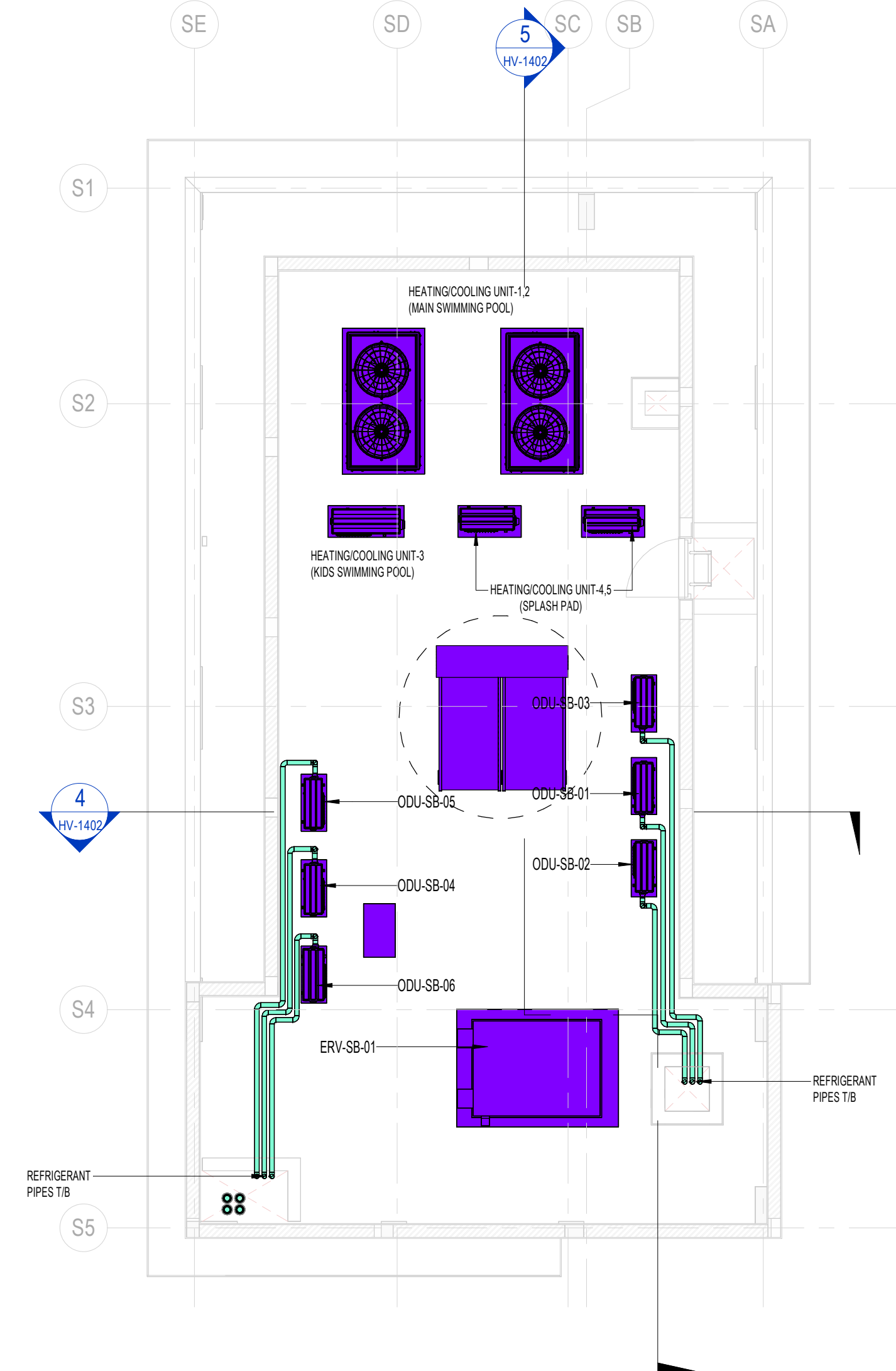
3 ROOF FLOOR HVAC LAYOUT-SERVICE BLOCK 1 : 75
