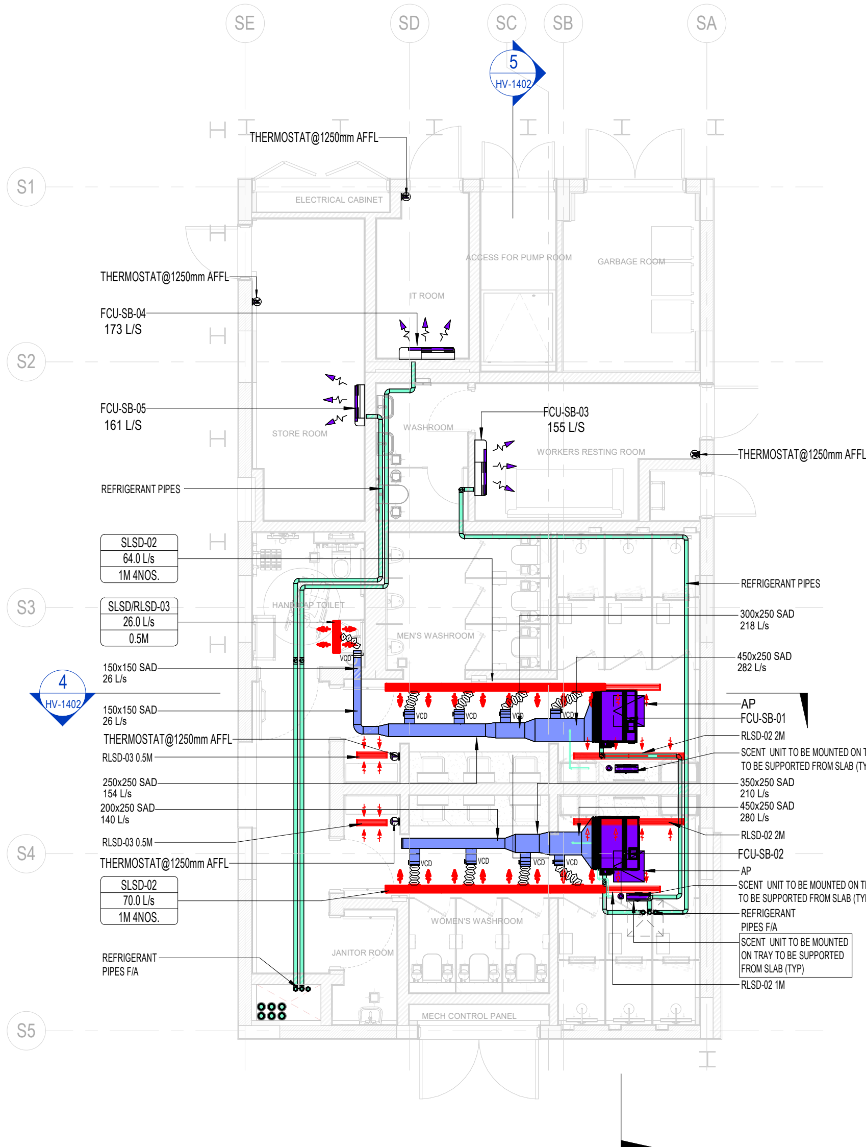
2 GROUND FLOOR HVAC LAYOUT-SERVICE BLOCK 1 : 75
