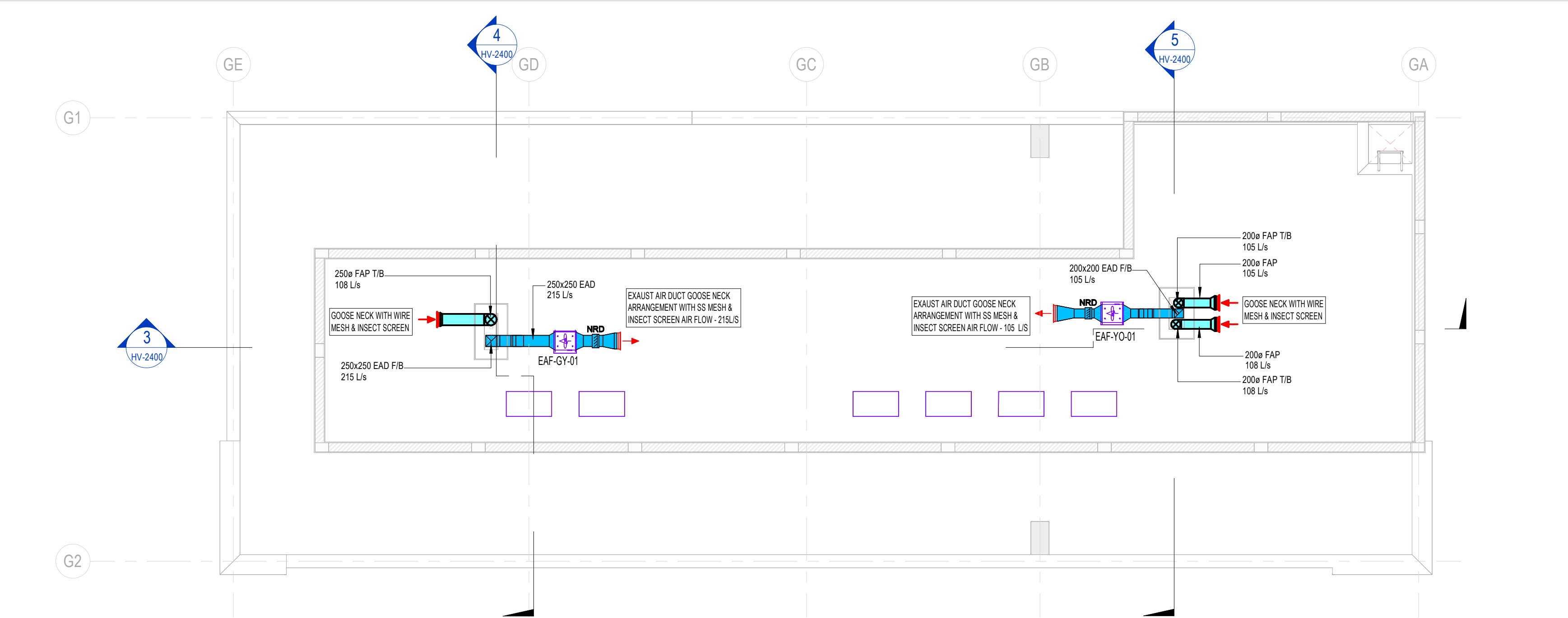
1 GROUND FLOOR VENTILATION LAYOUT-GYM&YOGA 1 : 75
