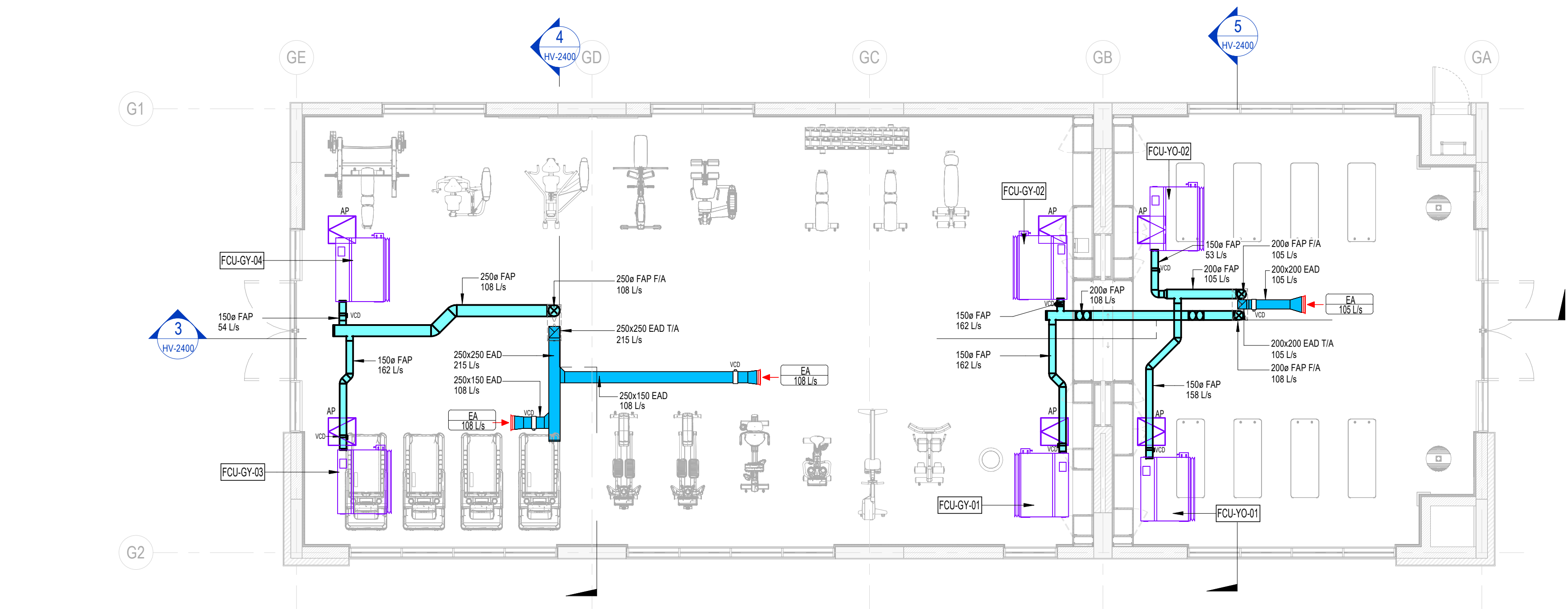
1 GROUND FLOOR VENTILATION LAYOUT-GYM&YOGA 1 : 75
