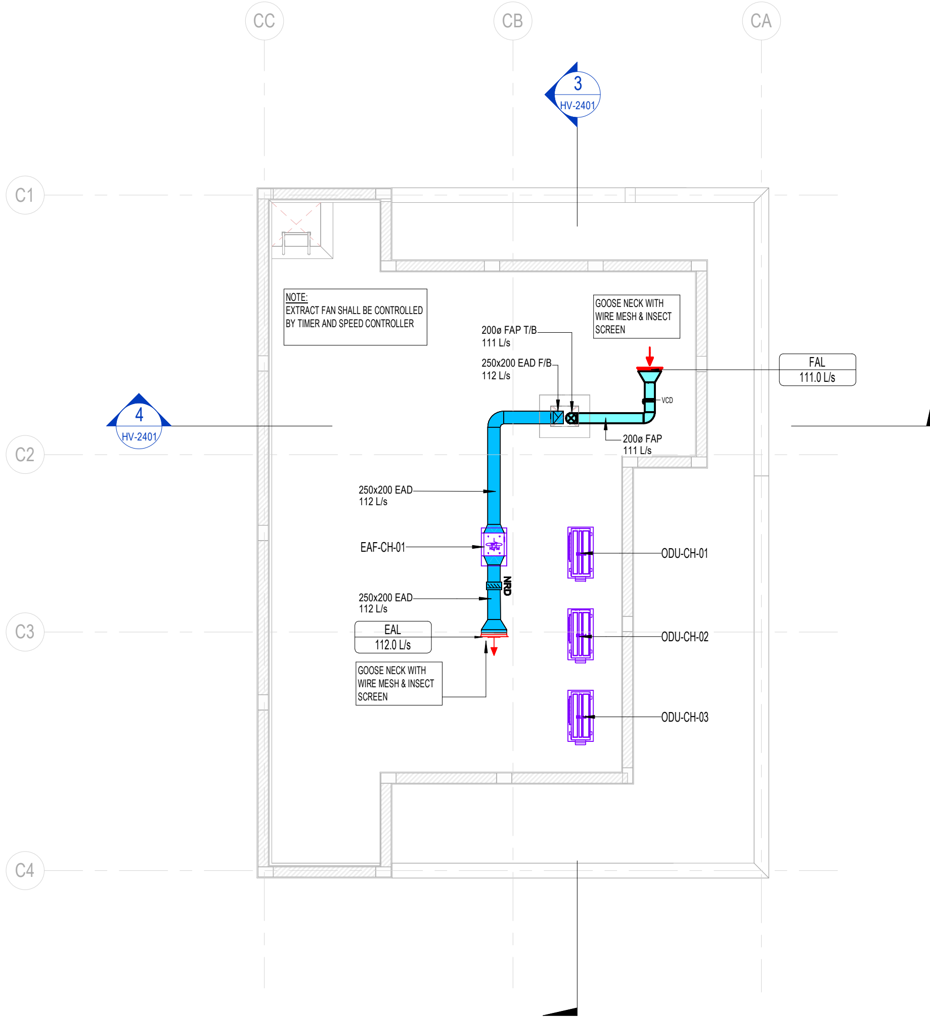
2 ROOF FLOOR VENTILATION LAYOUT-COMMUNITY HALL 1 : 75
