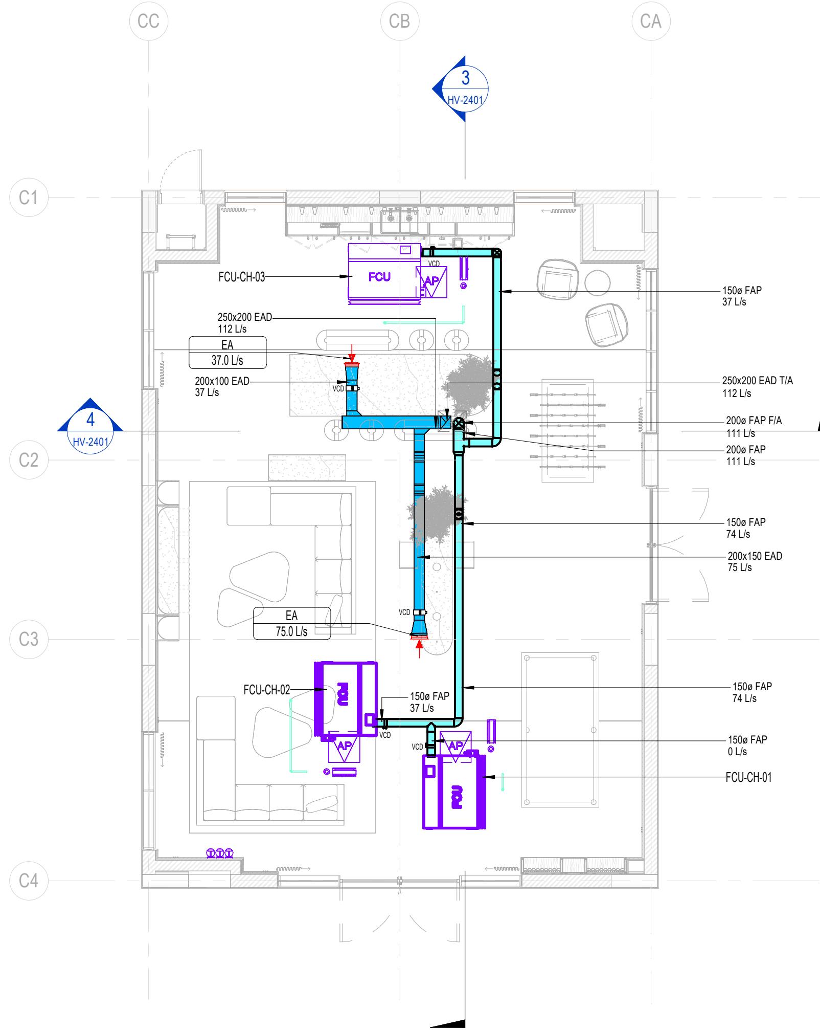
1 GROUND FLOOR VENTILATION LAYOUT-COMMUNITY HALL 1 : 75
