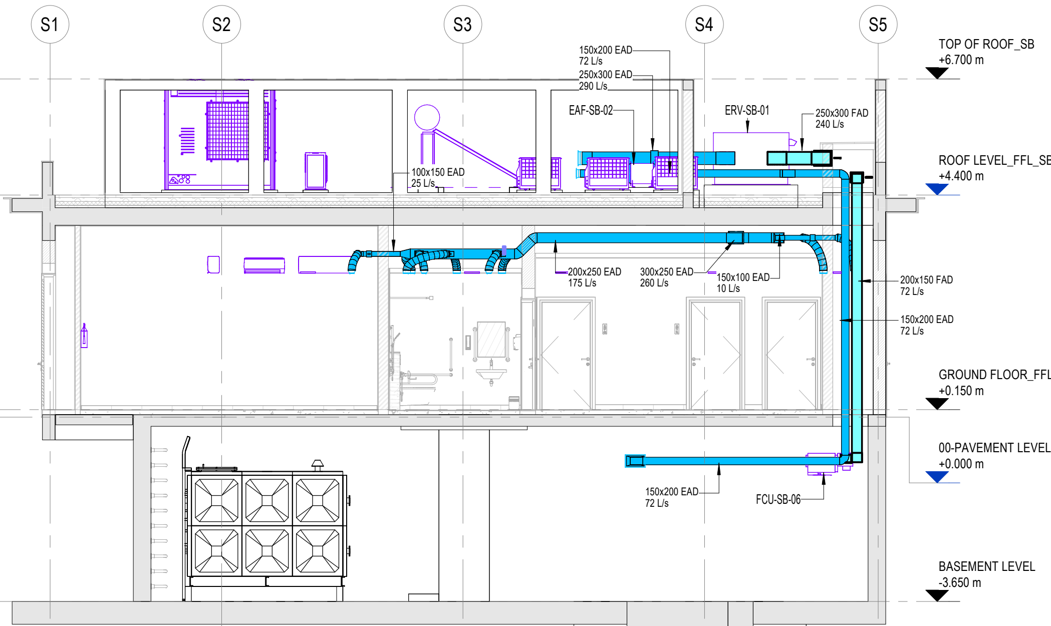
4 SERVICE BLOCK VENTILATION SECTION 01 1 : 75
