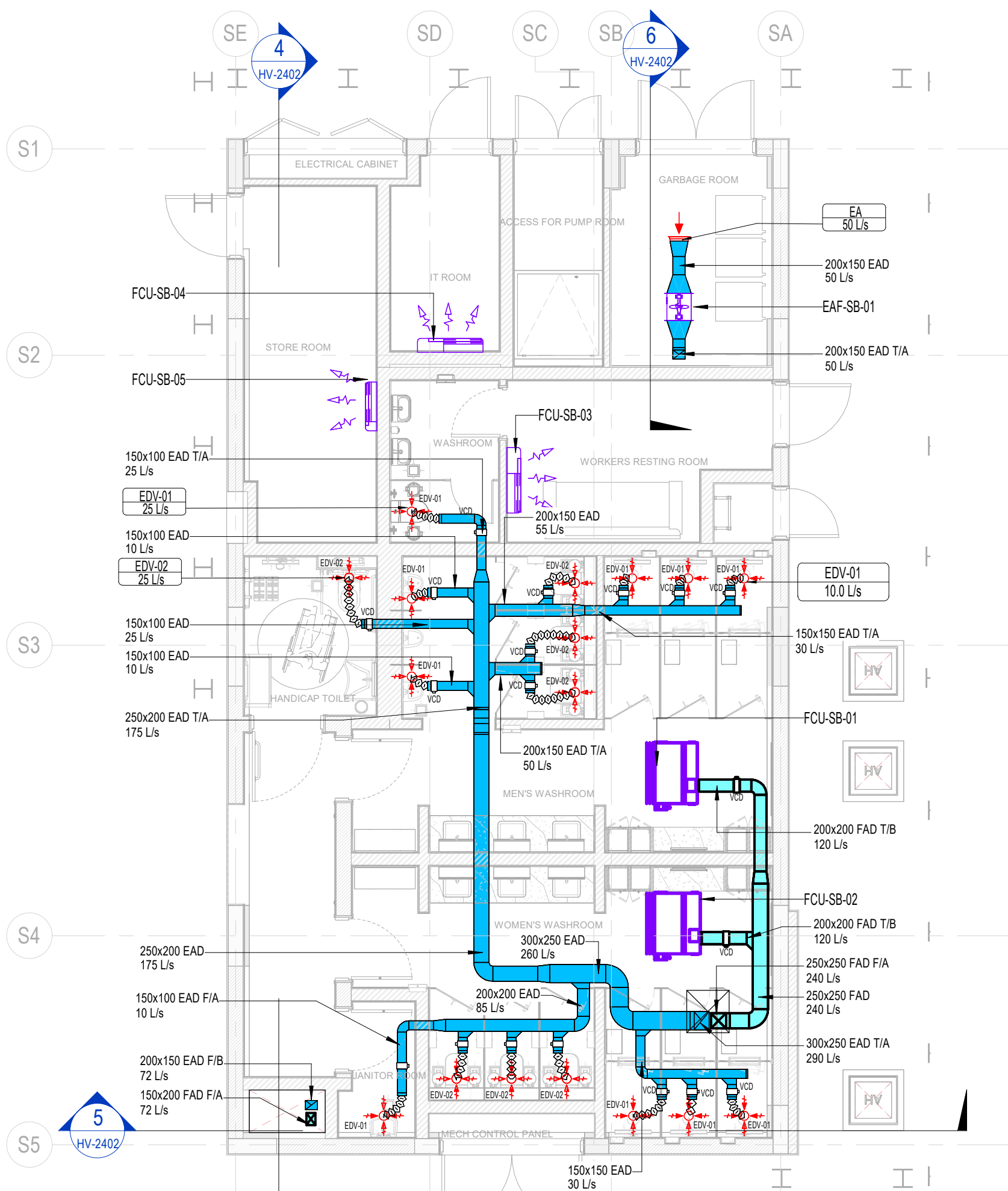
2 GROUND FLOOR VENTILATION LAYOUT-SERVICE BLOCK 1 : 75
