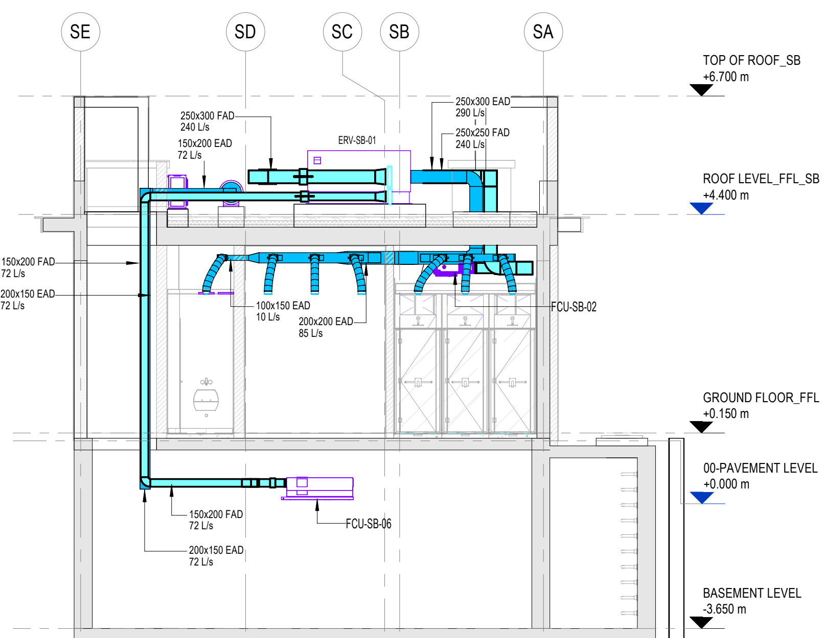
6 SERVICE BLOCK VENTILATION SECTION 03 1 : 75
