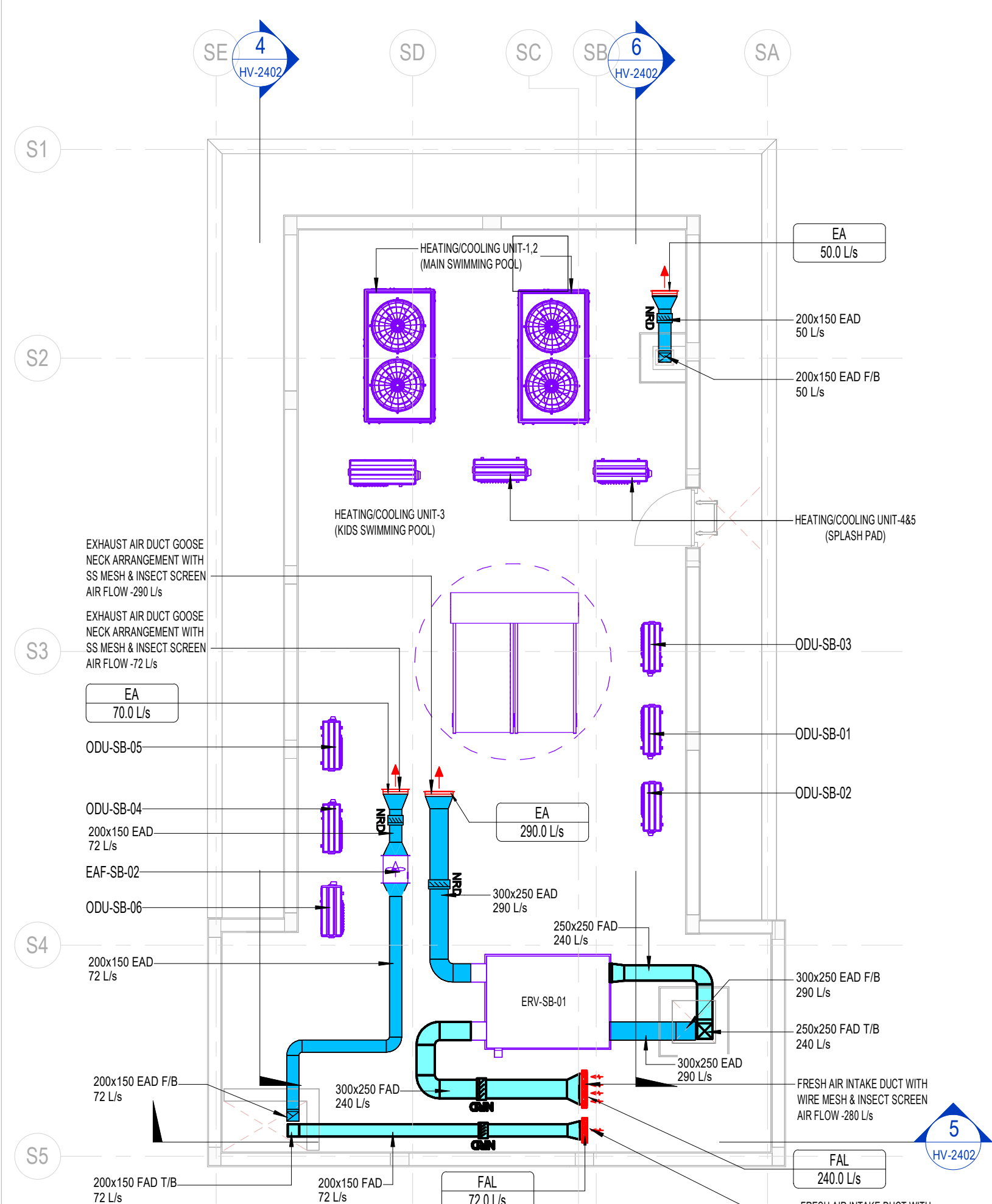
3 ROOF FLOOR VENTILATION LAYOUT-SERVICE BLOCK 1 : 75
