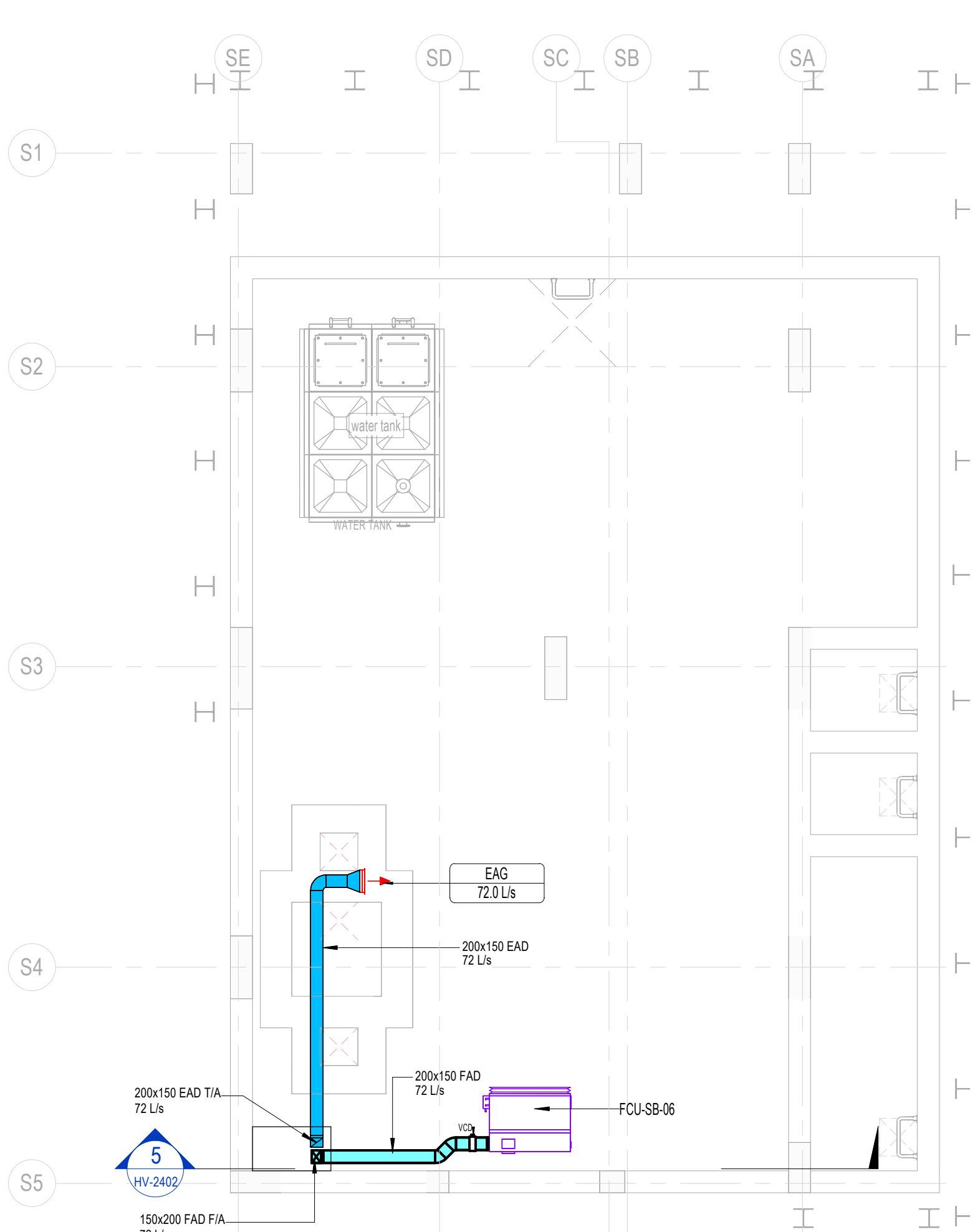
1 BASEMENT FLOOR VENTILATION LAYOUT 1 : 75
