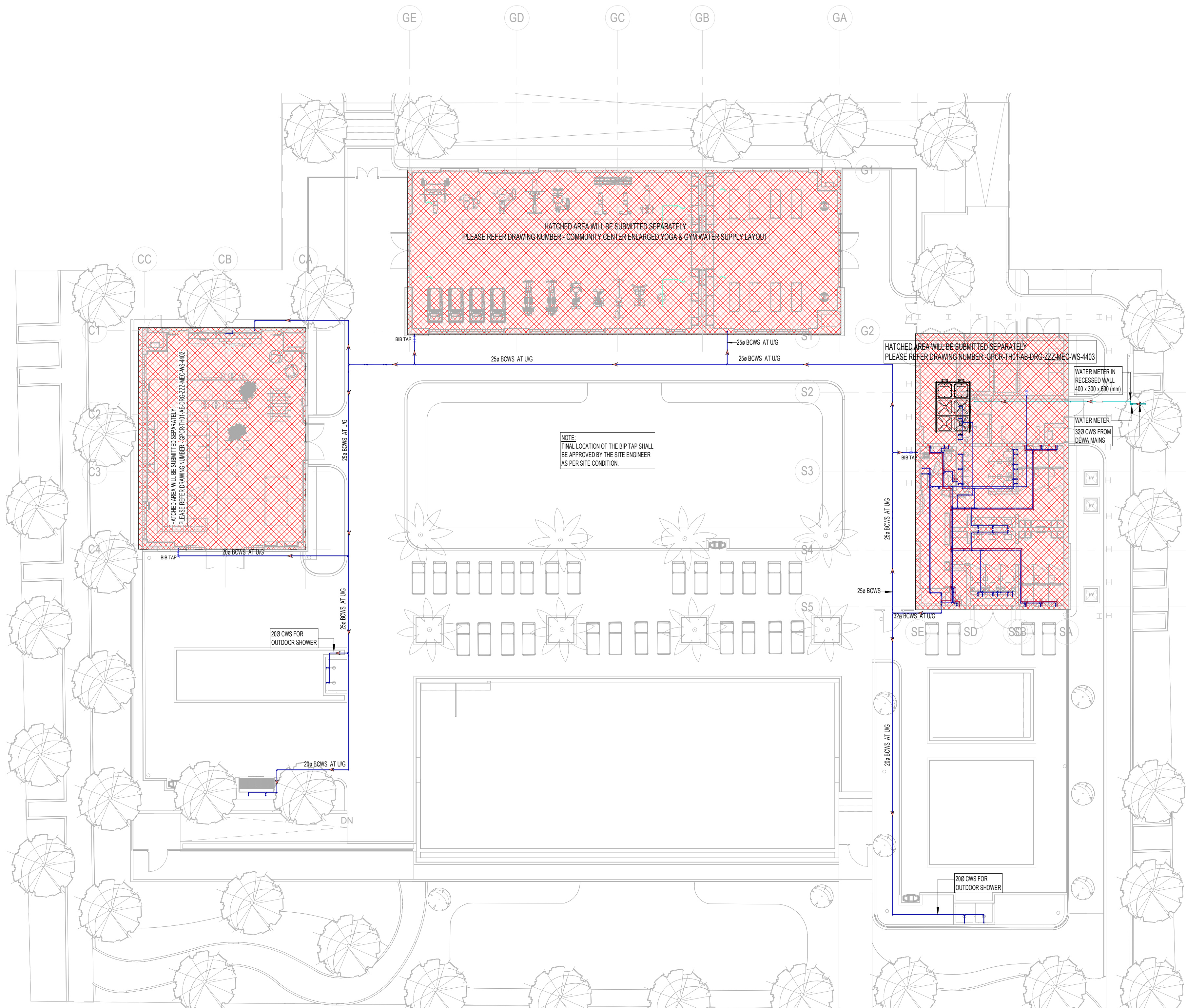
1 OVERALL GROUND FLOOR WATER SUPPLY LAYOUT 1 : 150
