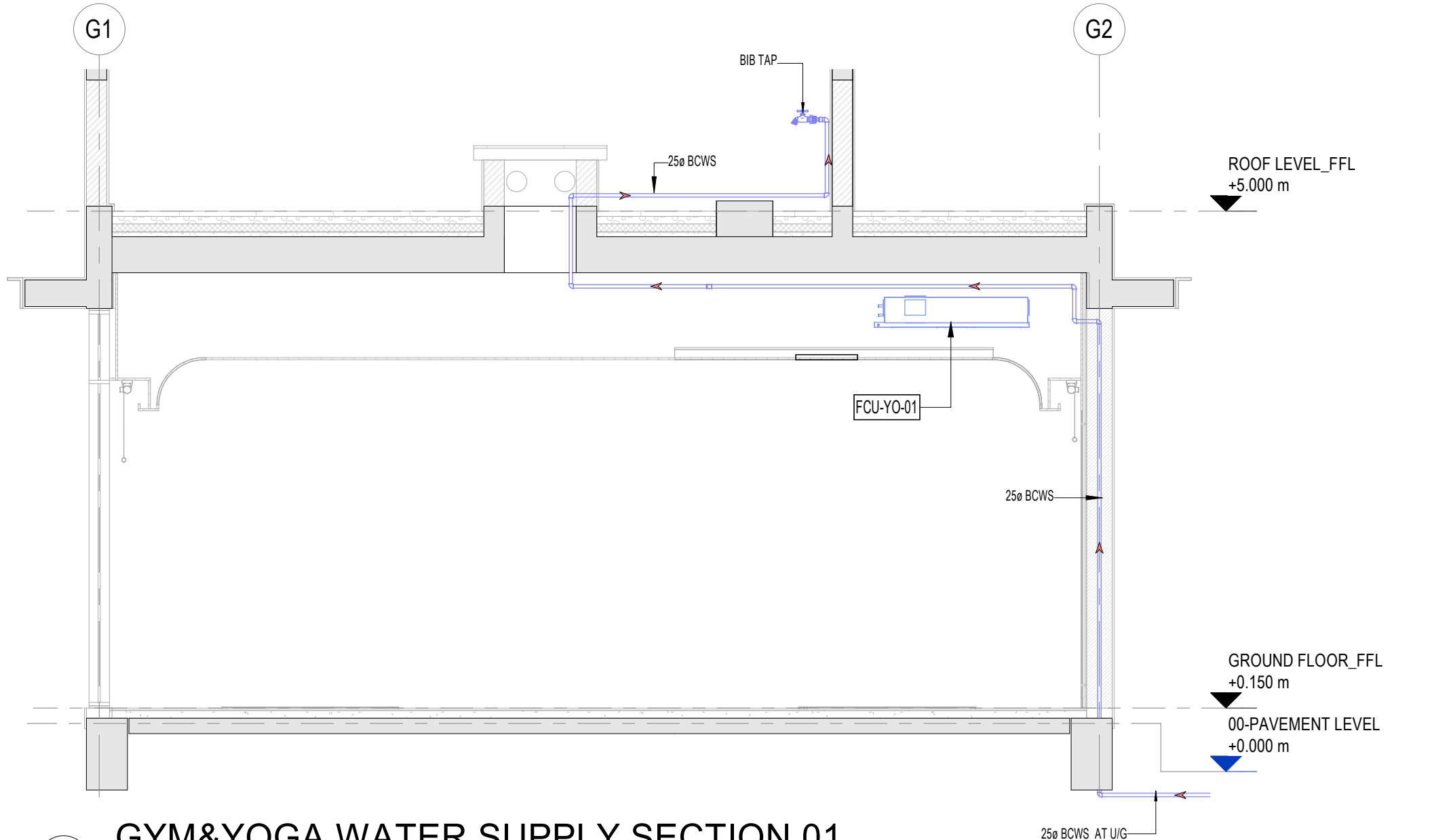
3 GYM&YOGA WATER SUPPLY SECTION 01 1 : 50
