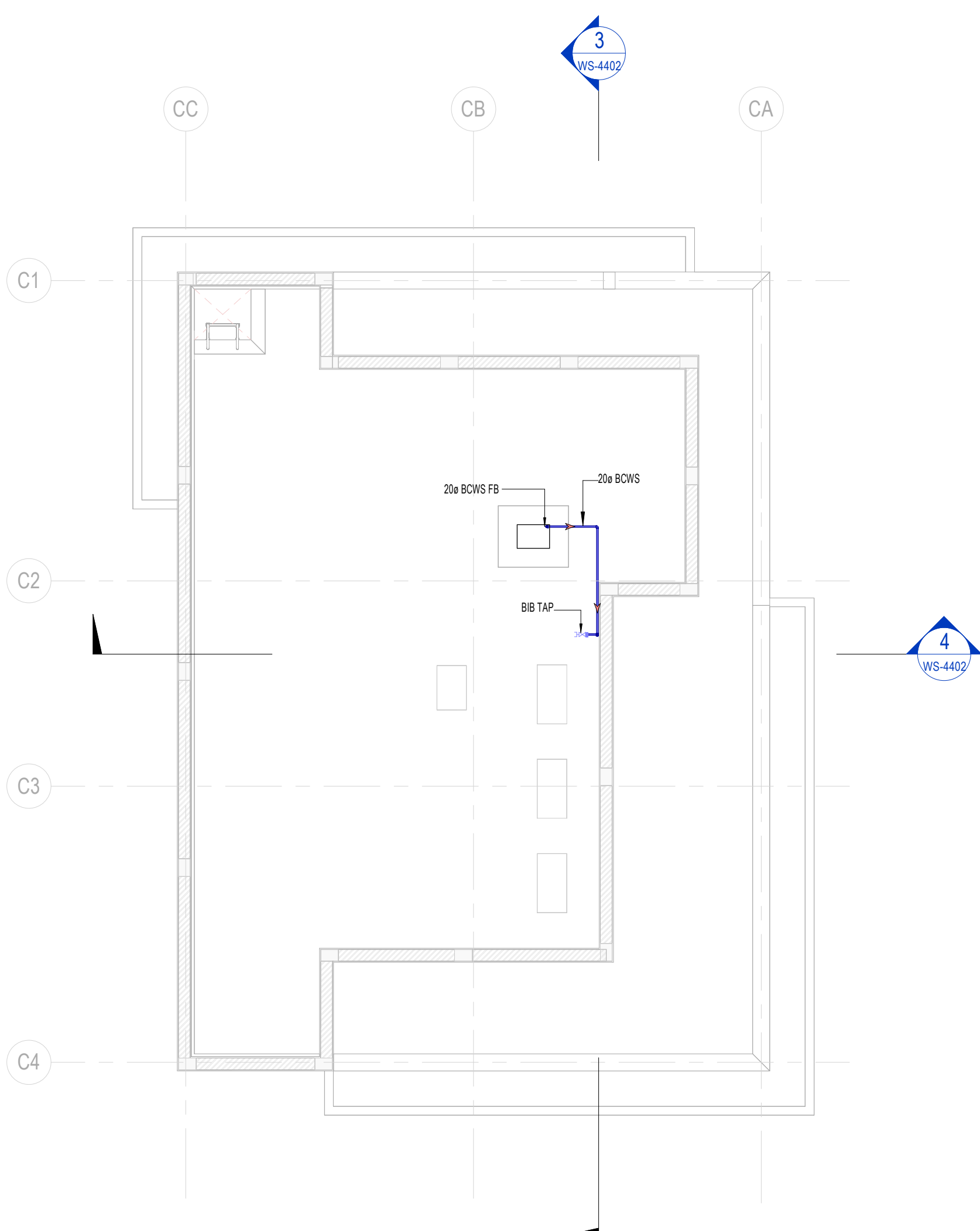
2 ROOF FLOOR WATER SUPPLY LAYOUT-COMMUNITY HALL 1 : 75
