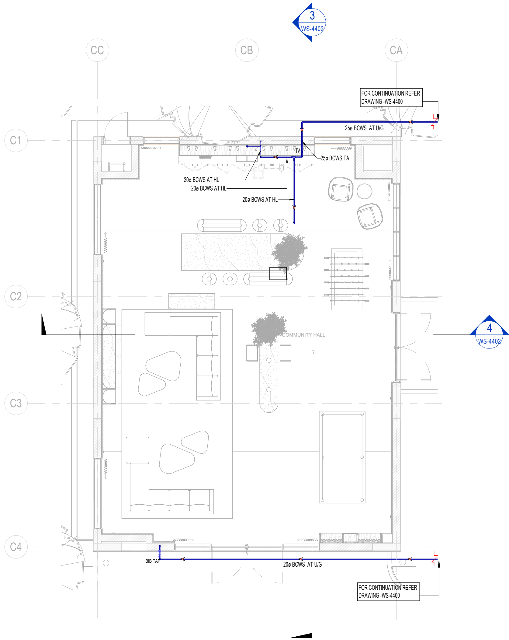
1 GROUND FLOOR WATER SUPPLY LAYOUT-COMMUNITY HALL 1 : 75
