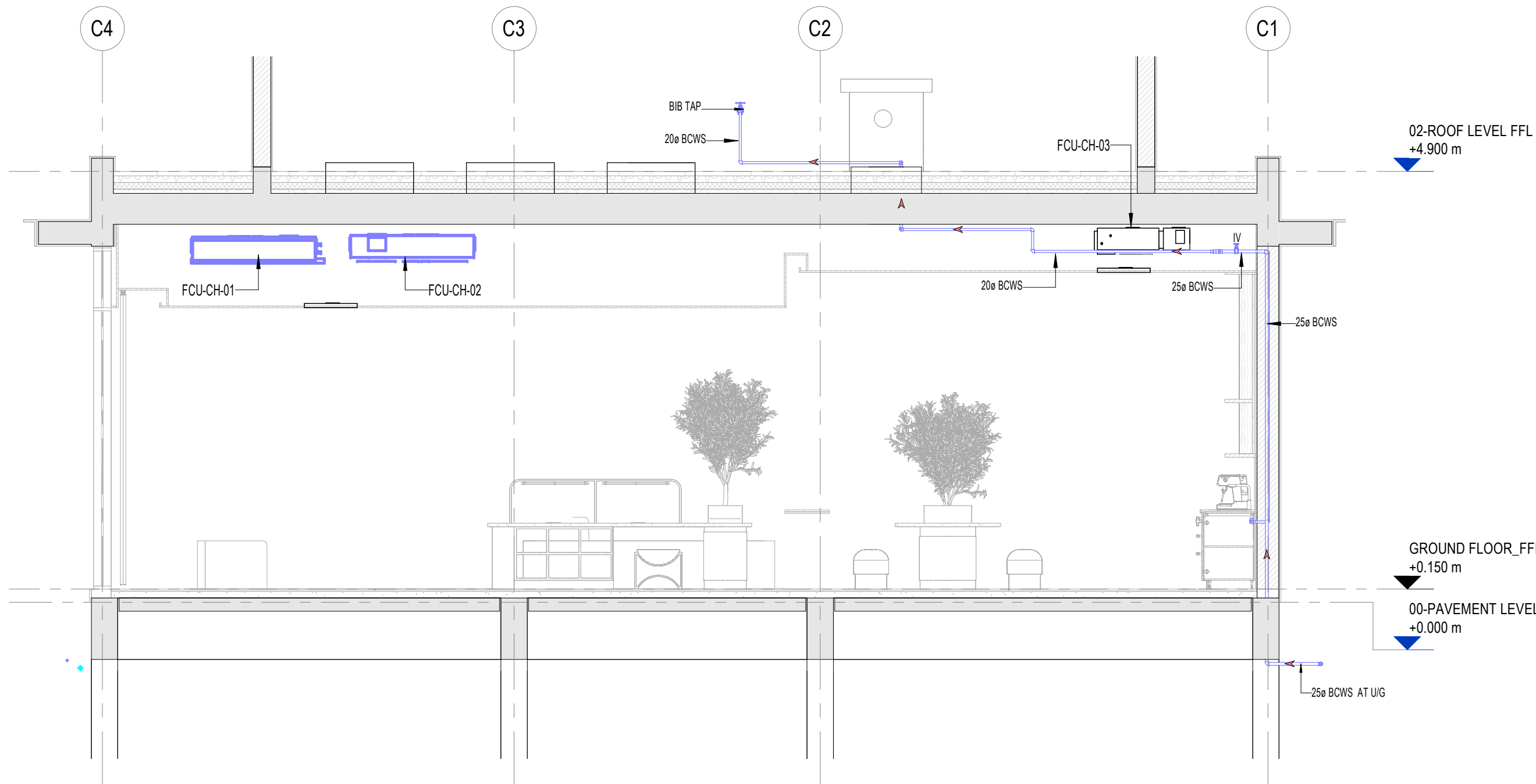
3 COMMUNITY HALL WATER SUPPLY SECTION 01 1 : 50
