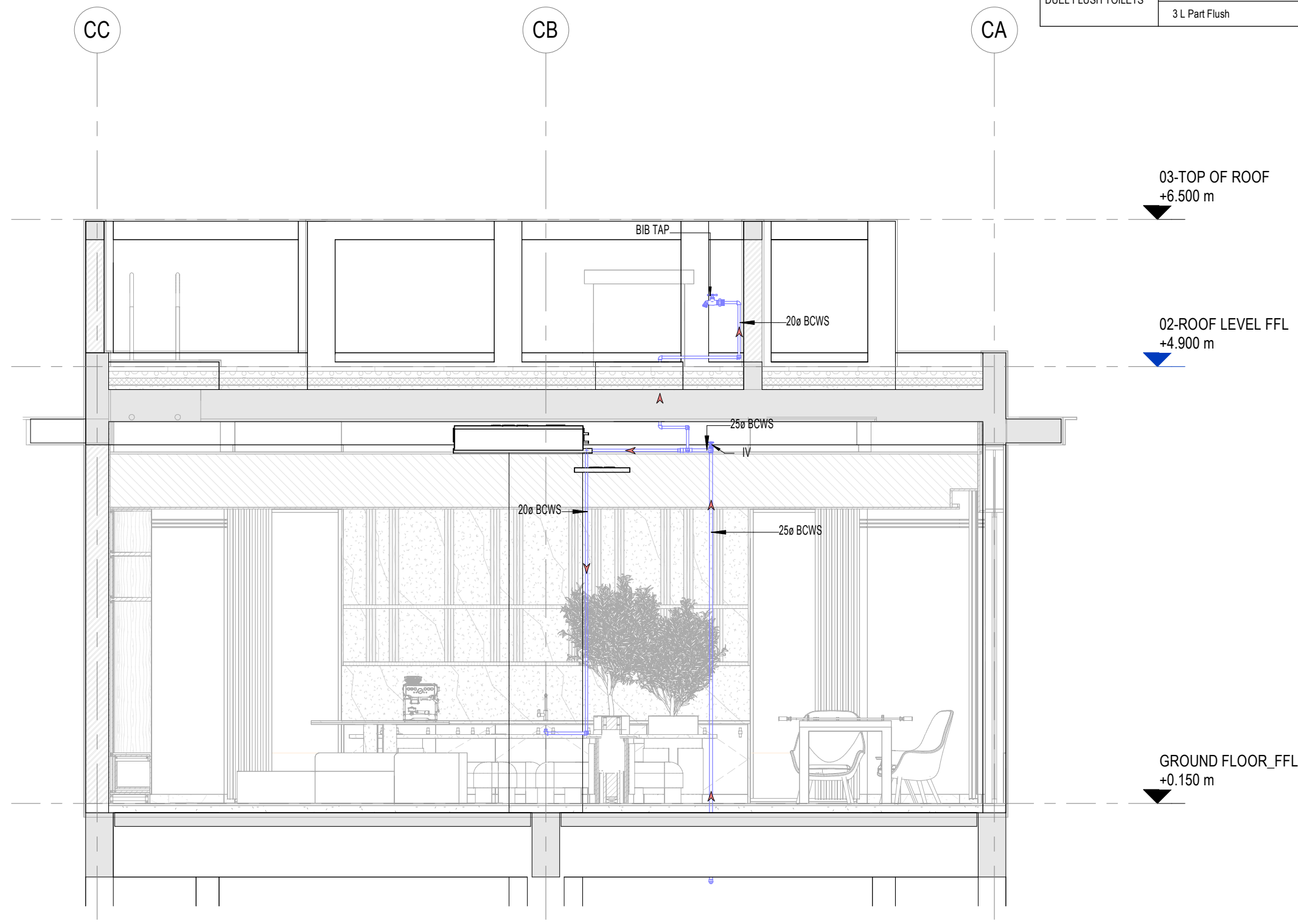
4 COMMUNITY HALL WATER SUPPLY SECTION 02 1 : 50
