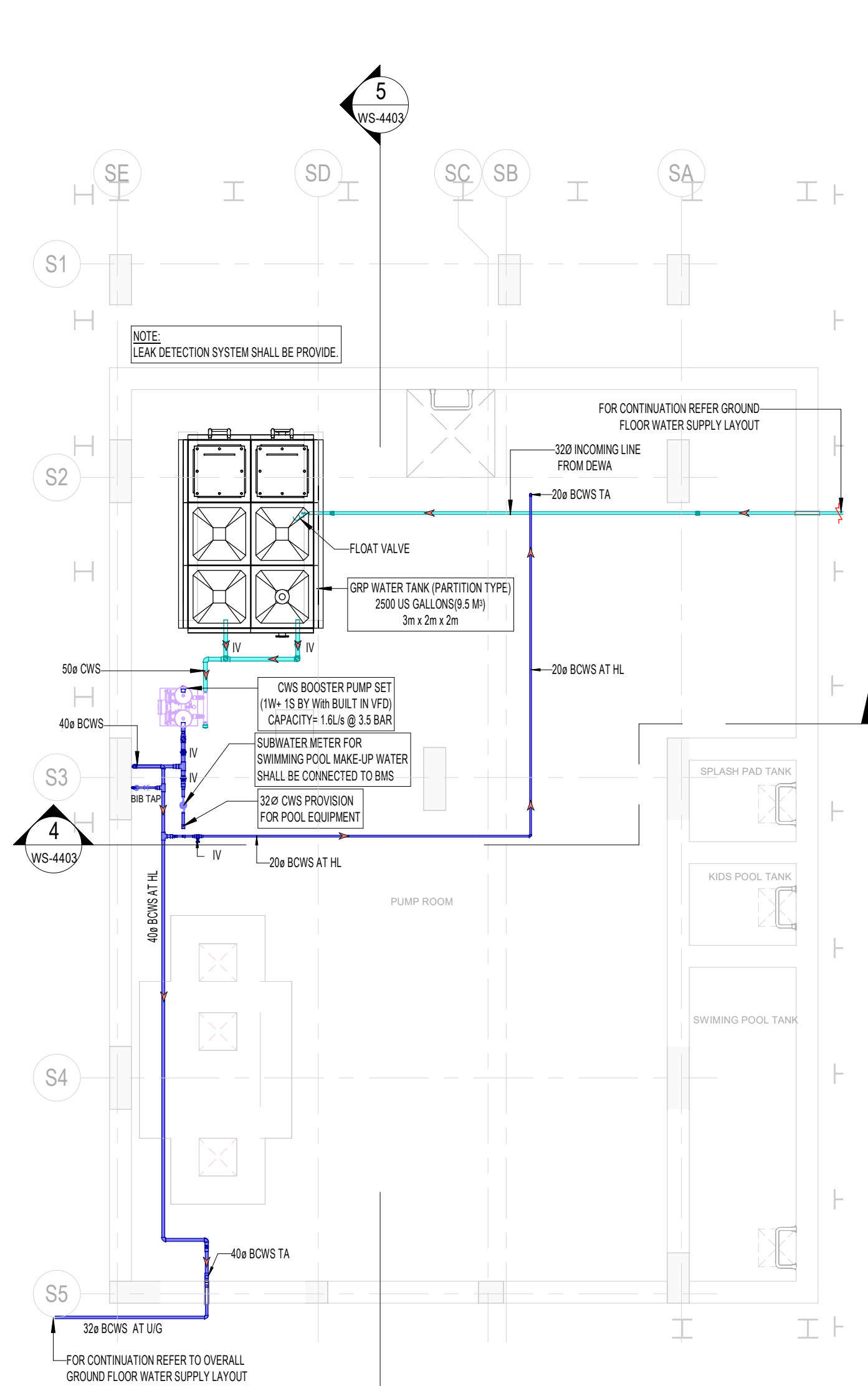
1 BASEMENT FLOOR WATER SUPPLY LAYOUT 1 : 75
