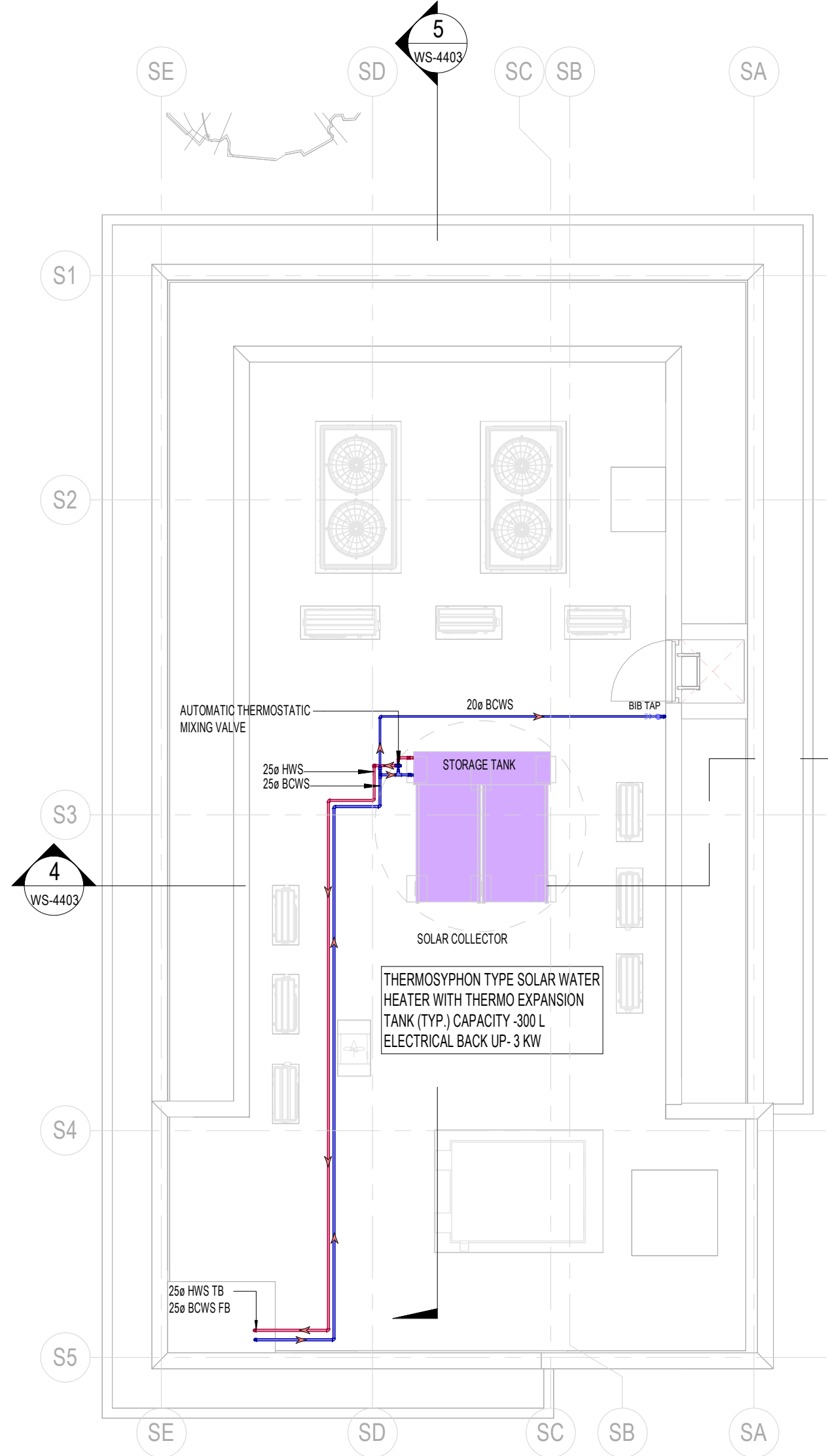
3 ROOF FLOOR WATER SUPPLY LAYOUT 1 : 75
