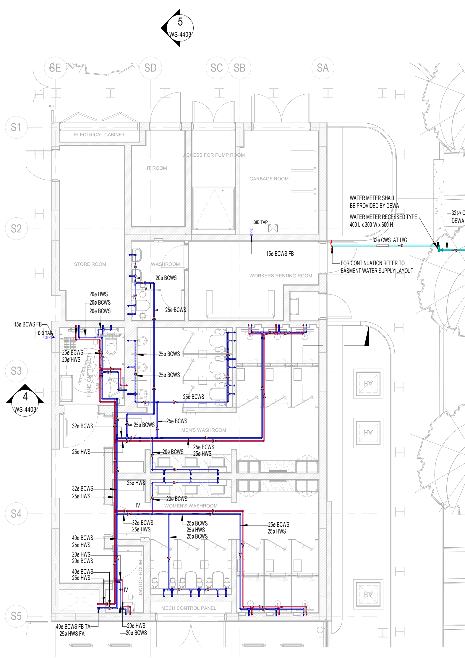
2 GROUND FLOOR_ WATER SUPPLY LAYOUT 1 : 75
