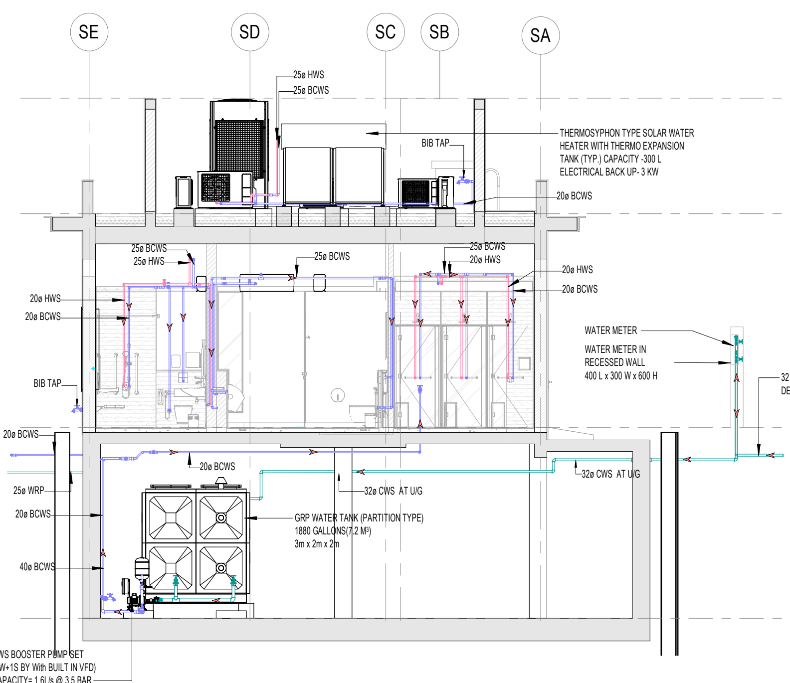
4 SERVICE BLOCK WATER SUPPLY SECTION 01 1 : 75
