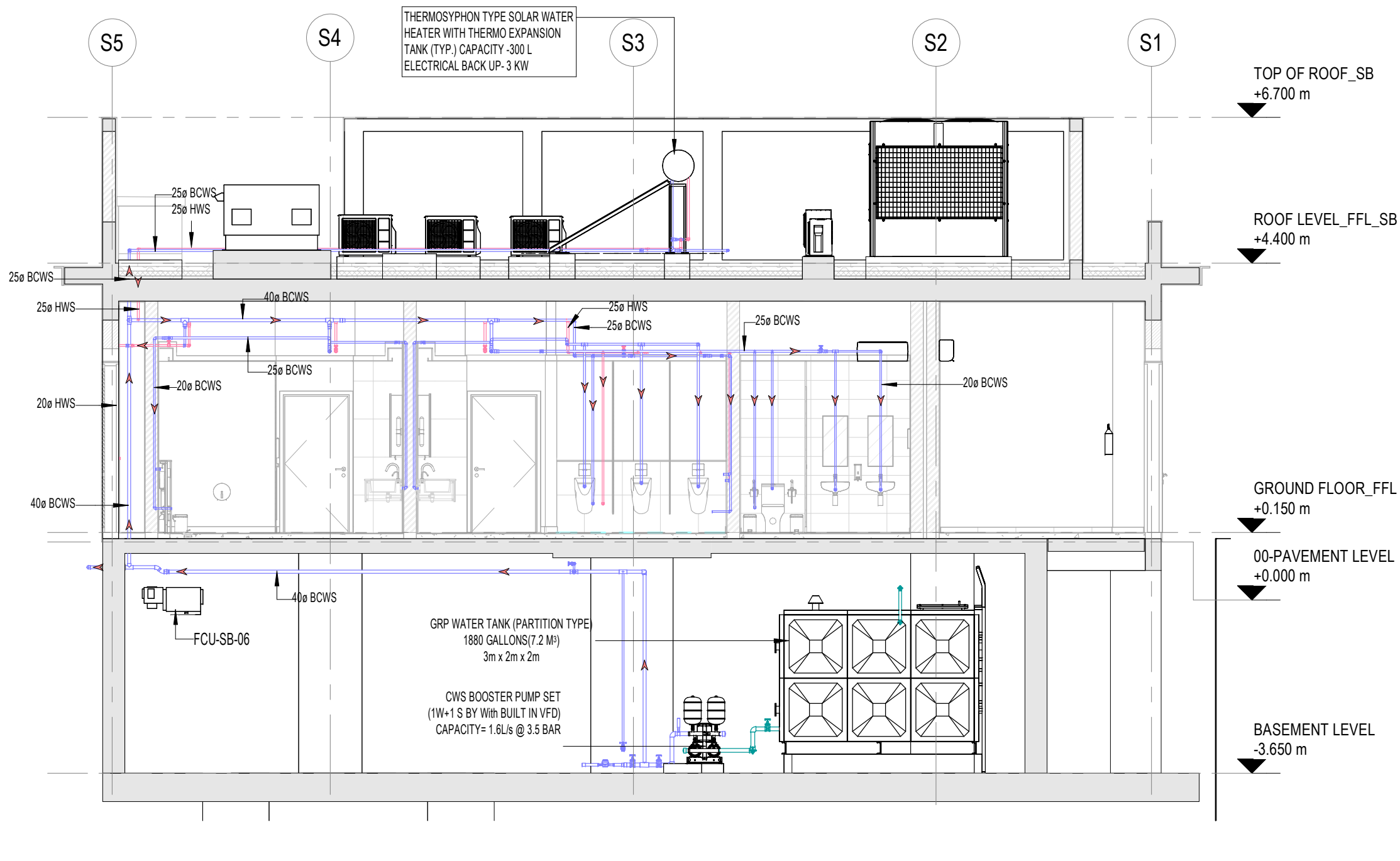
5 SERVICE BLOCK WATER SUPPLY SECTION 02 1 : 75
