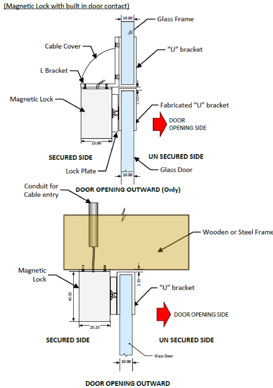
5 DOOR CONTACT & ELECTRO MAGNETIC LOCK TYPICAL POSITIONING IN GLASS DOOR NOT TO SCALE
