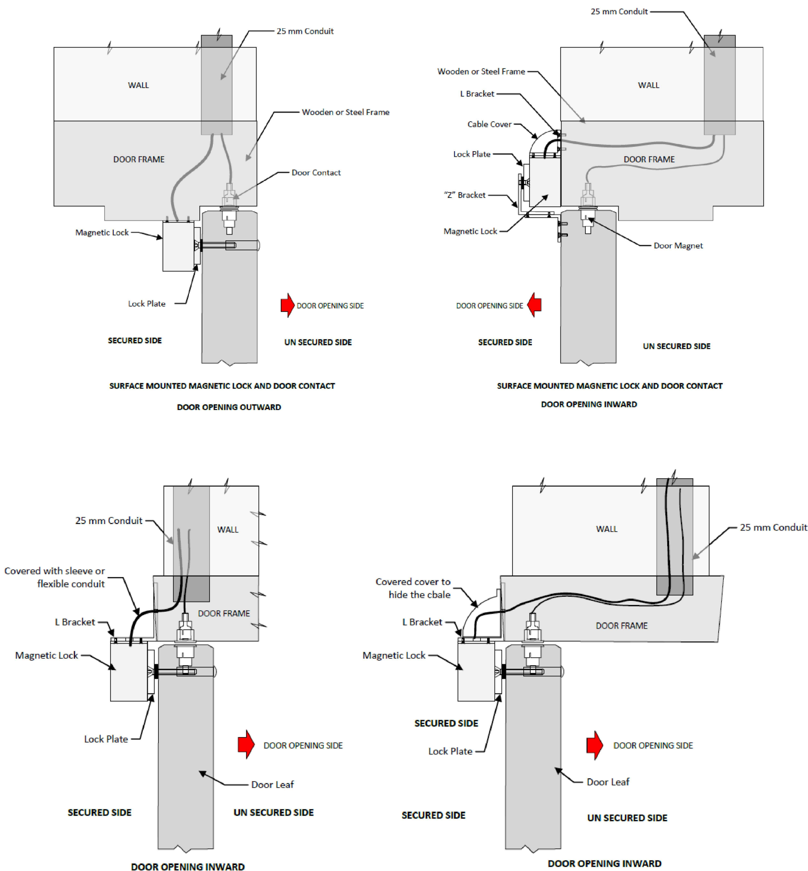
4 DOOR CONTACT & ELECTRO MAGNETIC LOCK TYPICAL POSITIONING IN WOOD OR STEEL DOOR NOT TO SCALE
