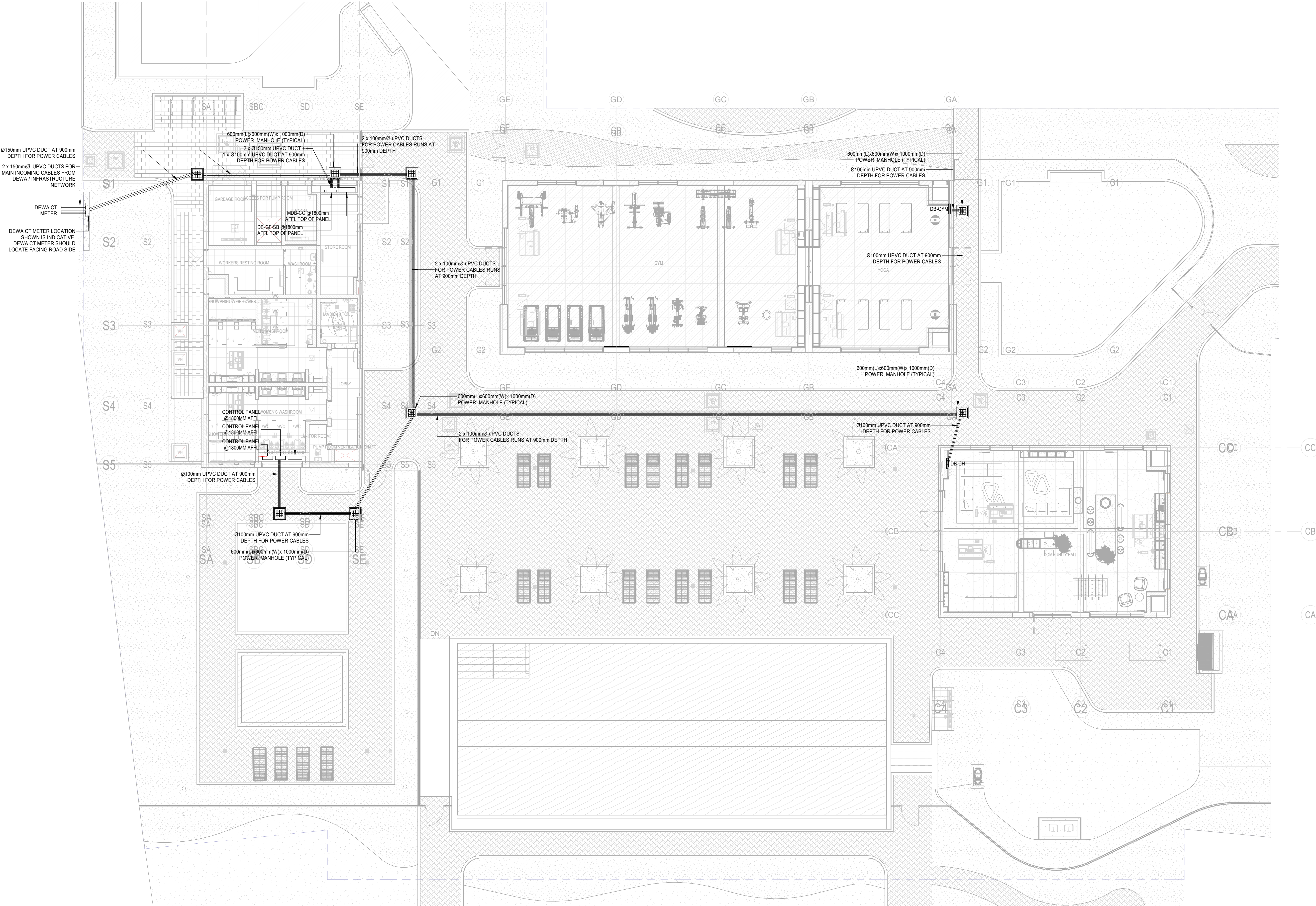
1 COMMUNITY CENTRE POWER SETTING OUT PLAN 1 : 110
