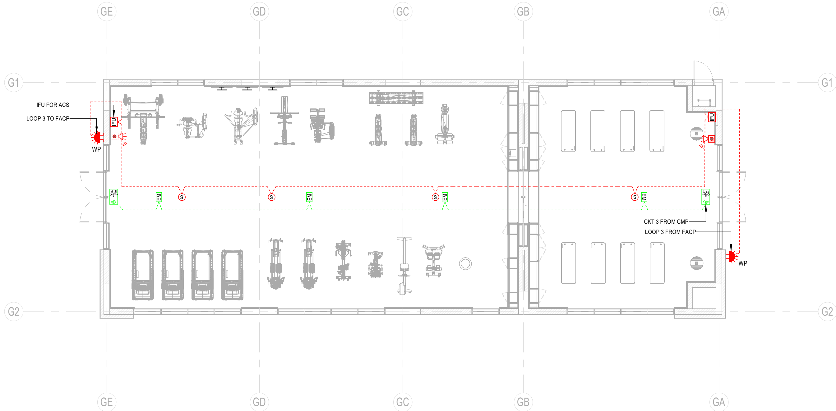
1 01-GROUND FLOOR GYM FIRE ALARM & EMERGENCY 1 : 100
