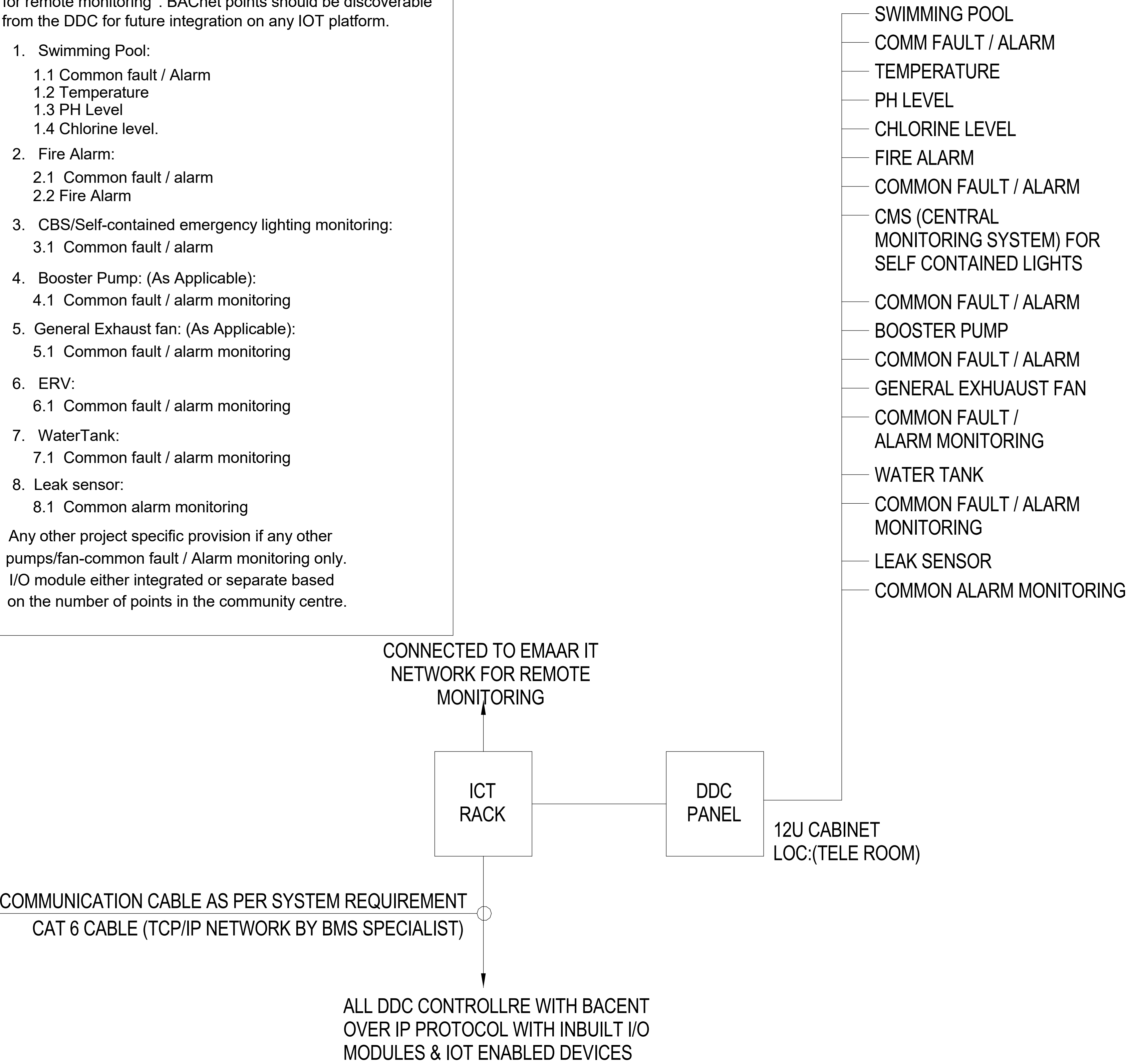
SYSTEM ARCHITECTURE - STANDALONE BMS SYSTEM)
