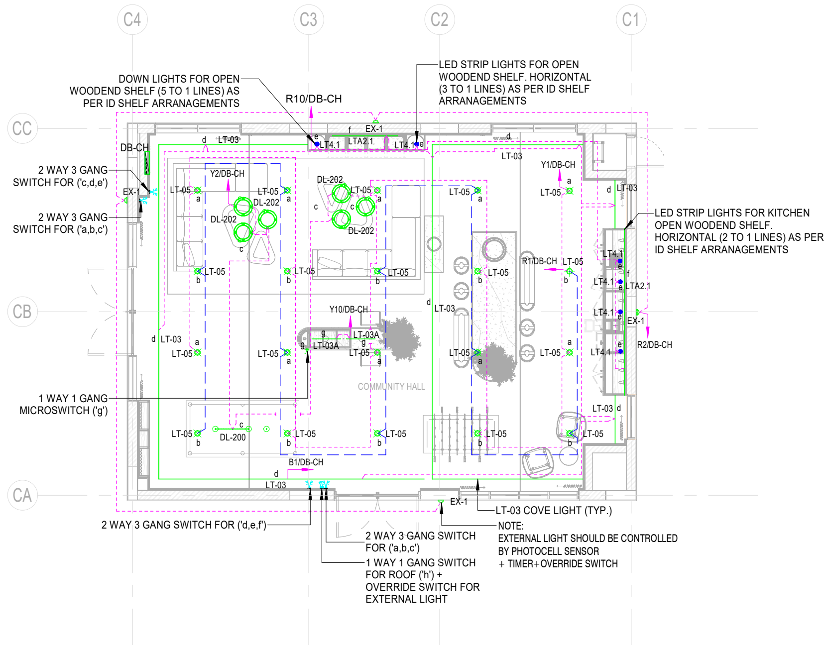
1 01-GROUND FLOOR COMMUNITY HALL LIGHTING 1 : 100
