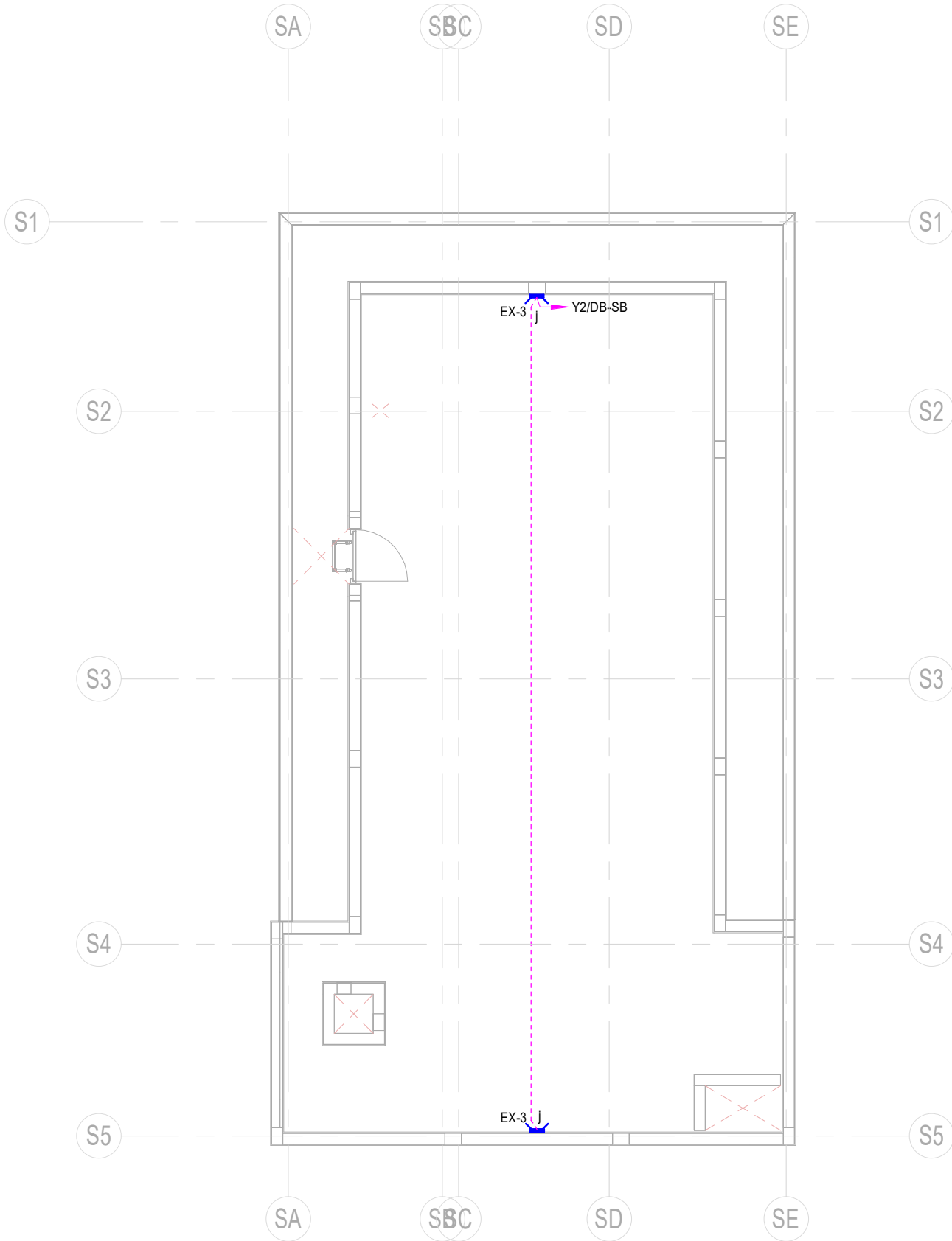
3 02-ROOF SERVICE BLOCK LIGHTING 1 : 100
