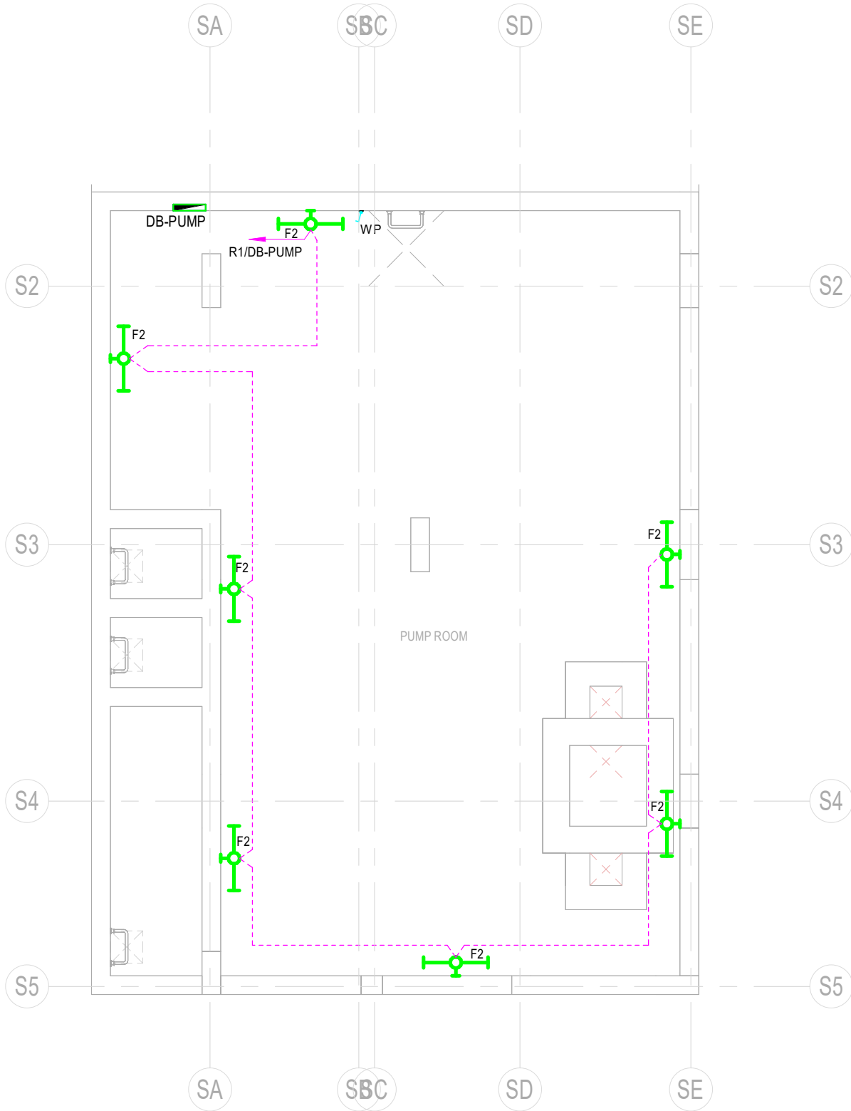
1 00-U.W.T SERVICE BLOCK LIGHTING 1 : 100
