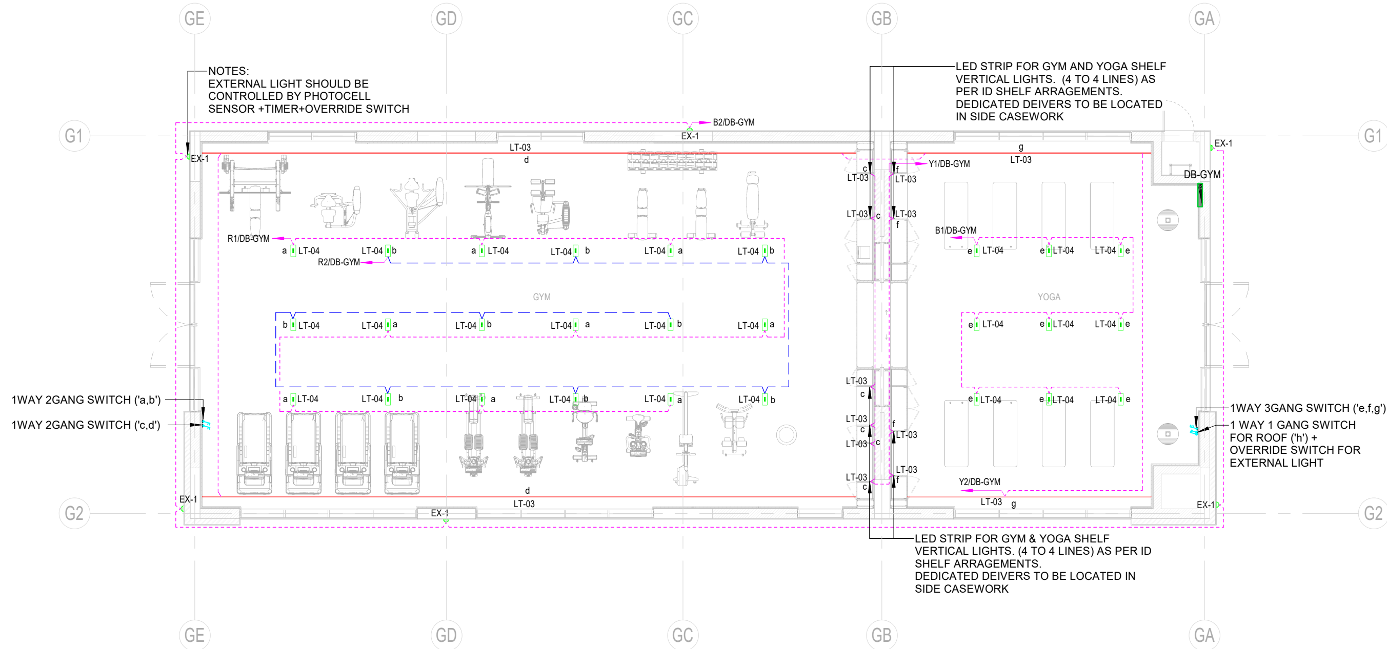
1 01-GROUND FLOOR GYM LIGHTING 1 : 100
