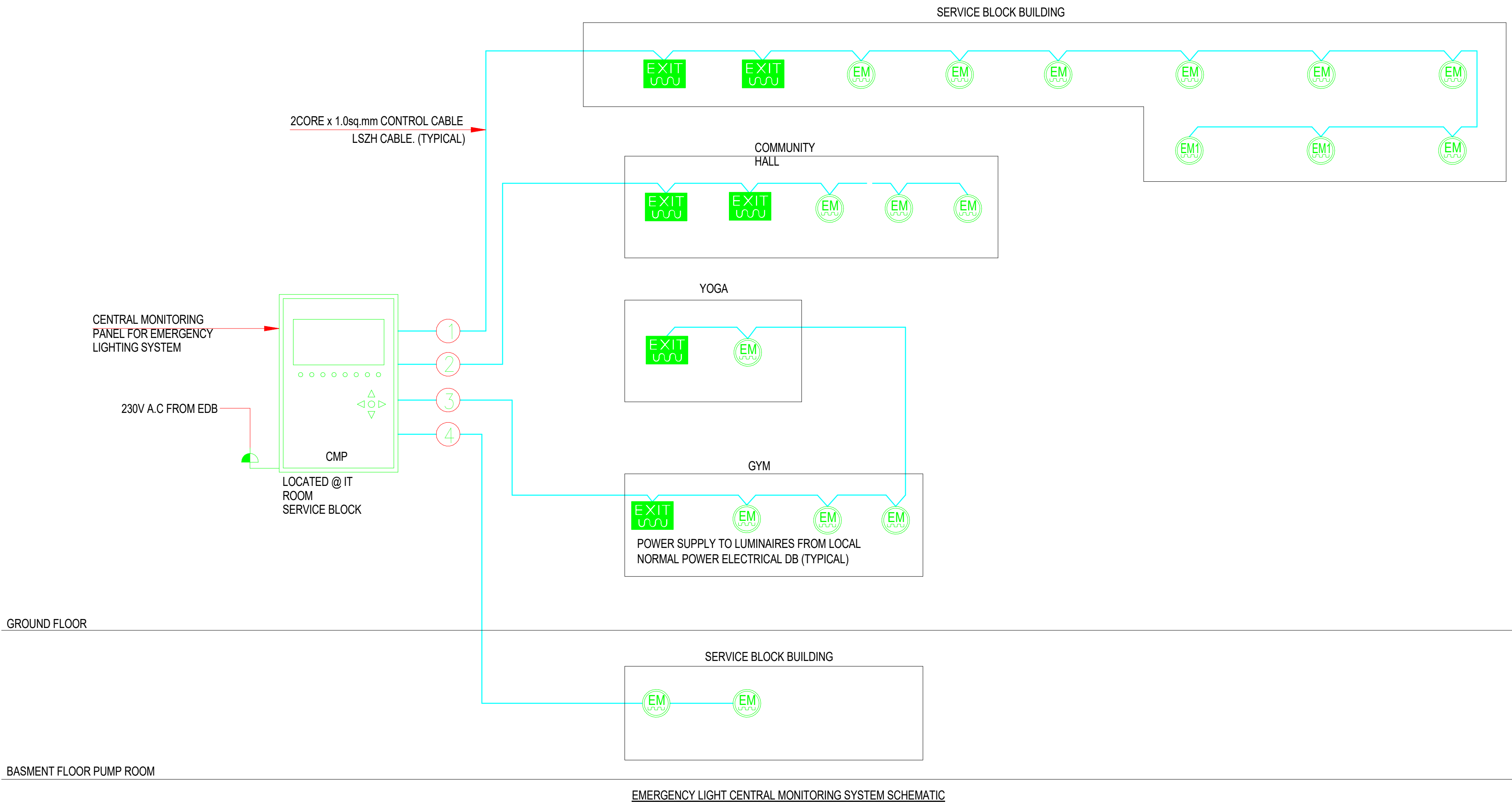
EMERGENCY LIGHT CENTRAL MONITORING SYSTEM SCHEMATIC
