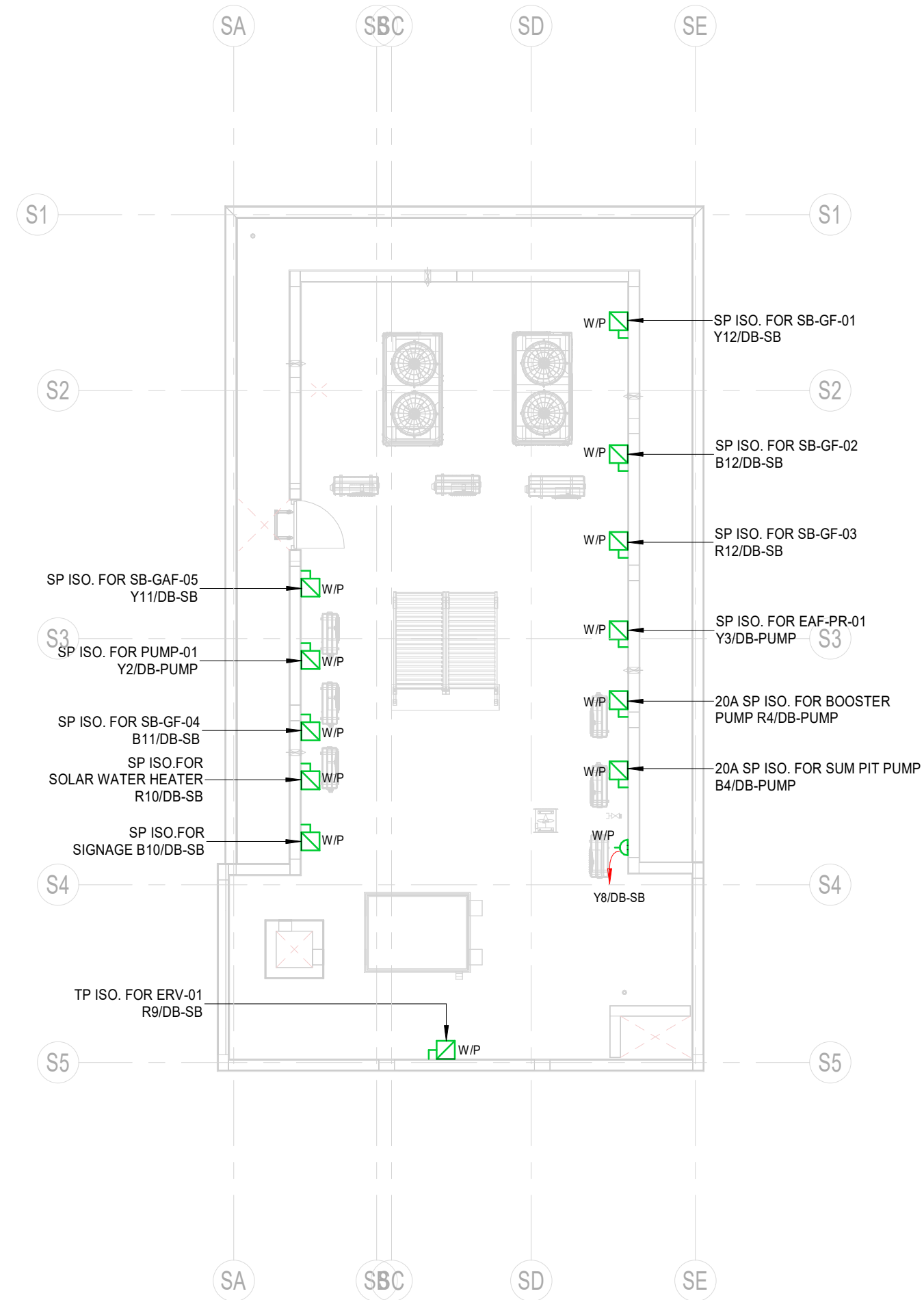
3 02-ROOF SERVICE BLOCK POWER 1 : 100
