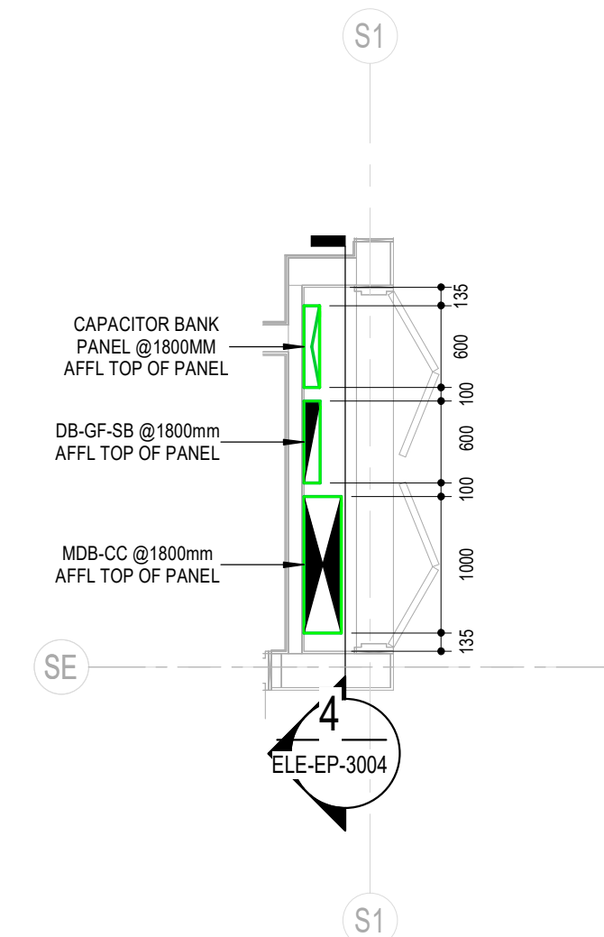
SERVICE BLOCK ELE.CABINET DETAILS
