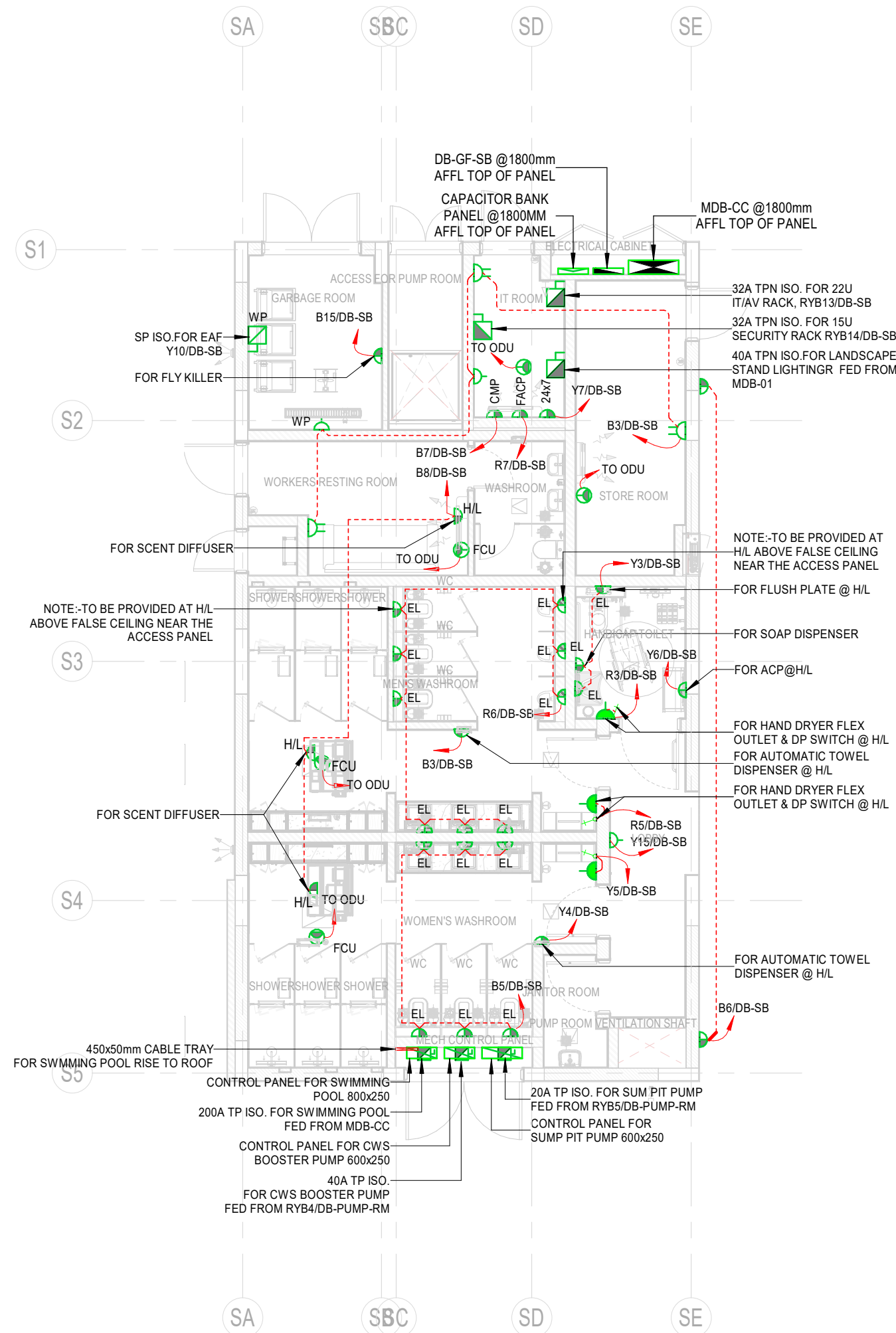
2 01-GROUND FLOOR SERVICE BLOCK POWER 1 : 100
