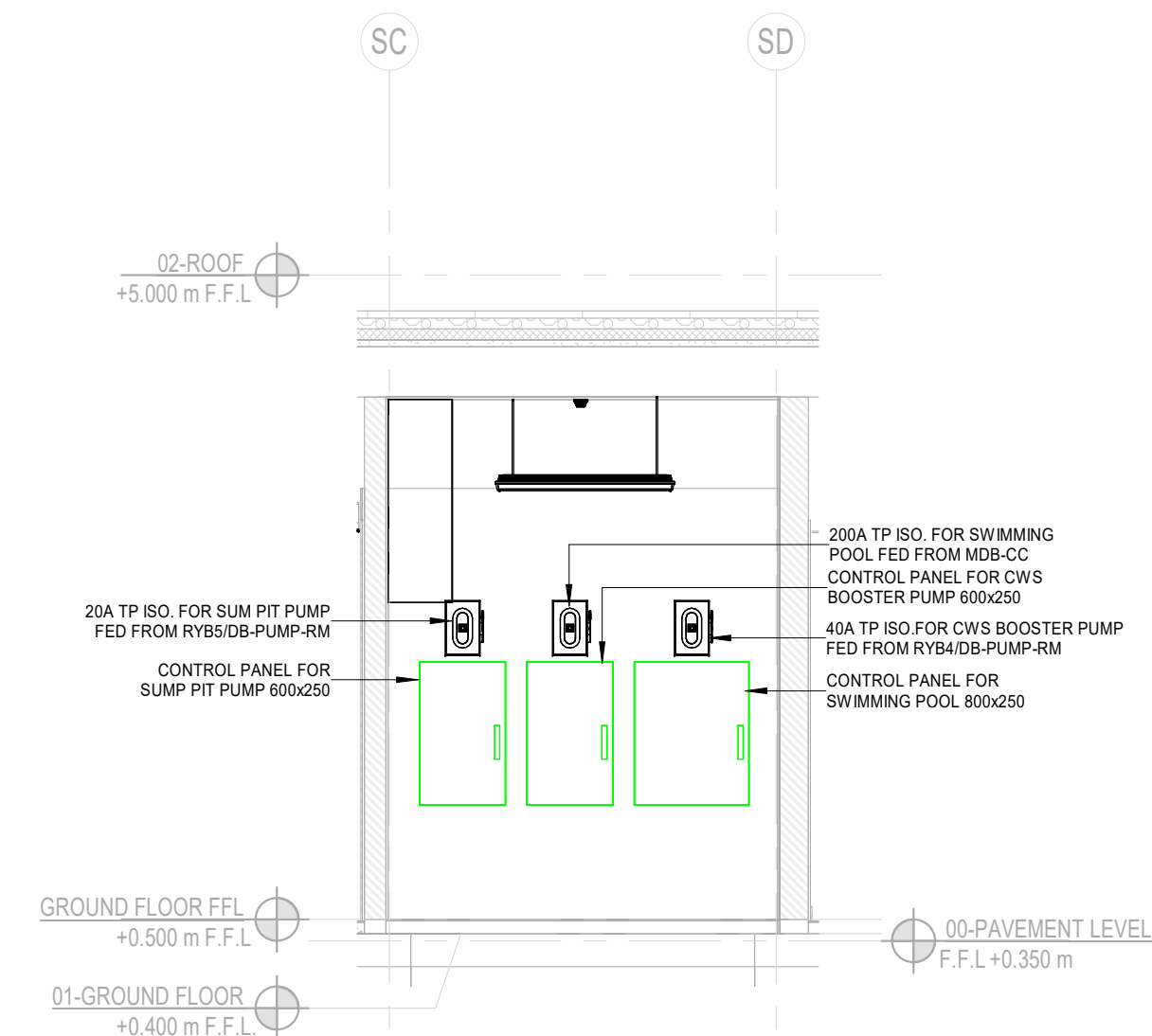
5 PUMP ROOM ELE. CABINET DETAILS SECTION 1 : 50
