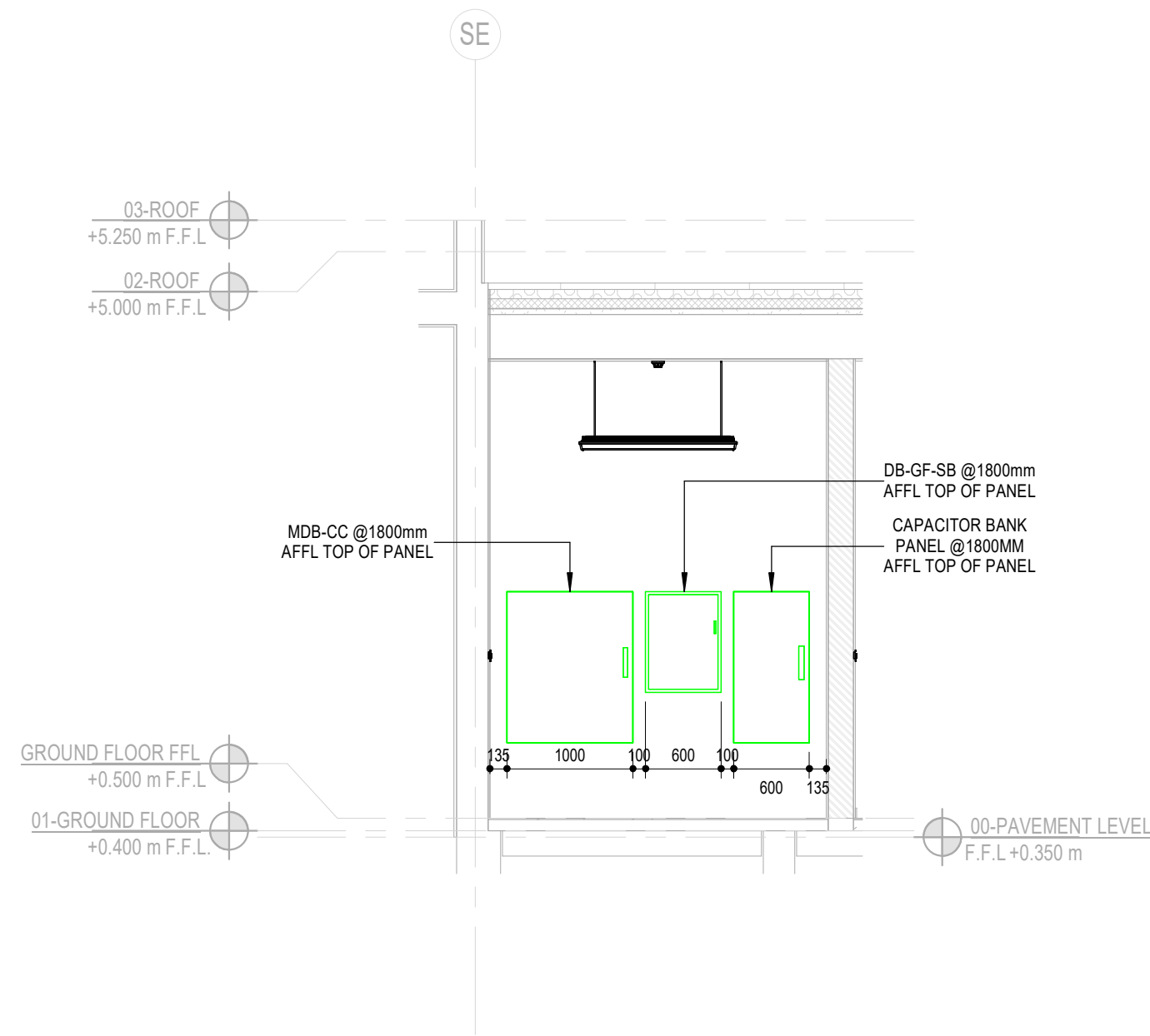
4 SERVICE BLOCK ELE. CABINET SECTION 1 : 50
