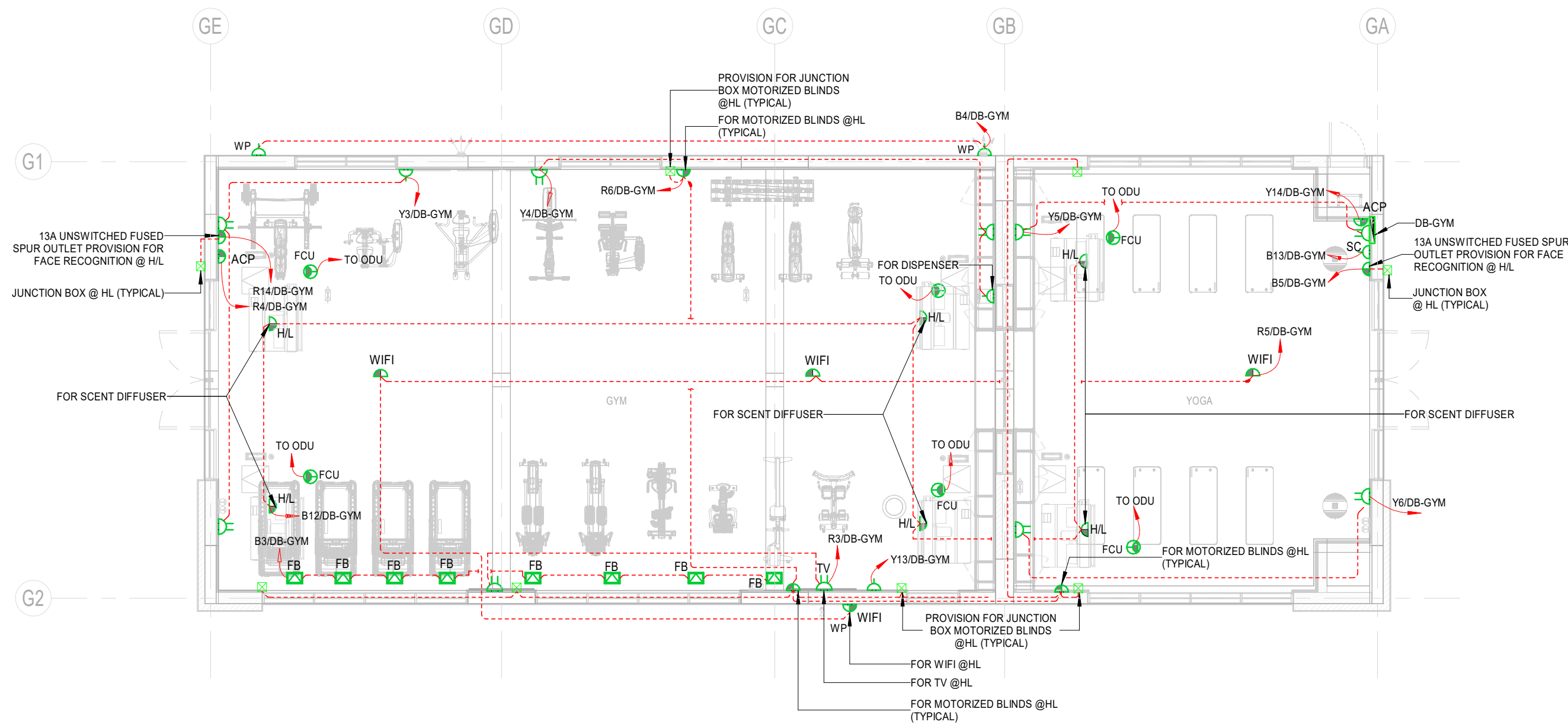
1 01-GROUND FLOOR GYM POWER 1 : 100
