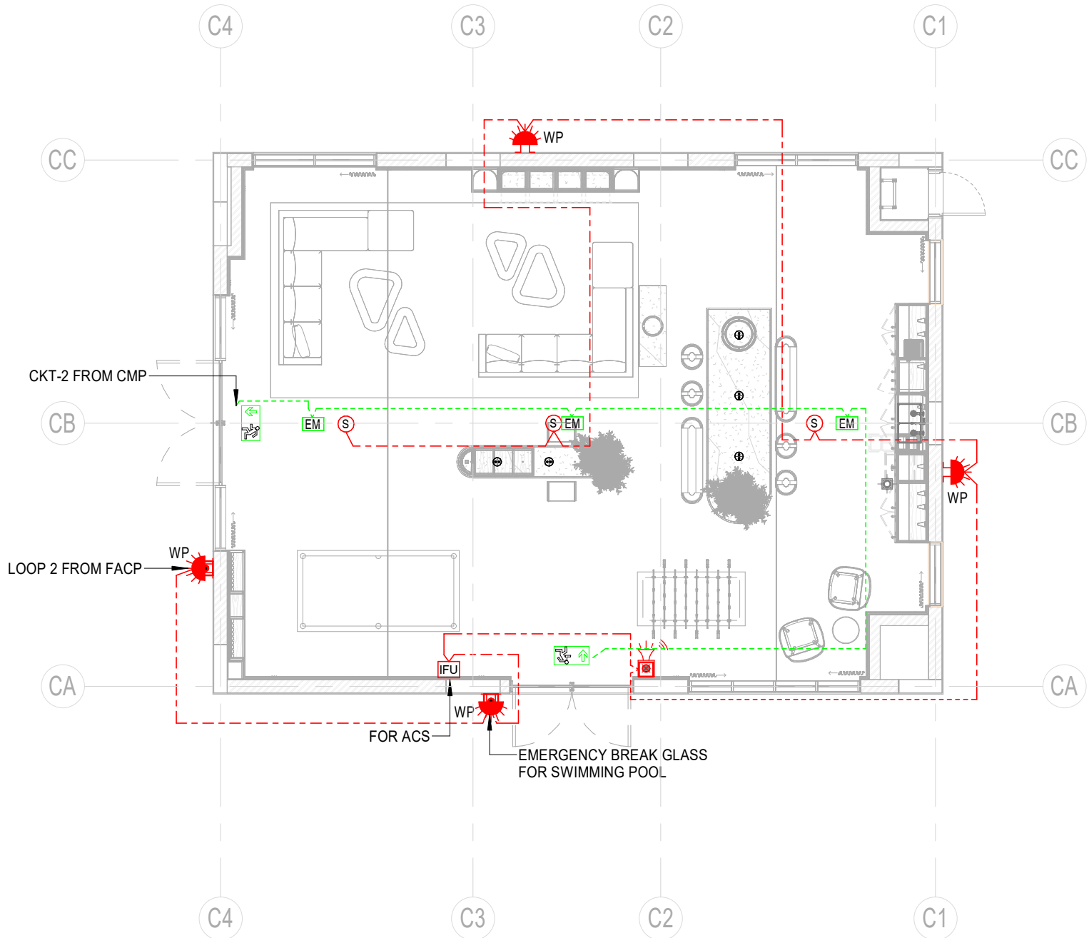
1 01-GROUND FLOOR COMMUNITY FIRE ALARM & EMERGENCY 1 : 100
