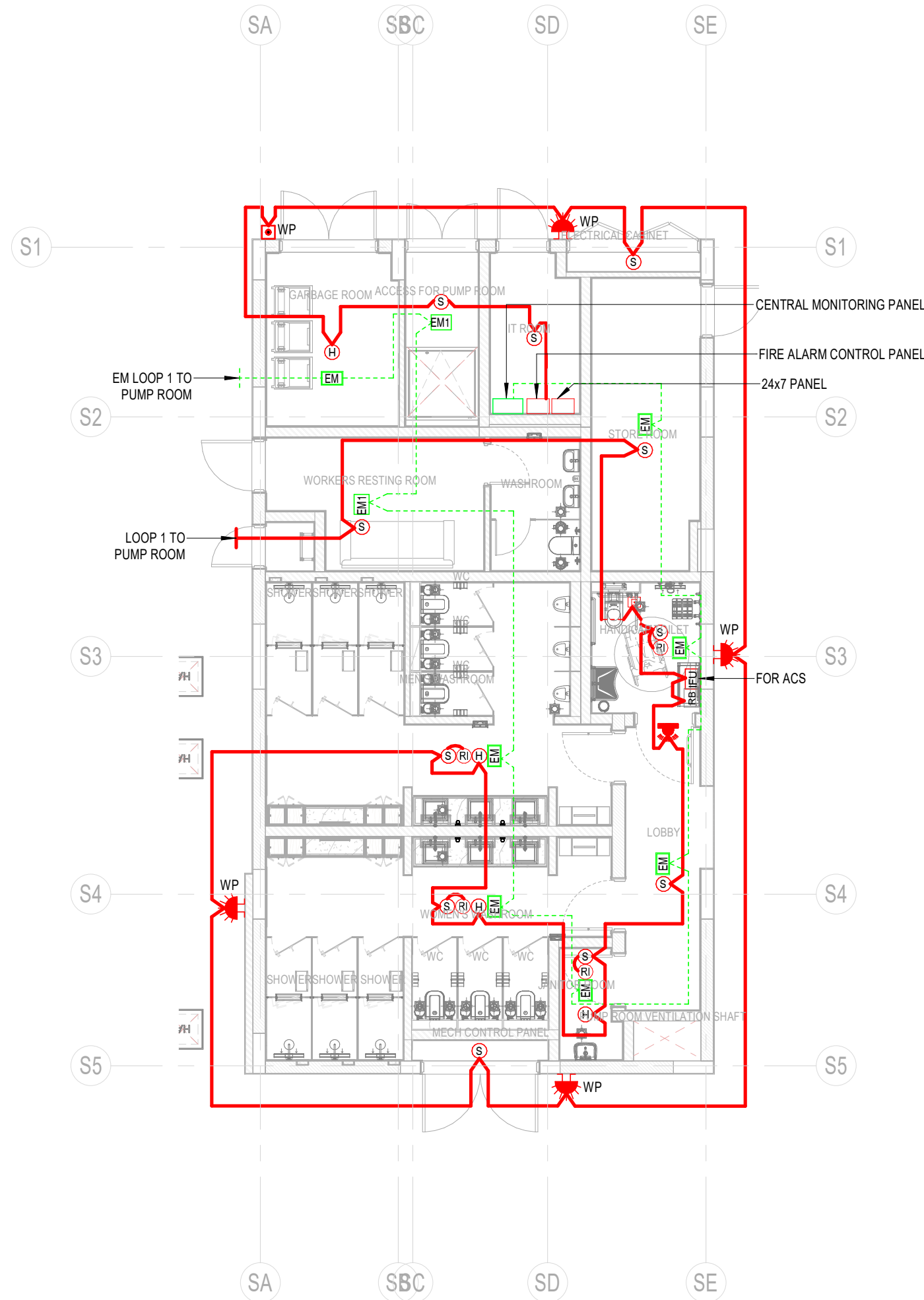
1 01-GROUND FLOOR SERVICE BLOCK FIRE ALARM & EMERGENCY 1 : 100
