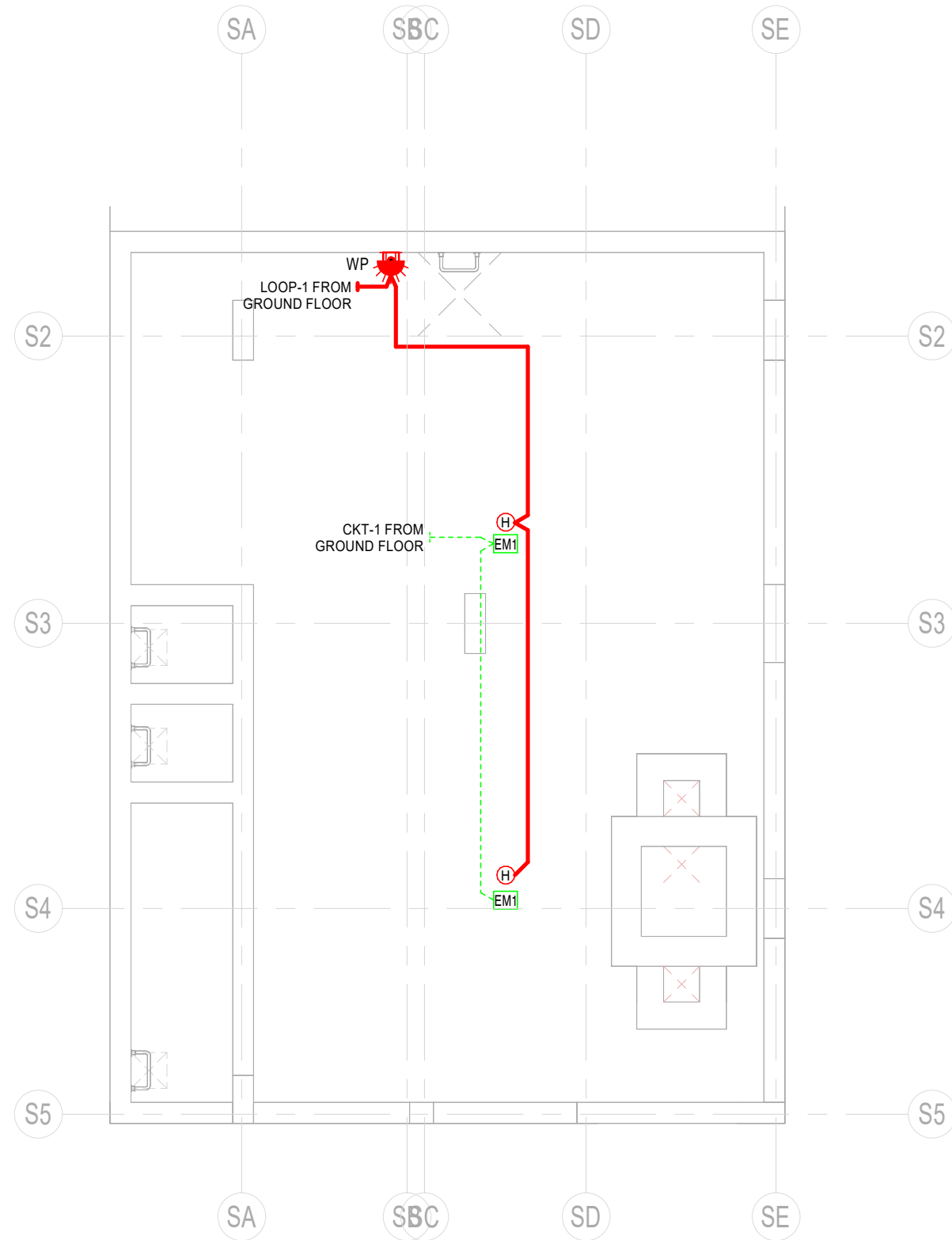
2 00-U.W.T SERVICE BLOCK FIRE ALARM & EMERGENCY 1 : 100
