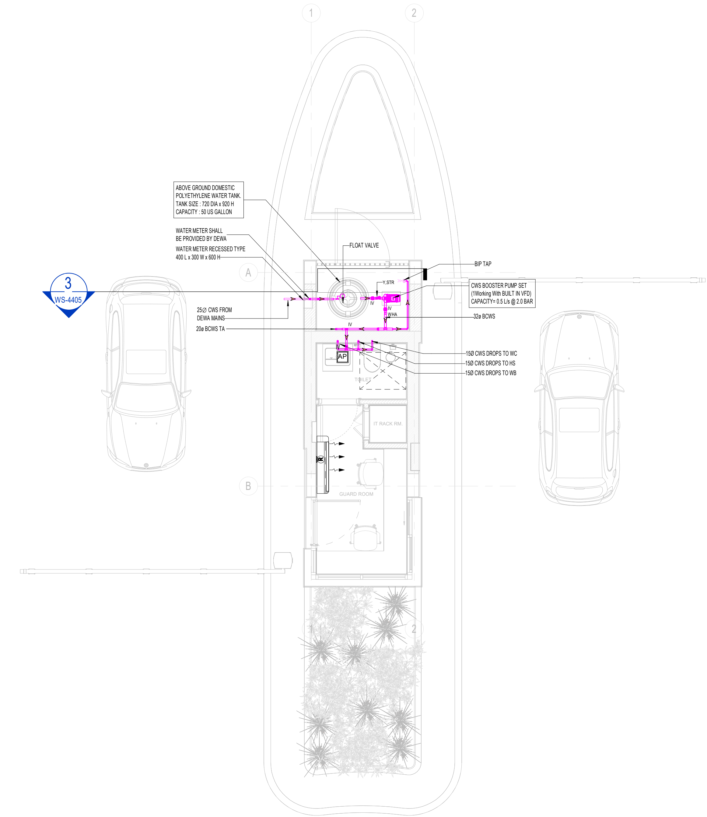
2 ROOF FLOOR PLAN WATER SUPPLY LAYOUT 1 : 50
