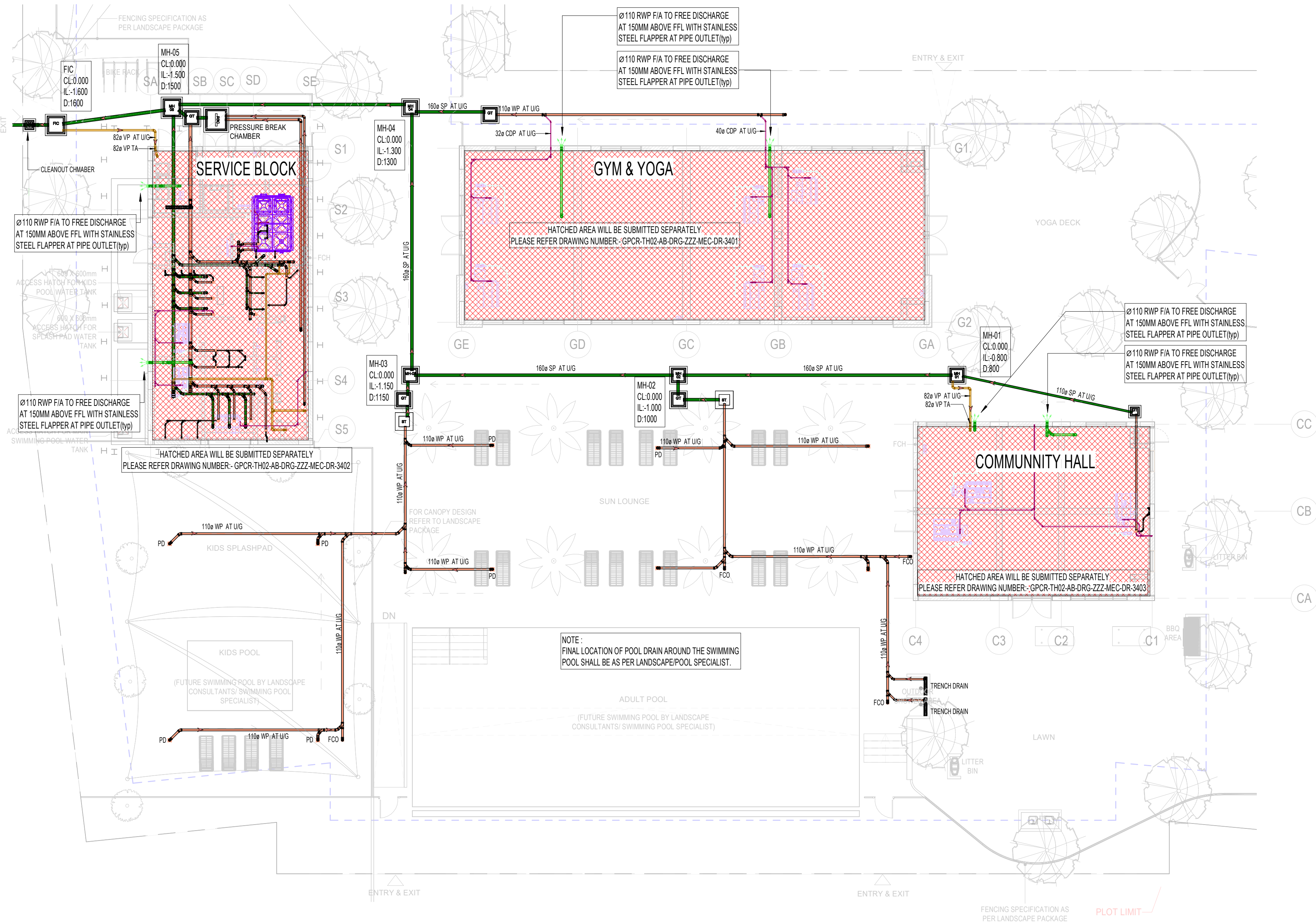
1 OVERALL GROUND FLOOR DRAINAGE LAYOUT 1 : 150
