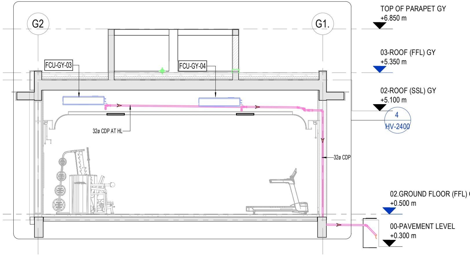
GYM&YOGA DRAINAGE SECTION 02
