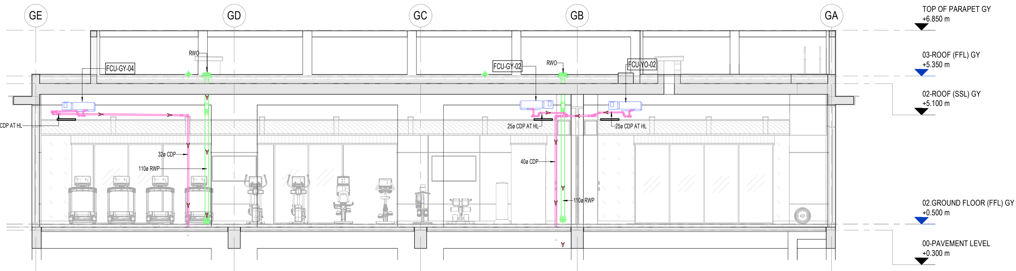
GYM&YOGA DRAINAGE SECTION 01
