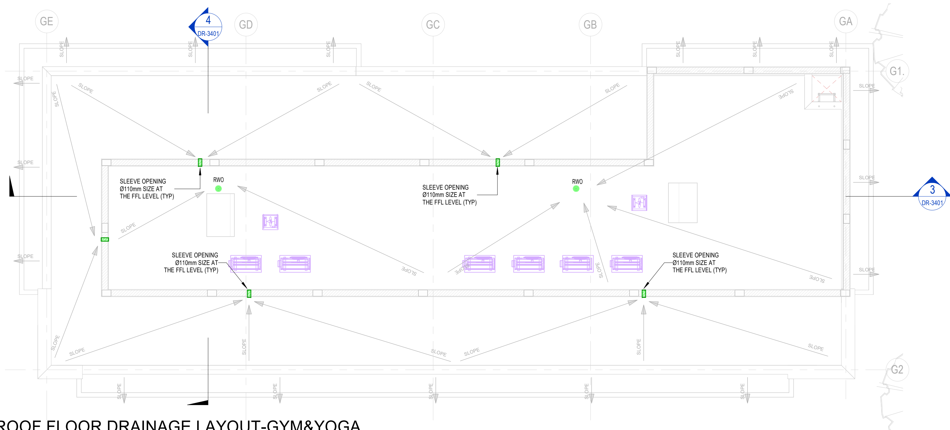
ROOF FLOOR DRAINAGE LAYOUT-GYM&YOGA
