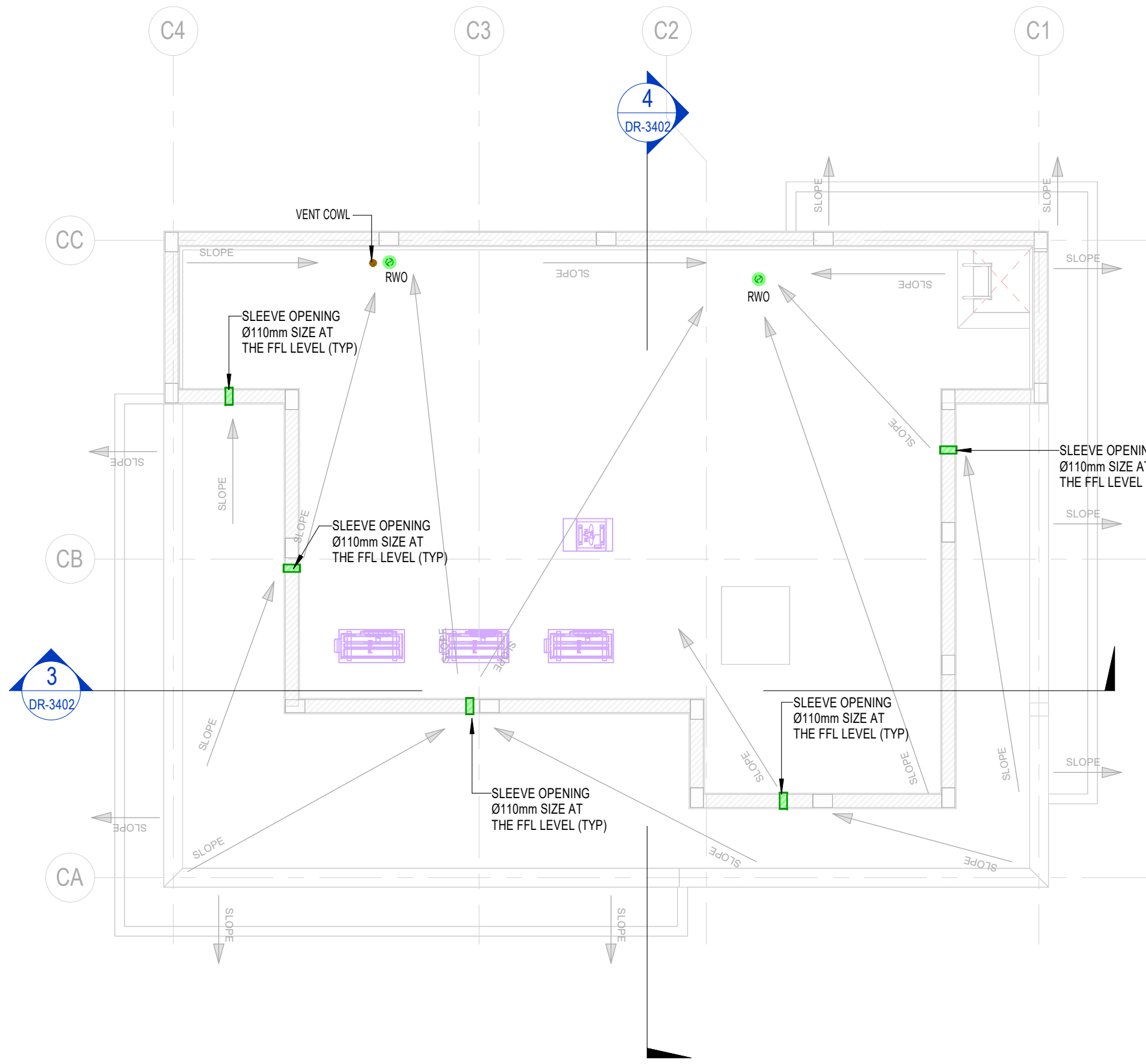
2 ROOF FLOOR DRAINAGE LAYOUT-COMMUNITY HALL 1 : 75
