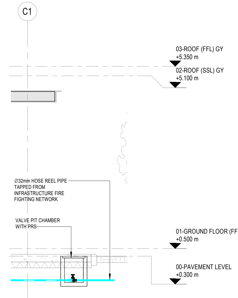
4 FIRE PROTECTION SECTION 03
