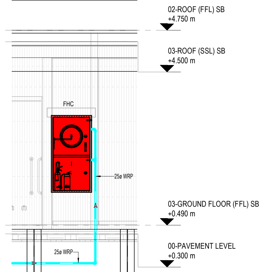
2 FIRE PROTECTION SECTION 01
