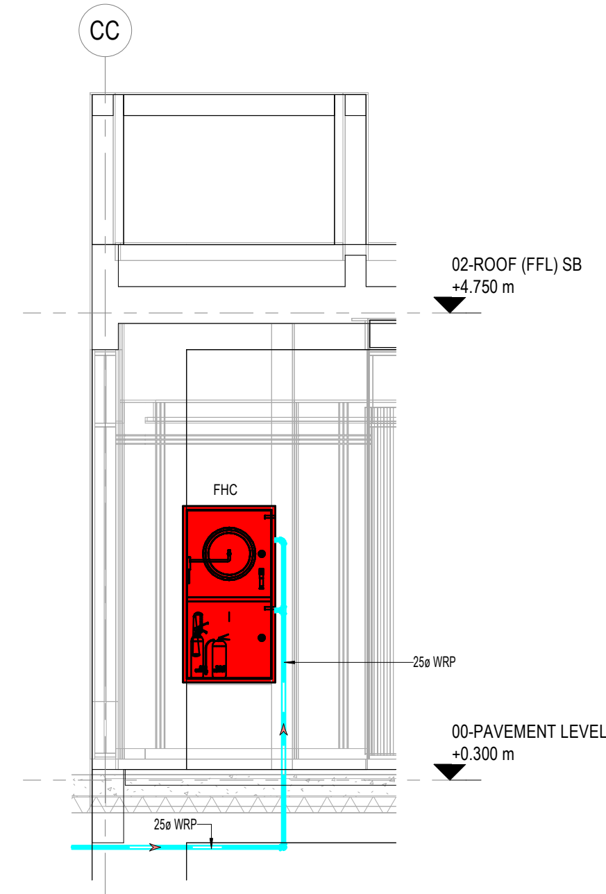
3 FIRE PROTECTION SECTION 02
