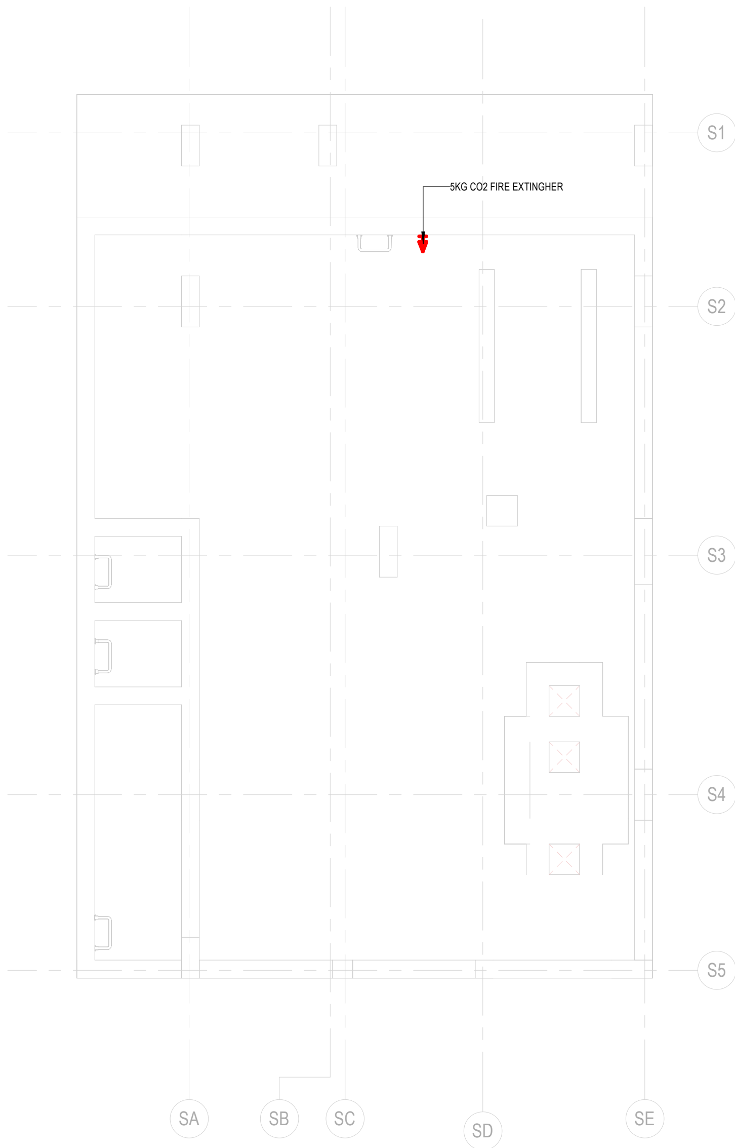
1 BASEMENT FLOOR FIRE LAYOUT 1 : 75
