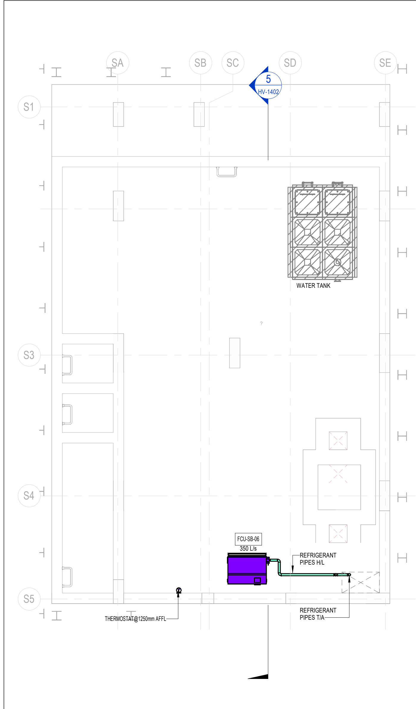
1 BASEMENT FLOOR HVAC LAYOUT 1 : 75
