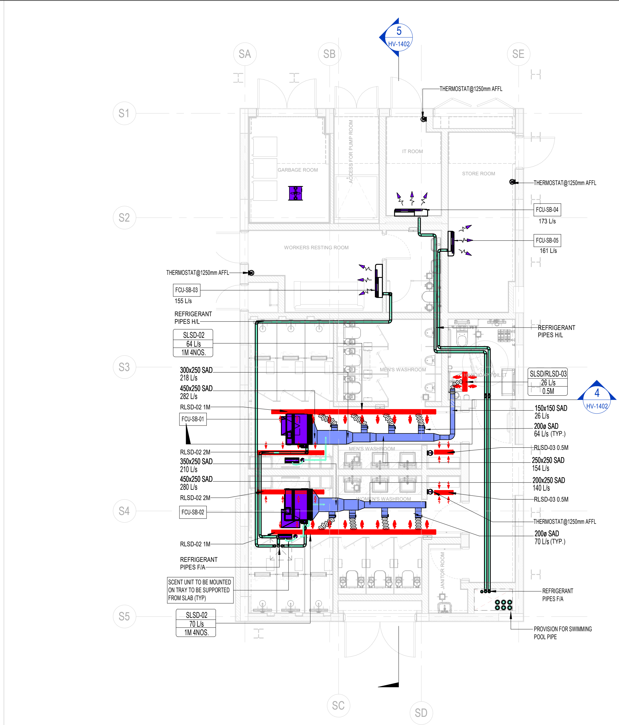
2 GROUND FLOOR HVAC LAYOUT-SERVICE BLOCK 1 : 75
