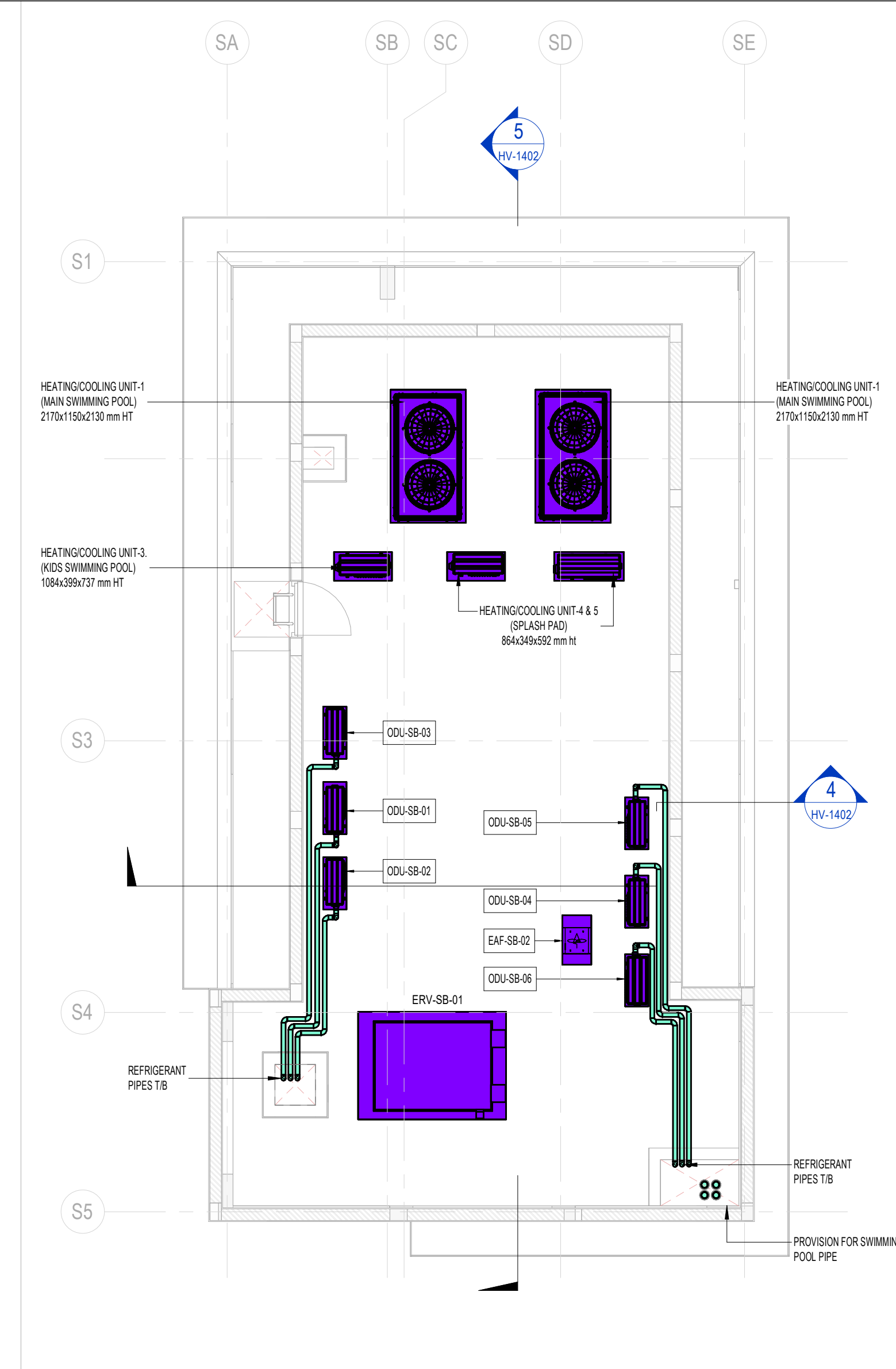
3 ROOF FLOOR HVAC LAYOUT-SERVICE BLOCK 1 : 75
