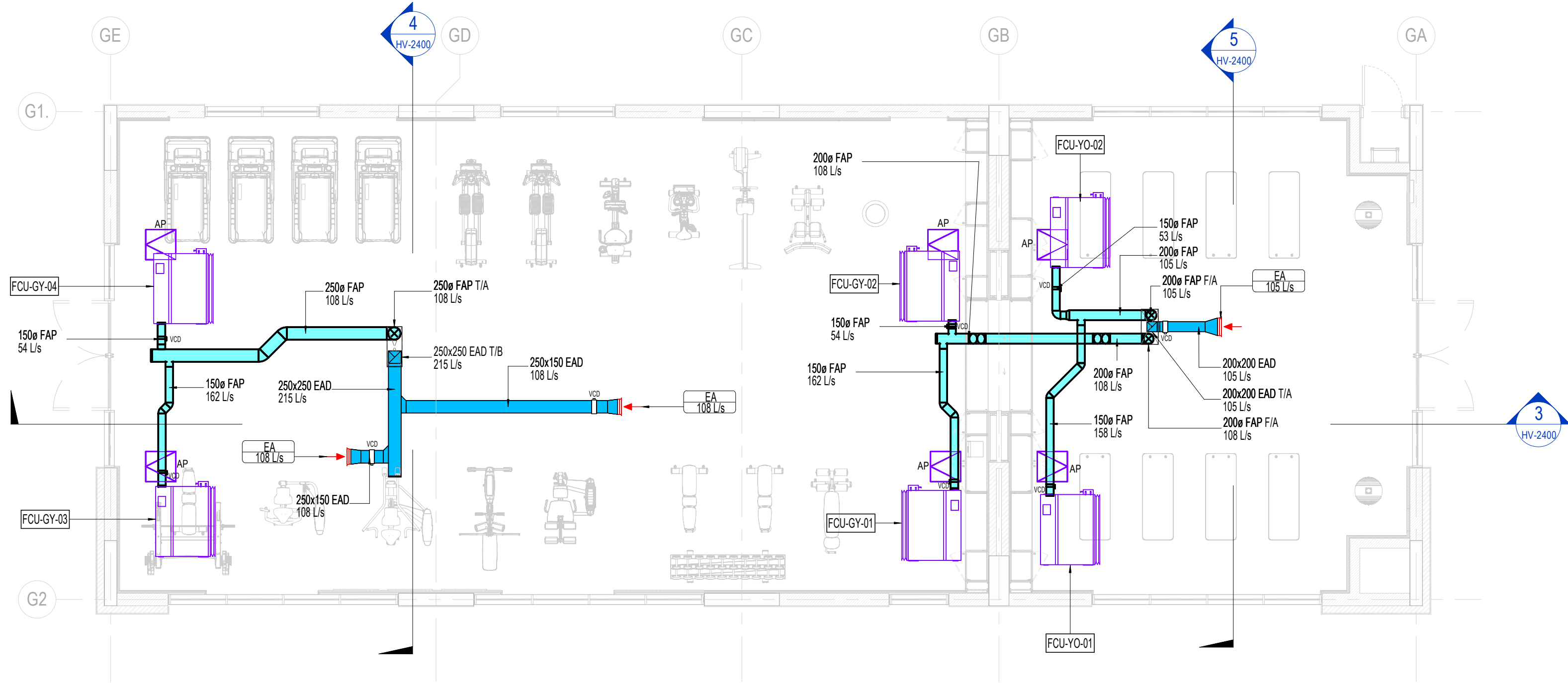
1 GROUND FLOOR VENTILATION LAYOUT-GYM&YOGA 1 : 75
