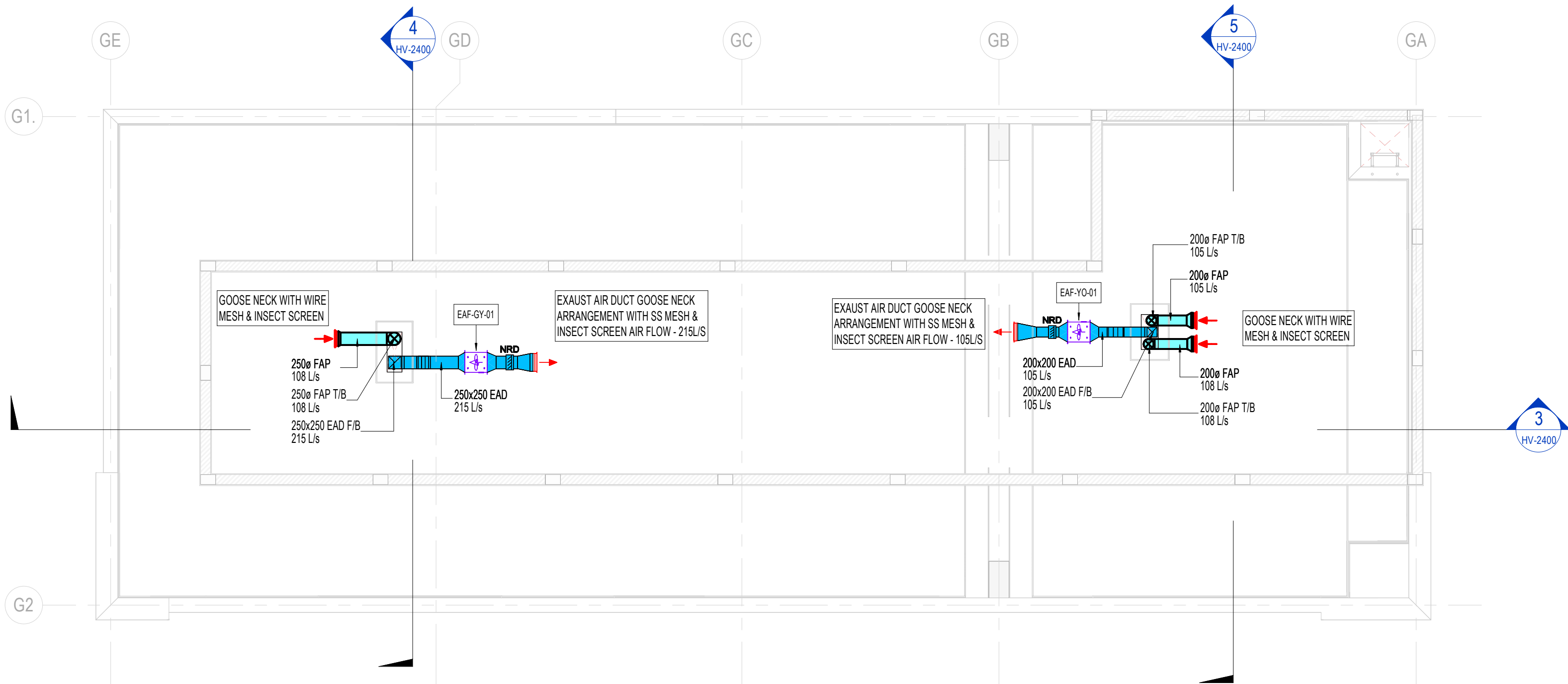
2 ROOF FLOOR VENTILATION LAYOUT-GYM&YOGA 1 : 75
