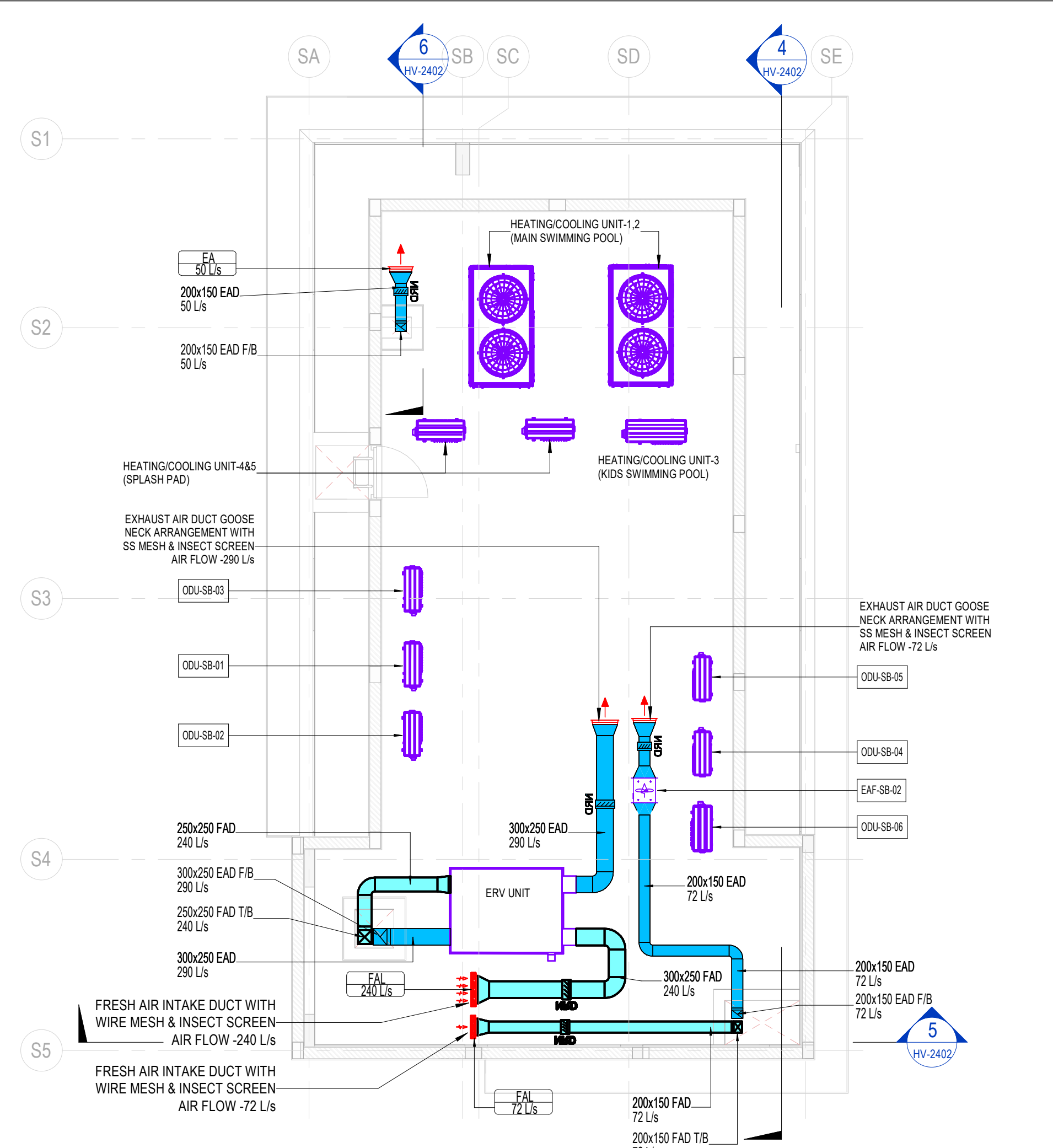
3 ROOF FLOOR VENTILATION LAYOUT-SERVICE BLOCK 1 : 75
