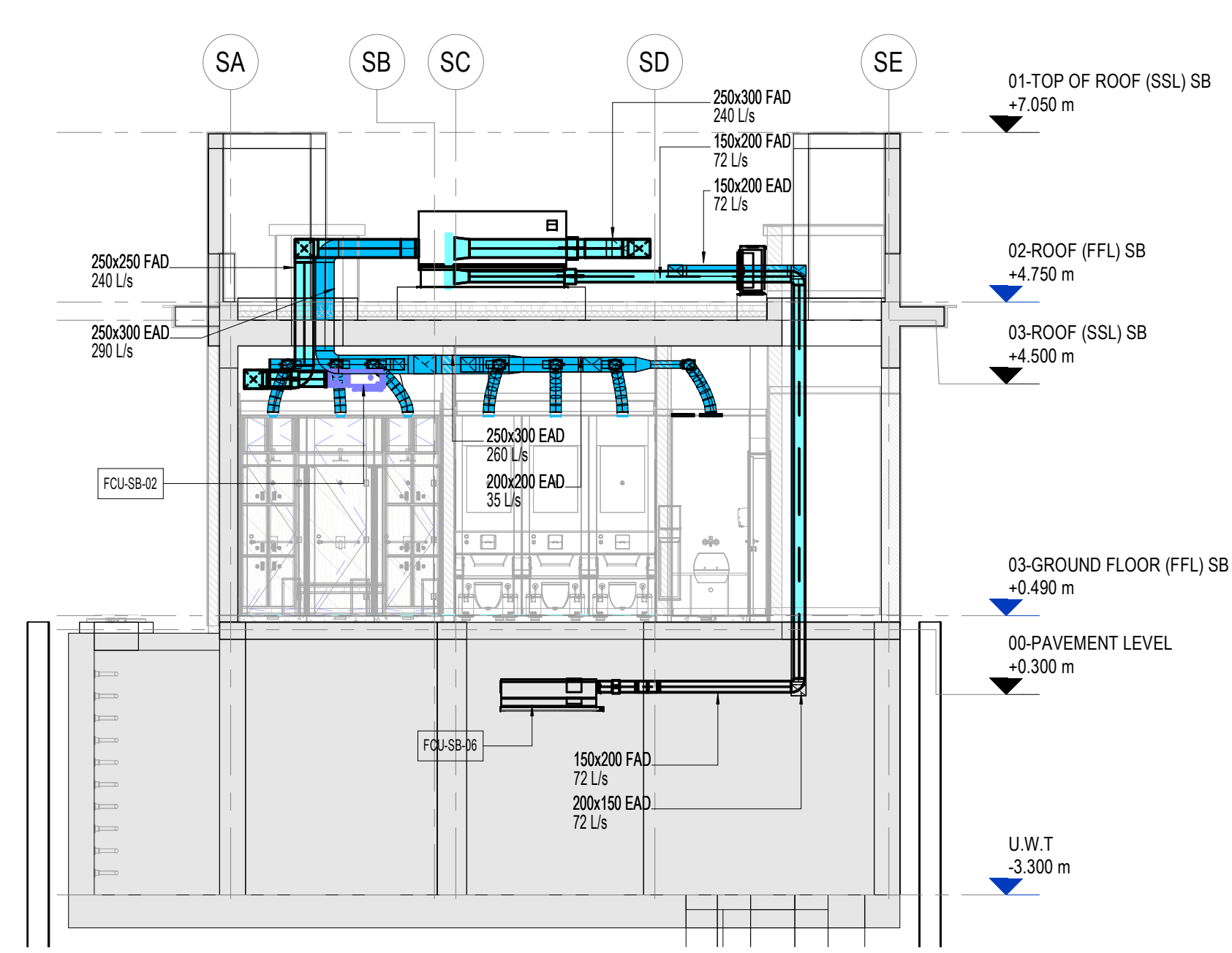
5 SERVICE BLOCK VENTILATION SECTION 02 1 : 75
