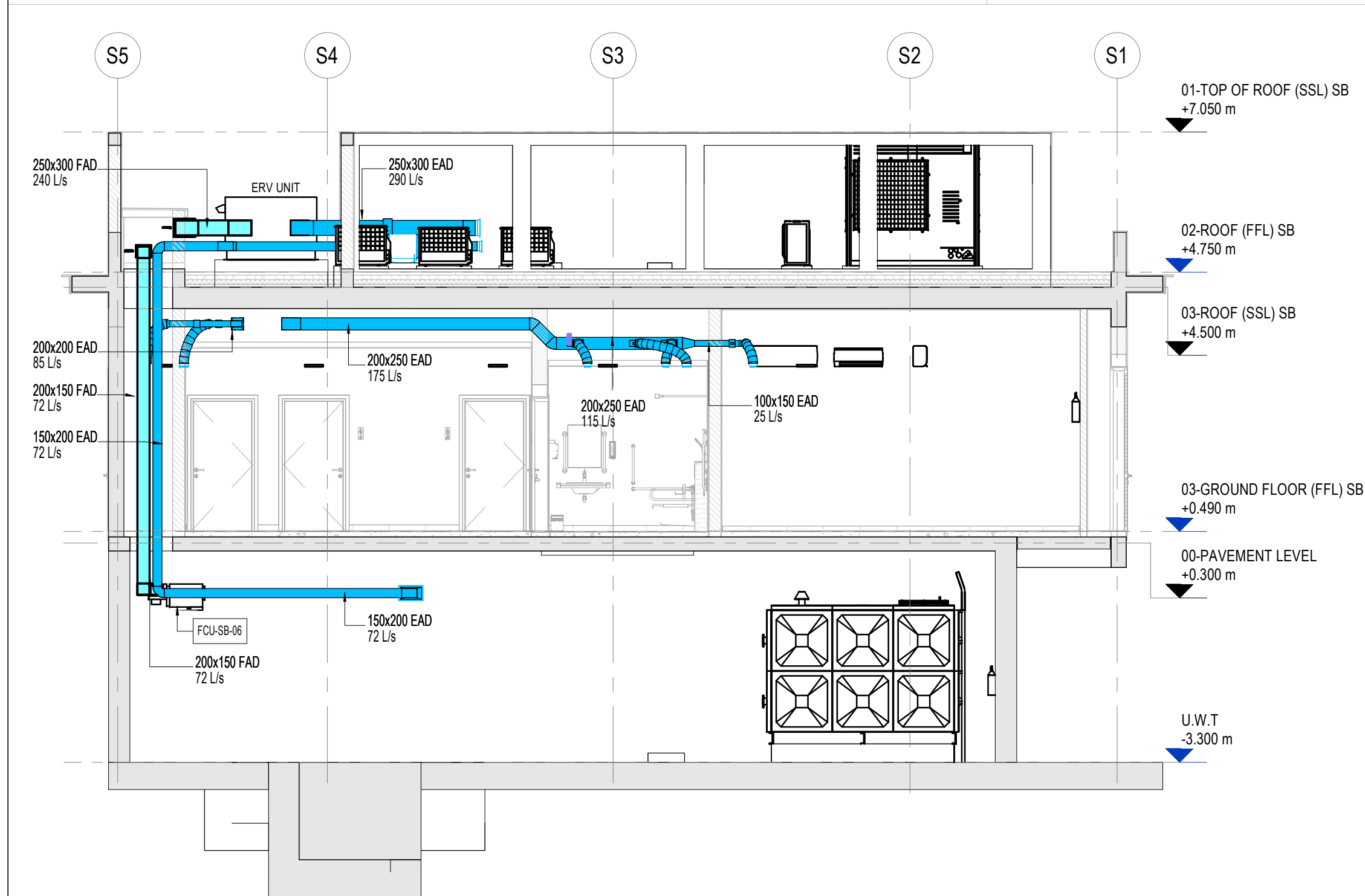
4 SERVICE BLOCK VENTILATION SECTION 01 1 : 75
