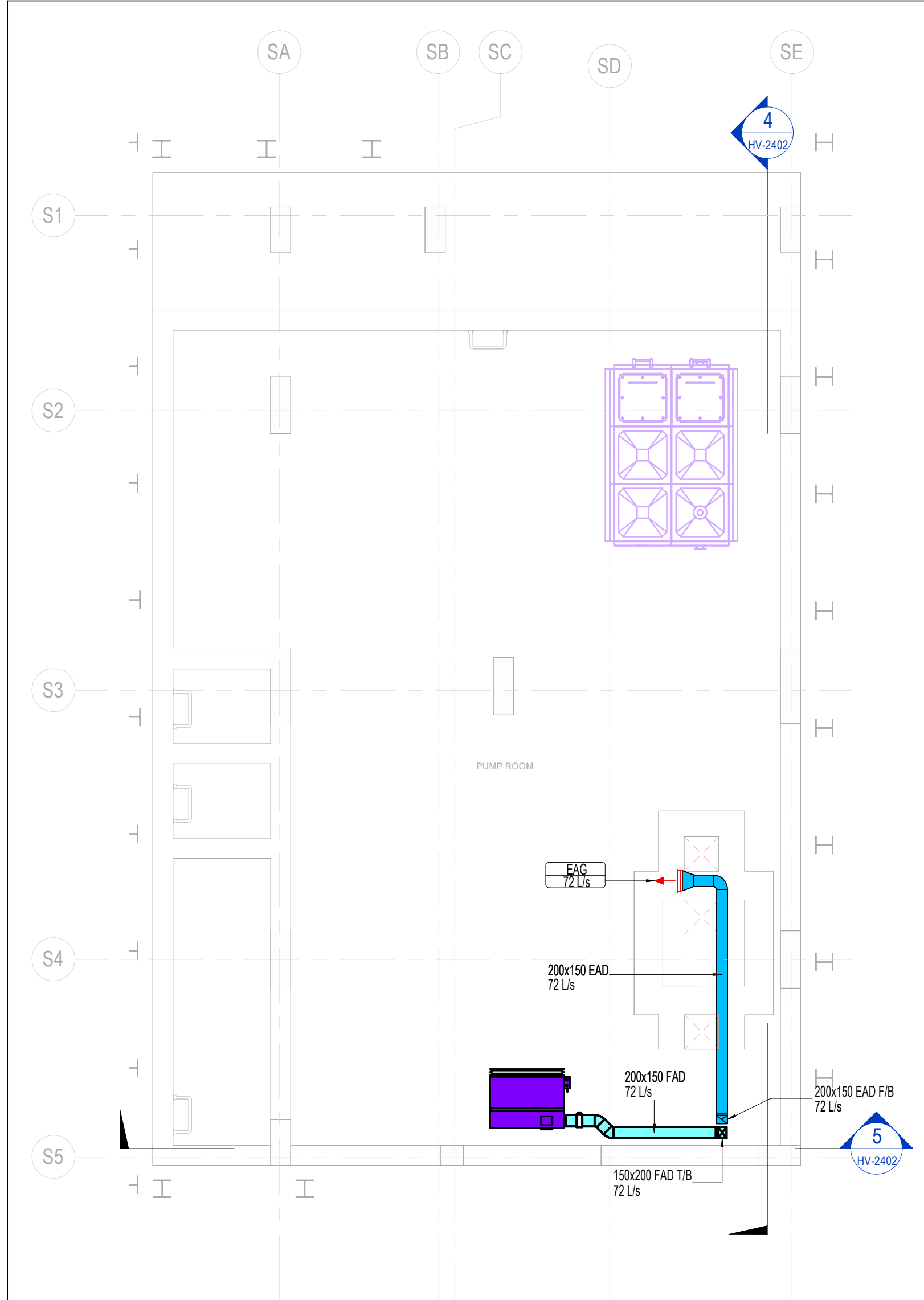
1 BASEMENT FLOOR VENTILATION LAYOUT 1 : 75
