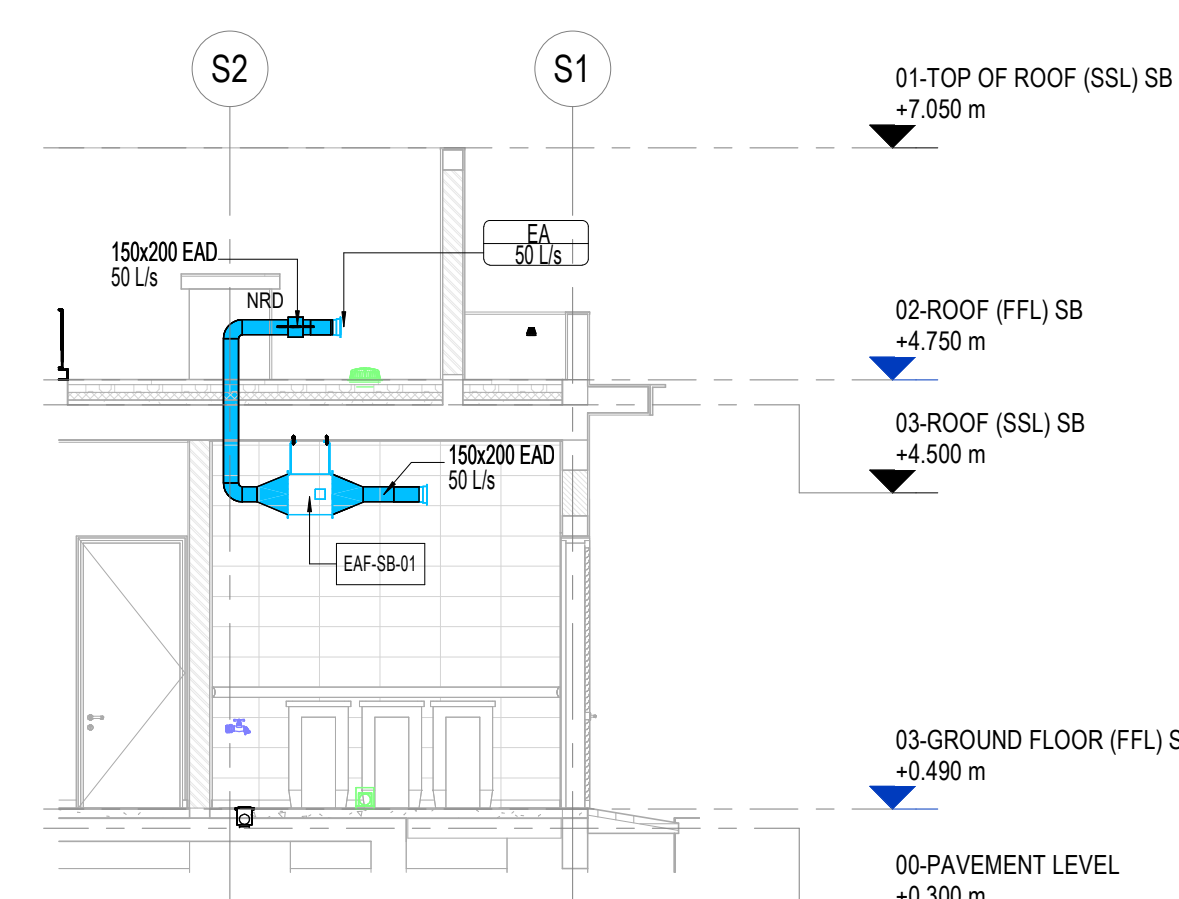
6 SERVICE BLOCK VENTILATION SECTION 03 1 : 75
