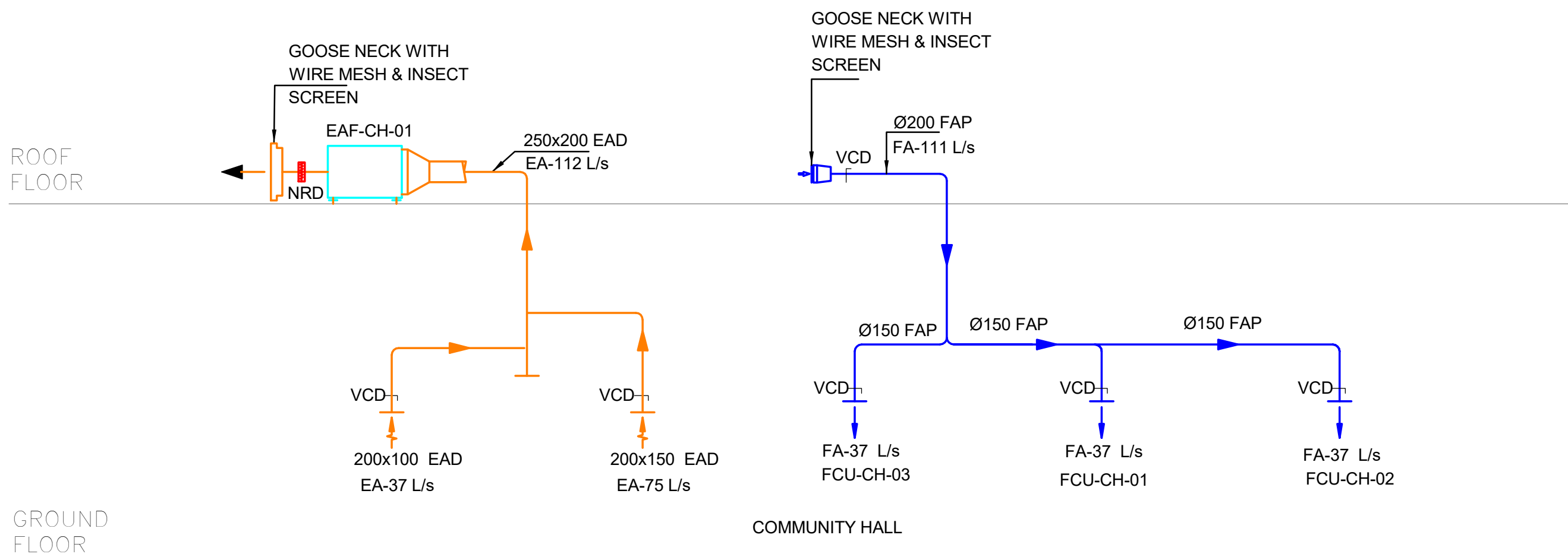
VENTILATION SCHEMATIC RISER DIAGRAM FOR COMMUNITY HALL
