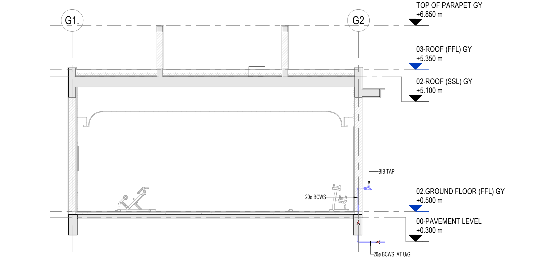
3 GYM&YOGA WATER SUPPLY SECTION 02 1 : 75
