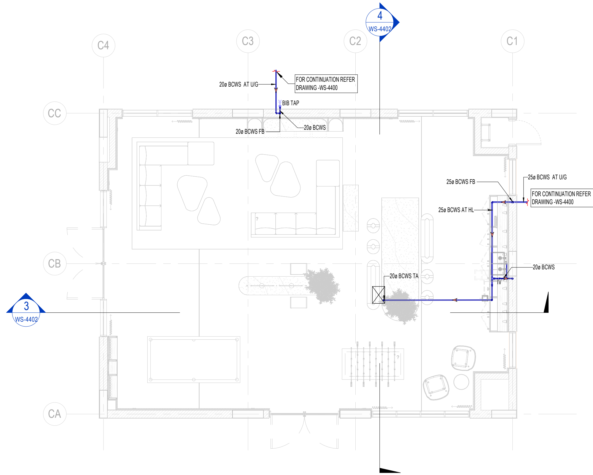
GROUND FLOOR WATER SUPPLY LAYOUT-COMMUNITY HALL
