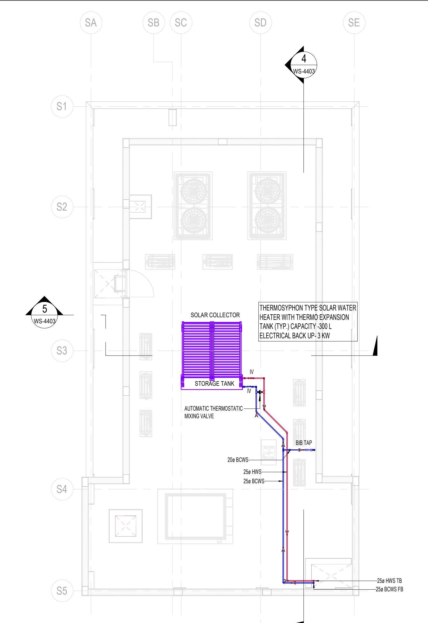
3 ROOF FLOOR WATER SUPPLY LAYOUT 1 : 75
