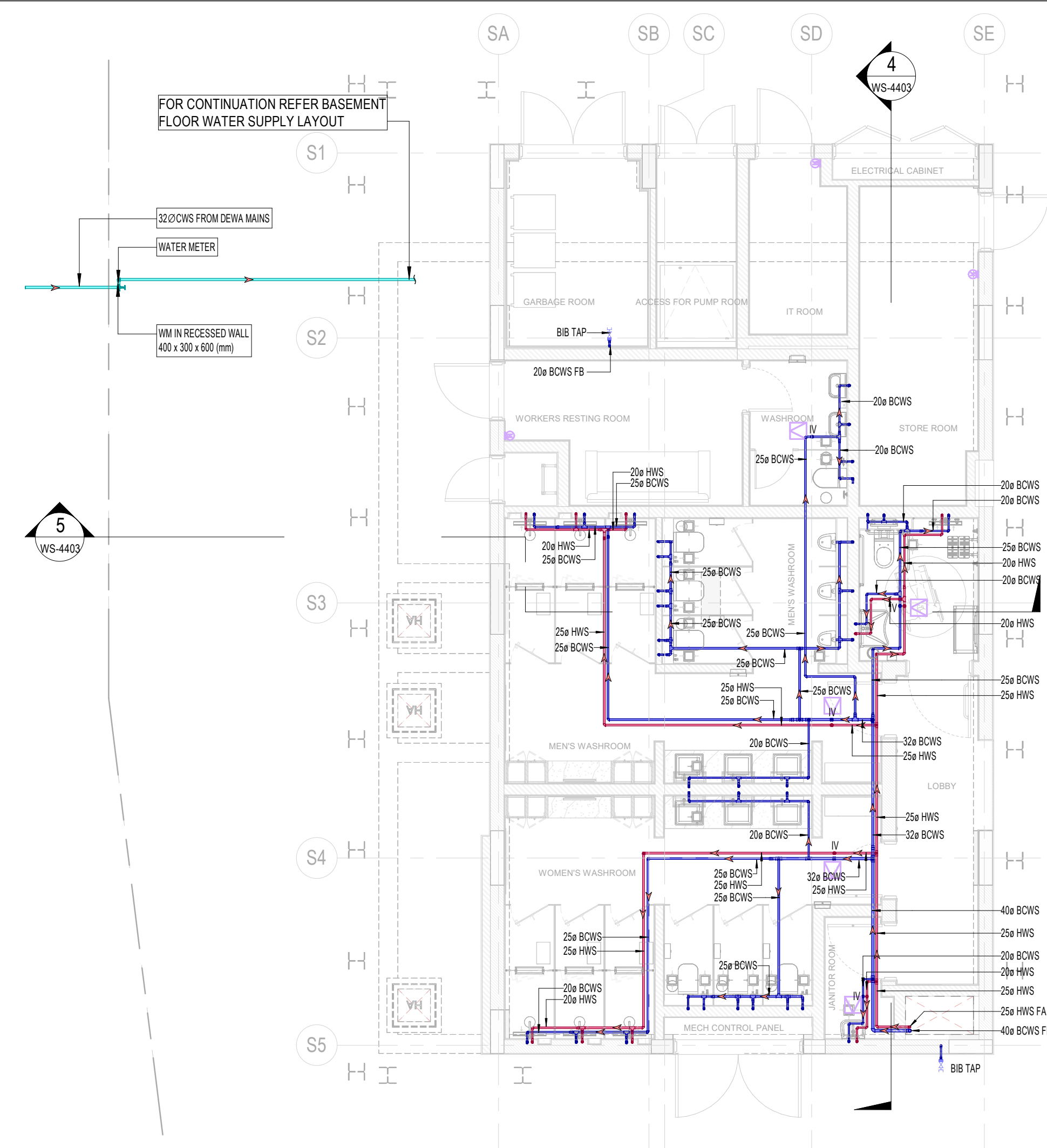
2 GROUND FLOOR_ WATER SUPPLY LAYOUT 1 : 75
