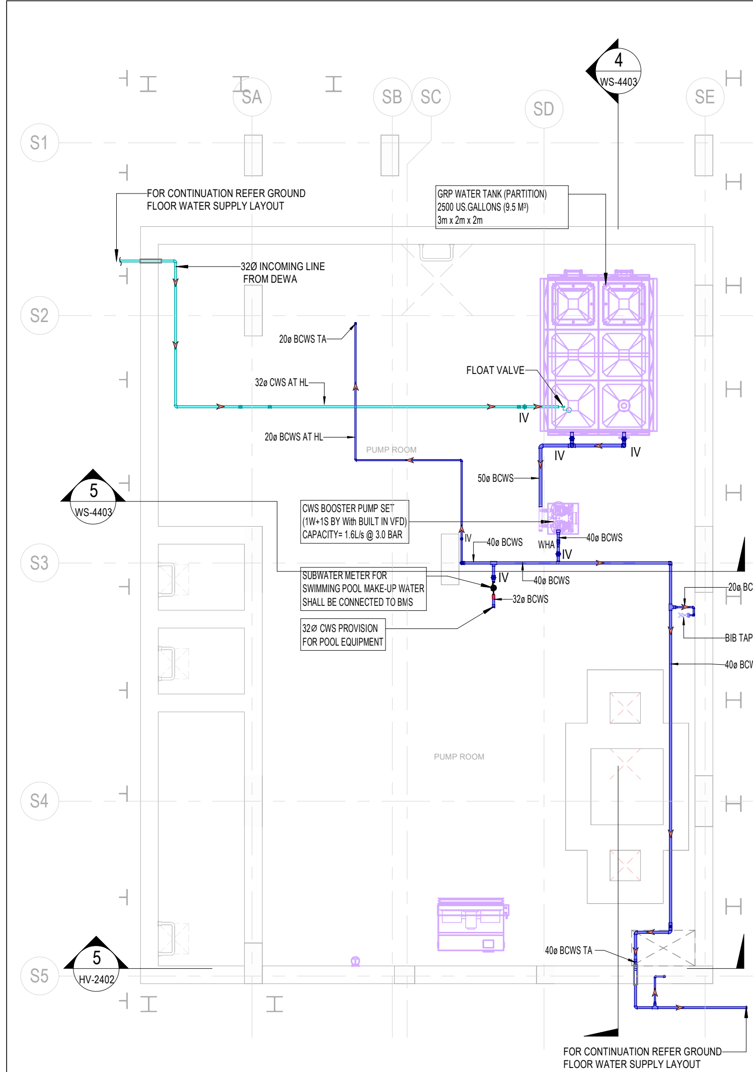
1 BASEMENT FLOOR WATER SUPPLY LAYOUT 1 : 75
