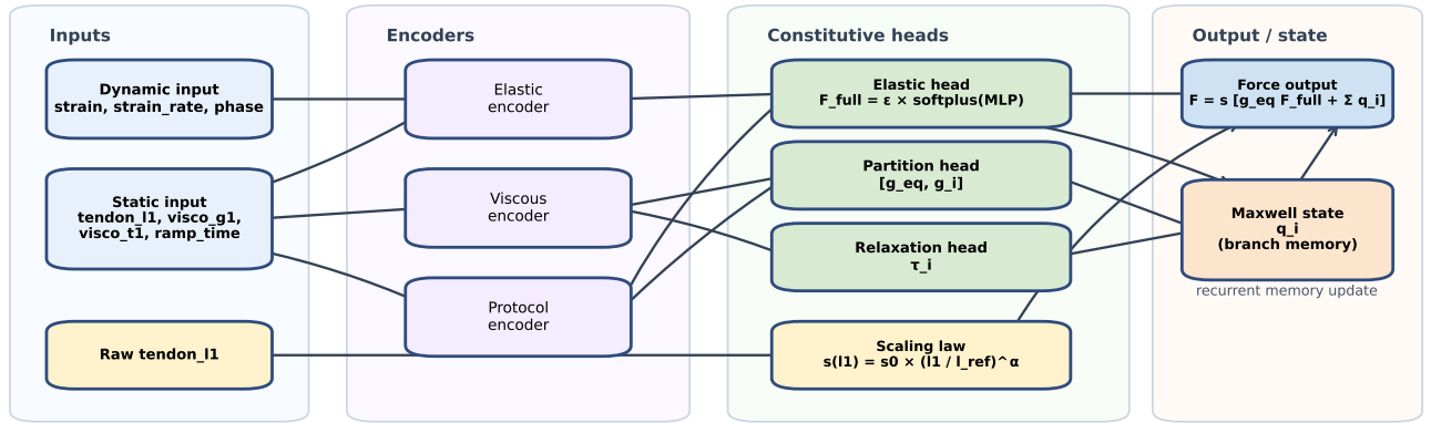
Figure 2: Architecture of the final physics-aware model. Small neural subnetworks encode static parameter groups and estimate elastic/viscous quantities, while explicit Maxwell branch states carry the viscoelastic memory over time.
