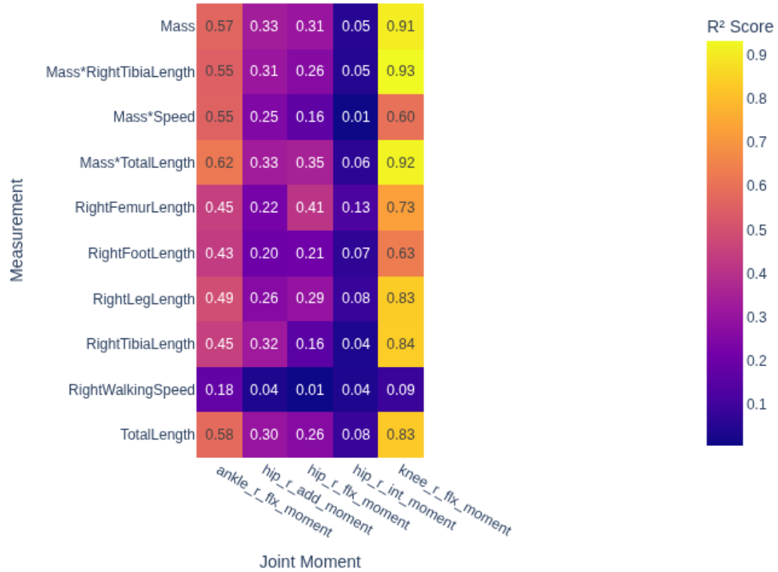
Figure 3.2: R 2 values for power fits of joint moment magnitudes to candidate normalization measurements. Higher values (yellow) indicate better fit.
