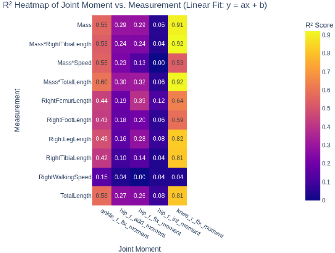
Figure 3.1: R^2 values for linear fits of joint moment magnitudes to candidate normalization measurements. Higher values (yellow) indicate better fit.
