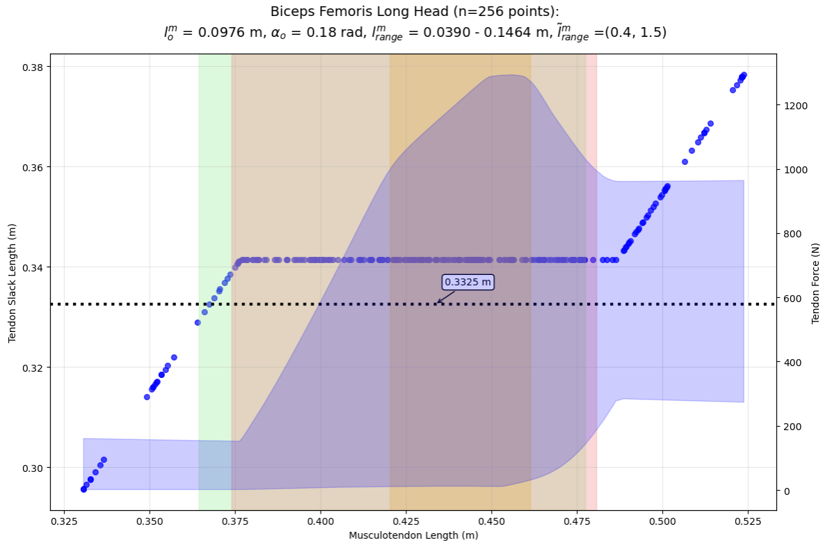
Figure 5.2: SSDP tendon slack length estimates and tendon force envelope for bfh across musculotendon lengths, with activity-specific length ranges overlaid.
