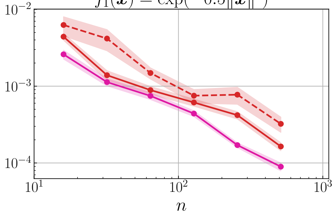
Cubature Error
