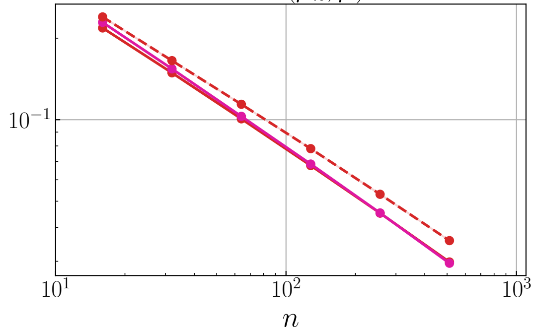
MMD
