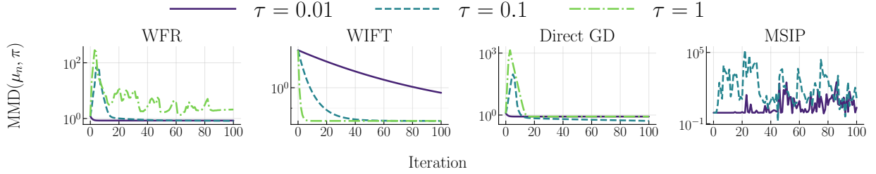
Figure 2: Distant initialization on [8, 10]. MMD trajectories for the particle update schemes.
