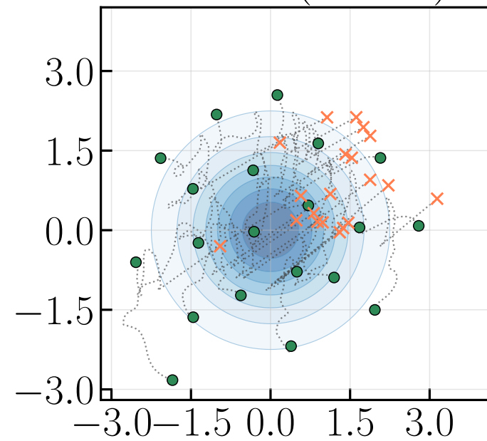
WIFT ( \tau = 1 )
