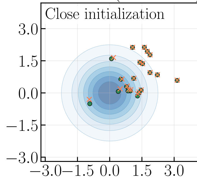
Euc-PD ( \tau = 0.01 )
