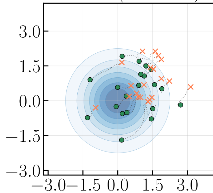
WFR ( \tau = 0.1 )
