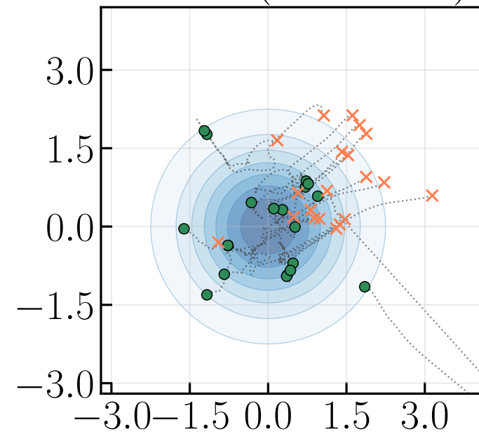
MSIP ( \tau = 0.01 )
