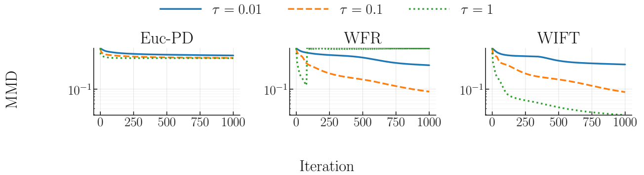
Figure 2: Mean-field ReLU student-teacher network with d = 5 , N = 40 , and M = 20 . MMD trajectories for Euc-PD, WFR, and WIFT over 1000 iterations and L = 256 fixed inputs, with \tau \in \{0.01, 0.1, 1\} . All panels use the y-axis range of the WIFT trajectories.
