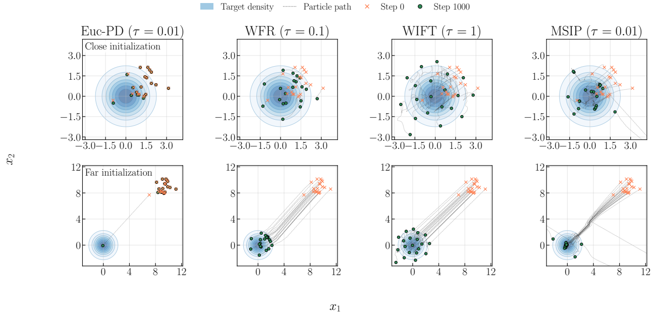
Figure 3: Particle trajectories under close and far initialization. Paths of all 20 particles from step 0 to step 1000 for initial distributions \mathcal{N}((1, 1), I_2) and \mathcal{N}((9, 9), I_2) , respectively.
