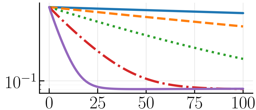
WIFT
