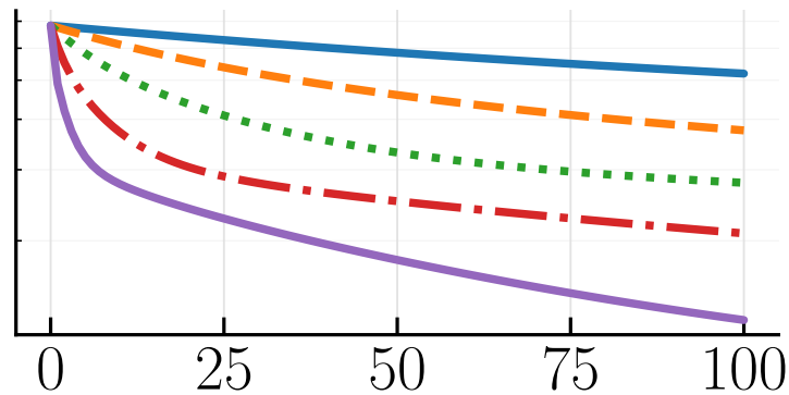
Euc-PD
