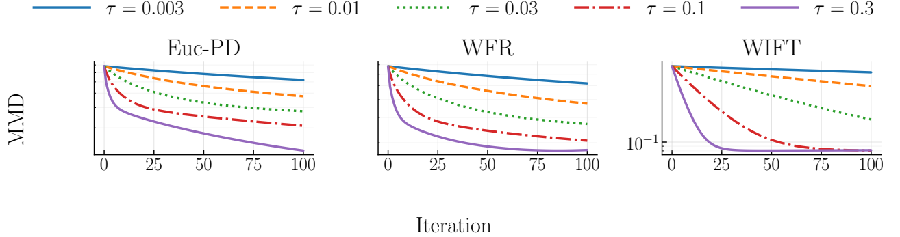
Figure 2: Mean-field ReLU student-teacher network with d = 5 , N = 40 , and M = 20 . MMD trajectories for Euc-PD, WFR, and WIFT over 100 iterations and L = 256 fixed inputs.
