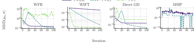
Figure 1: An empirical plot for the various particle update schemes.
