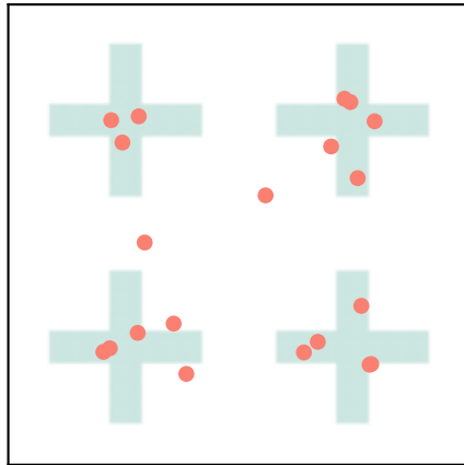
MMD Flow ( T=20 )
