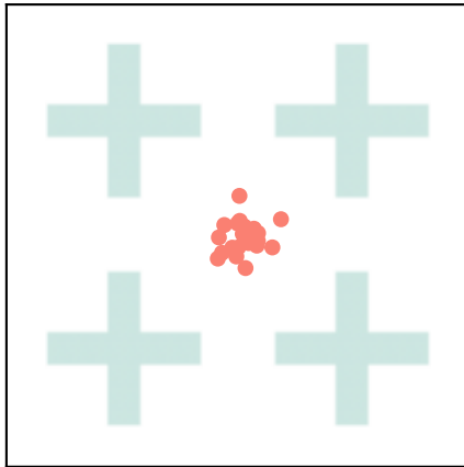
MMD Flow ( T=0 )
