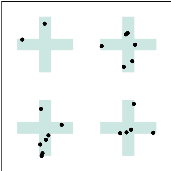
IID
