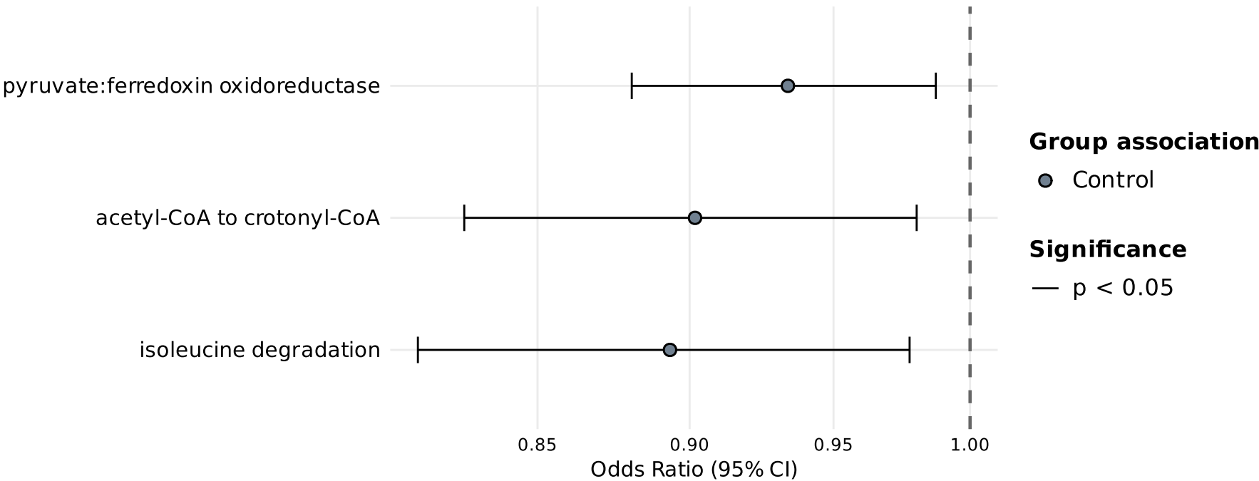
C) Logistic regression: high prevalence modules (>85%) (p < 0.05) at TP2
