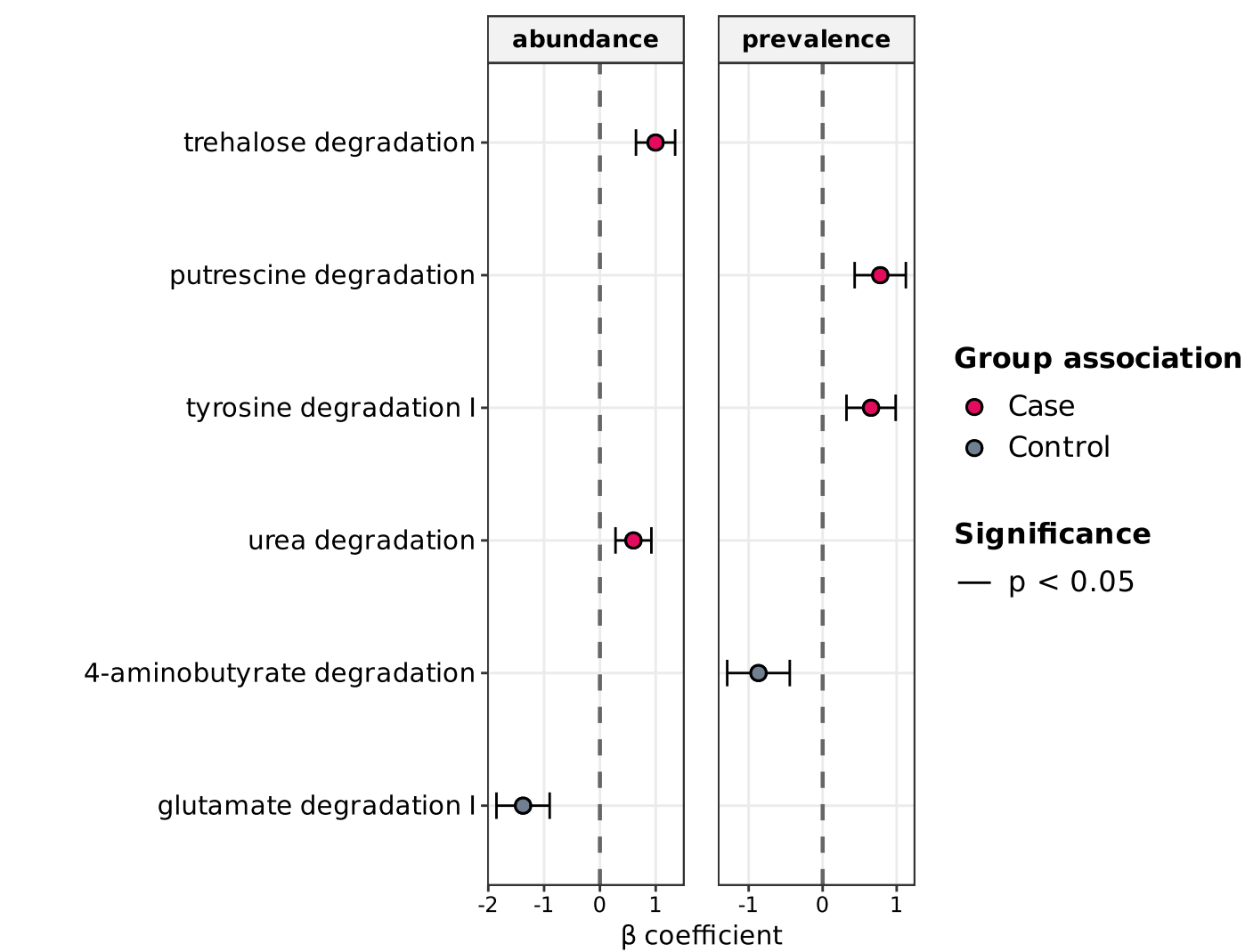
A) MaAsLin3: significant GMM associations (p < 0.05) at TP2
