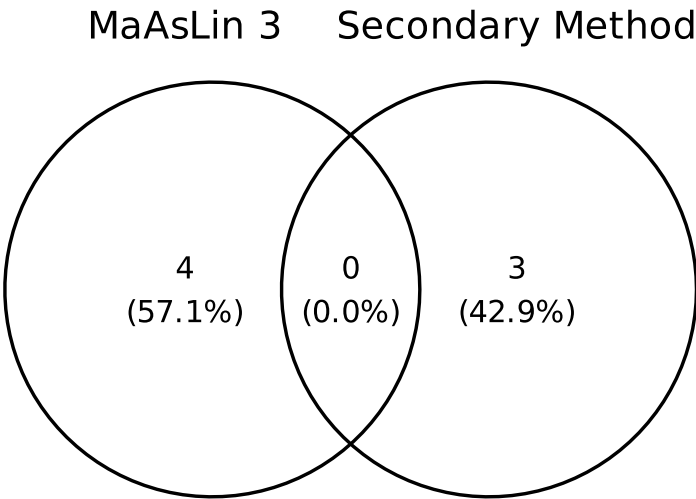
D) Convergent GMM findings (p < 0.05) at TP2
