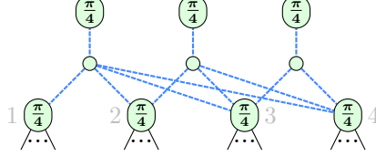
Figure 3.4: Diagram where the heuristic (3.21) underestimates the effective heuristic value
