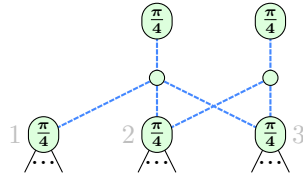
Figure 3.3: Diagram where the heuristic (3.17) is not valid
